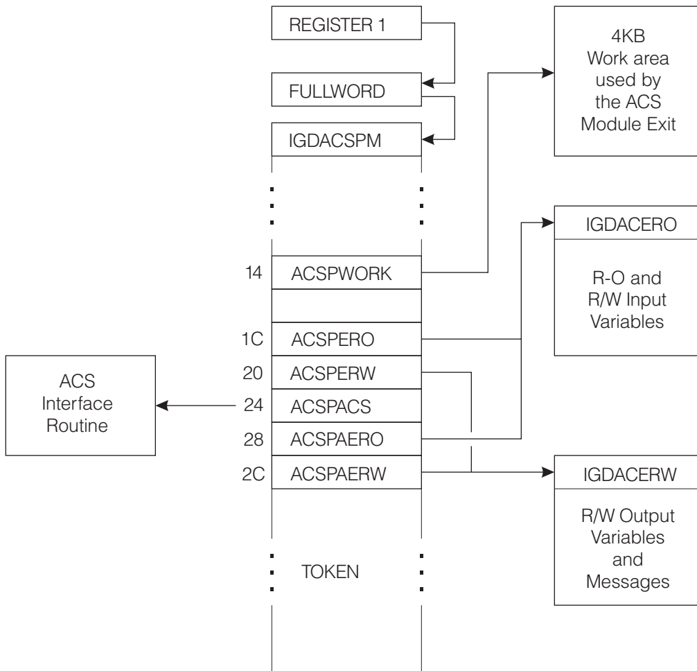
Figure 105. Parameter Structure for the ACS Module Exit. This figure shows the control-block structure upon entry into the exit.
