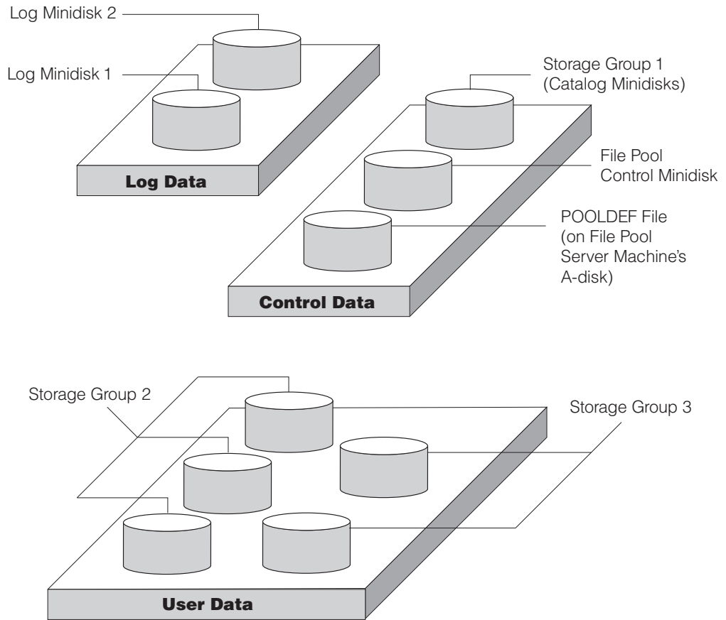
Figure 3. SFS File Pool Structure
