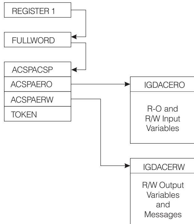
Figure 112. Parameter Structure for the ACS Interface Routine. This figure shows the control-block structure for invoking the ACS interface routine from the module exit routine.
