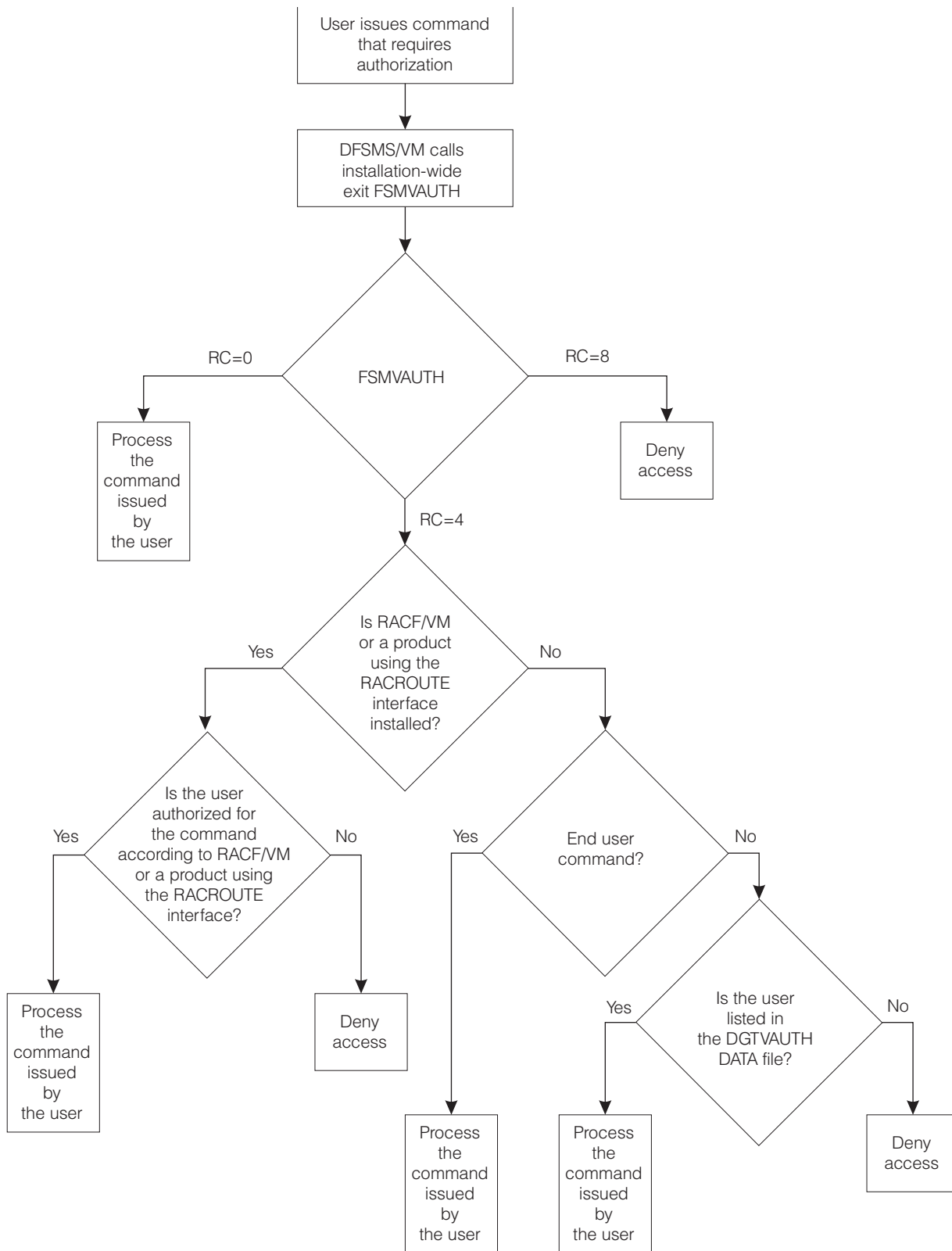
Figure 65. The DFSMS Command Authorization Process
