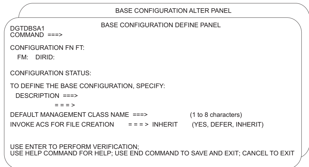
Figure 31. Base Configuration Define or Alter Panels
