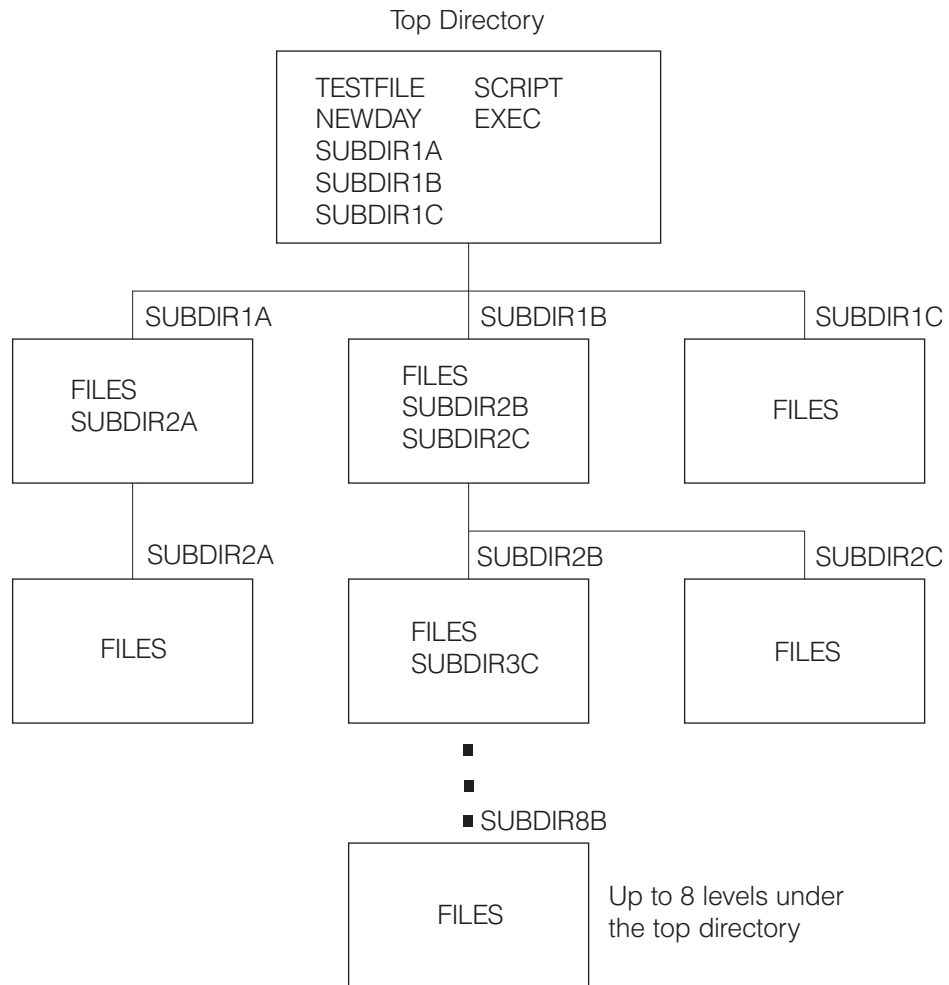
Figure 4. SFS Directory Structure
