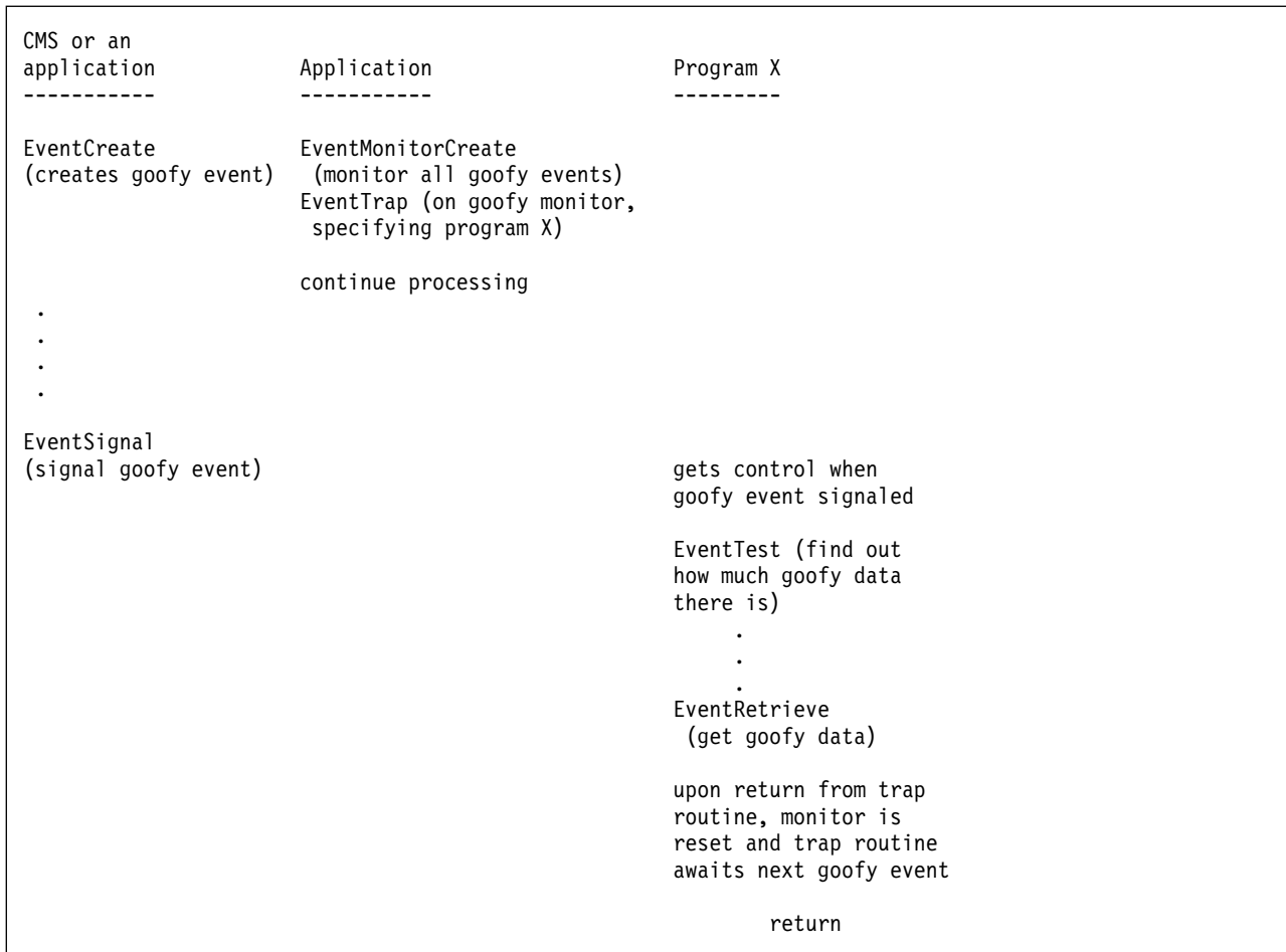
Figure 5. EventTrap Example
