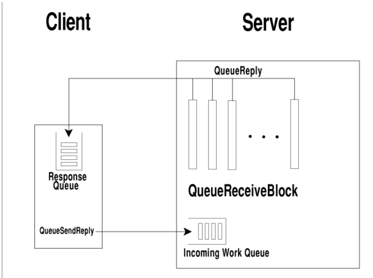
Figure 2. Queue-Based Structure
