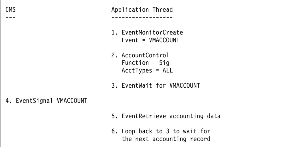
Figure 28. Requesting and Collecting Accounting Data
