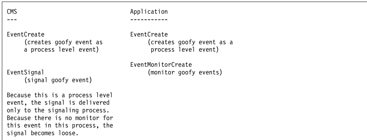
Figure 10. Process Level Events Example
