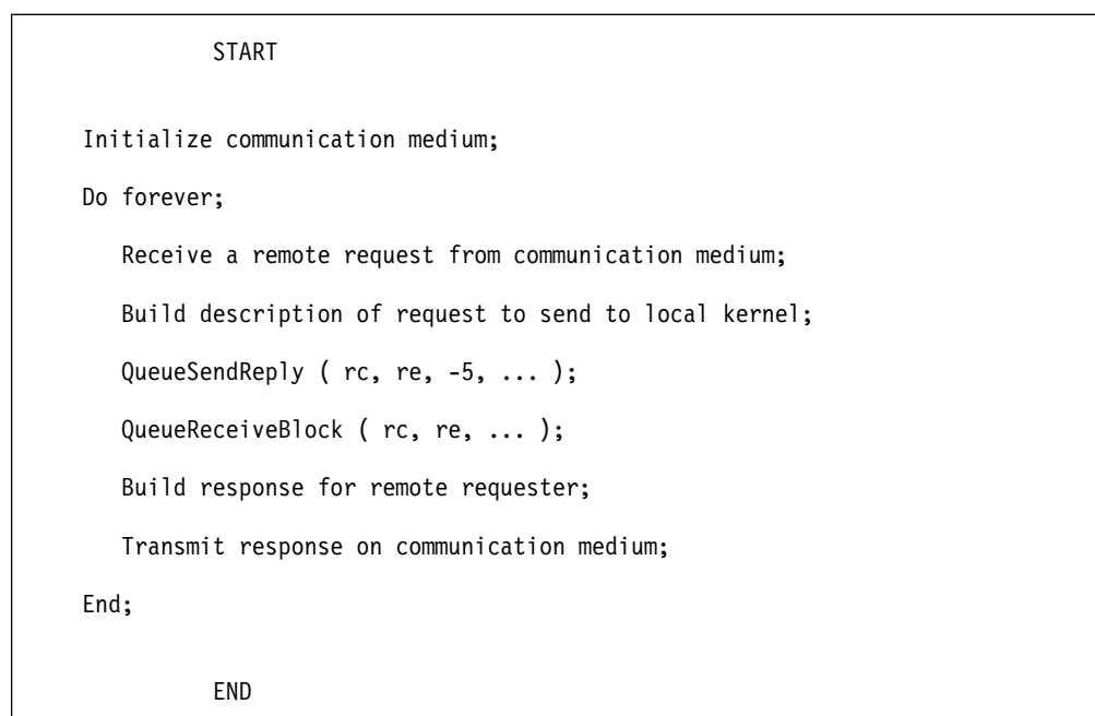
Figure 32. Skeleton of an IPC Carrier (Carrier-Initiated Requests)
