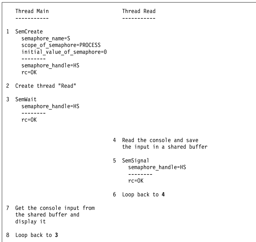
Figure 21. Wait/Post Processing Using a Semaphore
