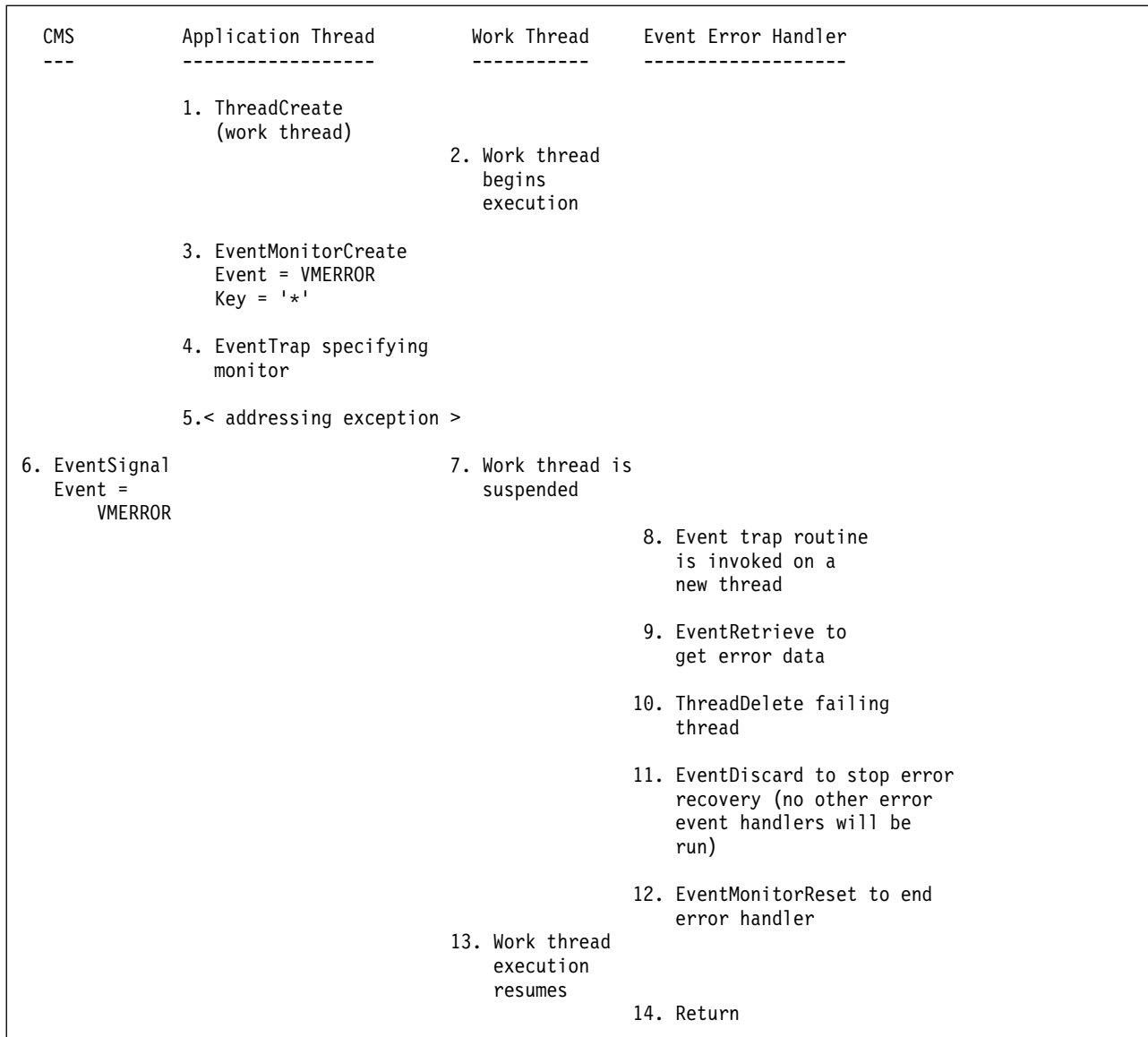
Figure 30. Event Trap Deleting Failing Thread
