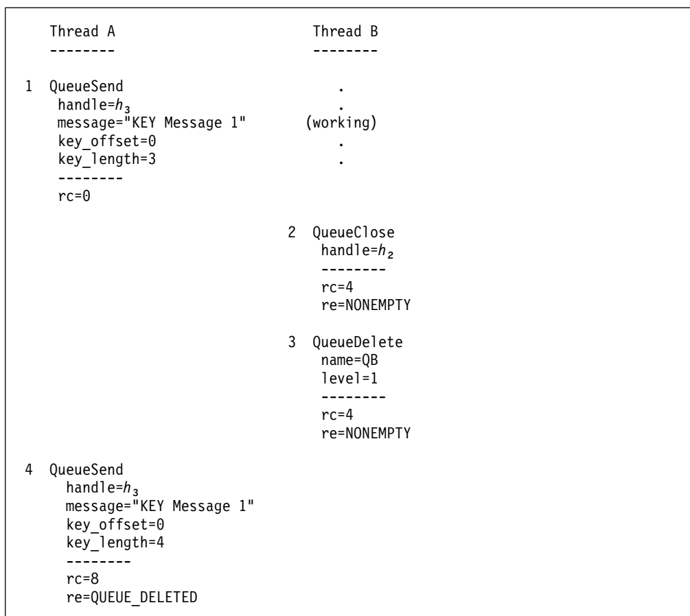
Figure 19. Closing and Deleting Queues
