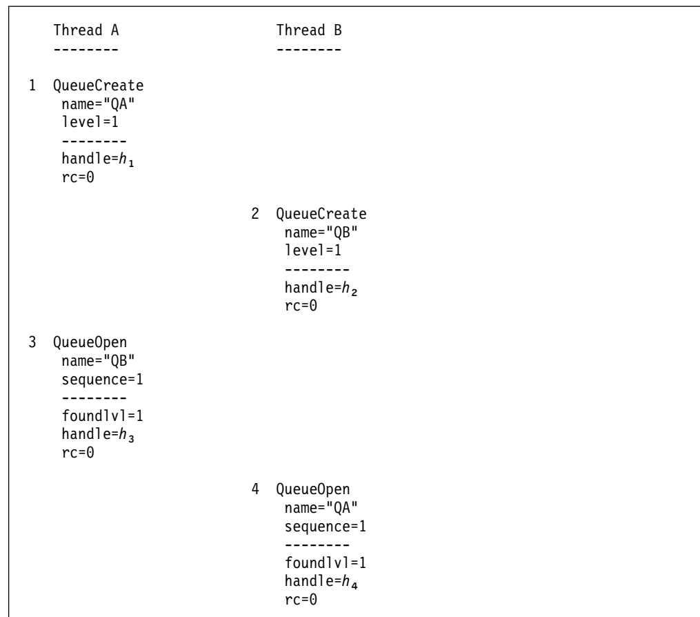
Figure 12. Creating and Opening Queues
