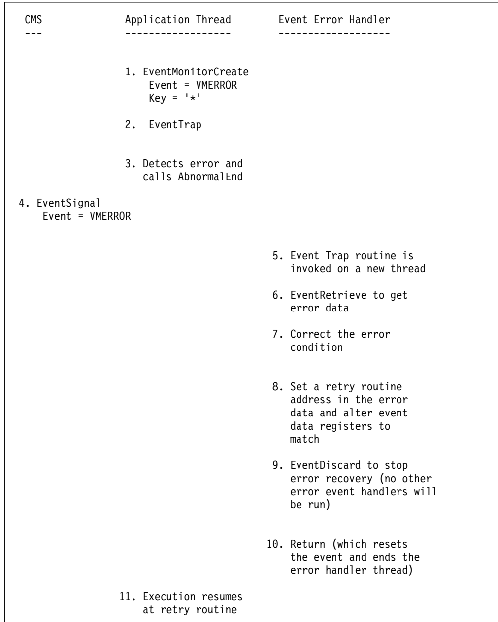
Figure 29. AbnormalEnd with Error Recovery Specifying Retry Routine
