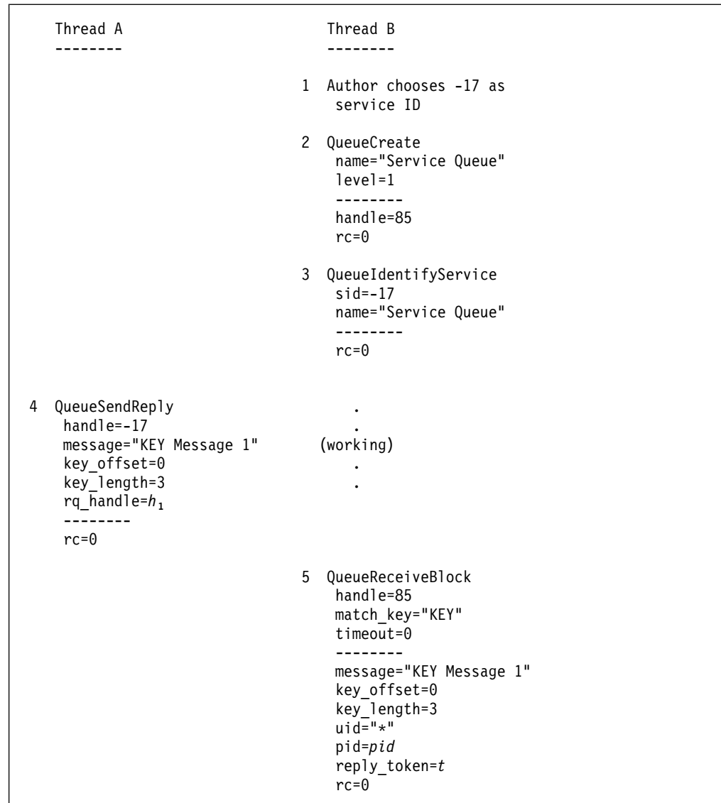
Figure 18. Using Service Queues
