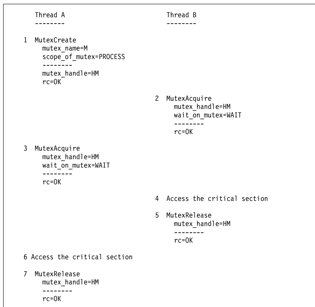
Figure 20. Accessing a Critical Section Protected by a Mutex
