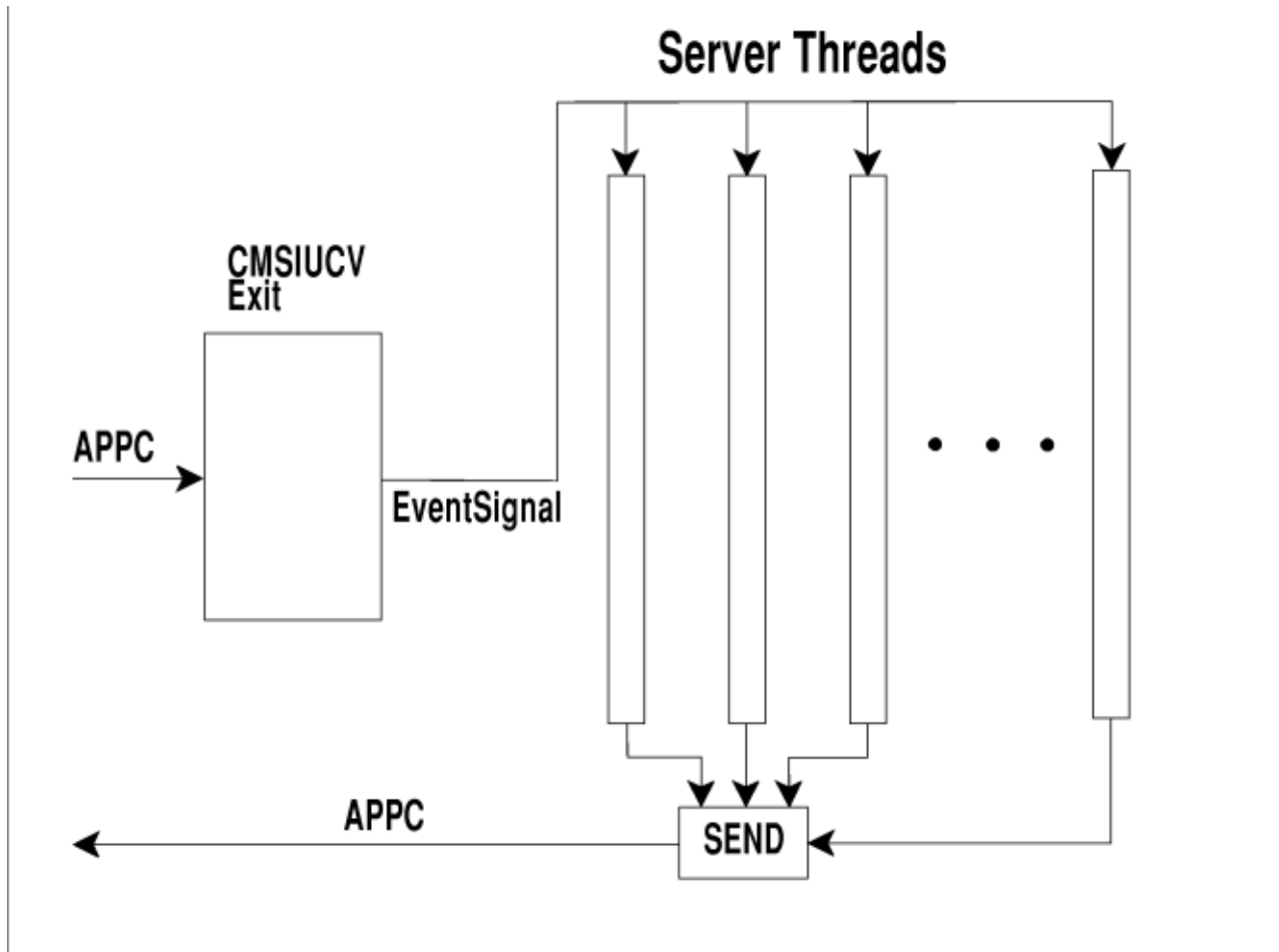
Figure 3. Event-Based Structure
