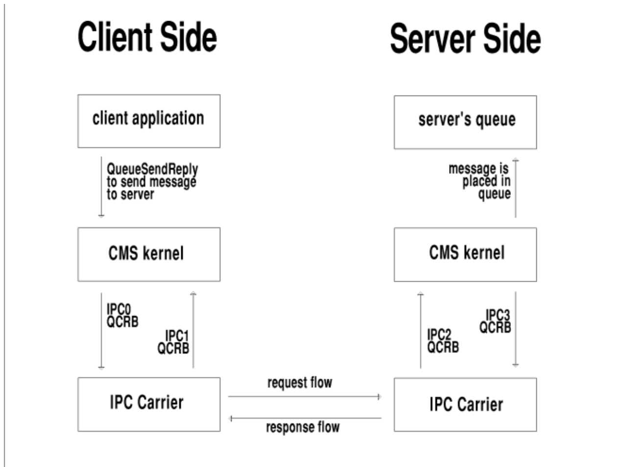
Figure 33. Flow of Requests and Responses for Distributed IPC
