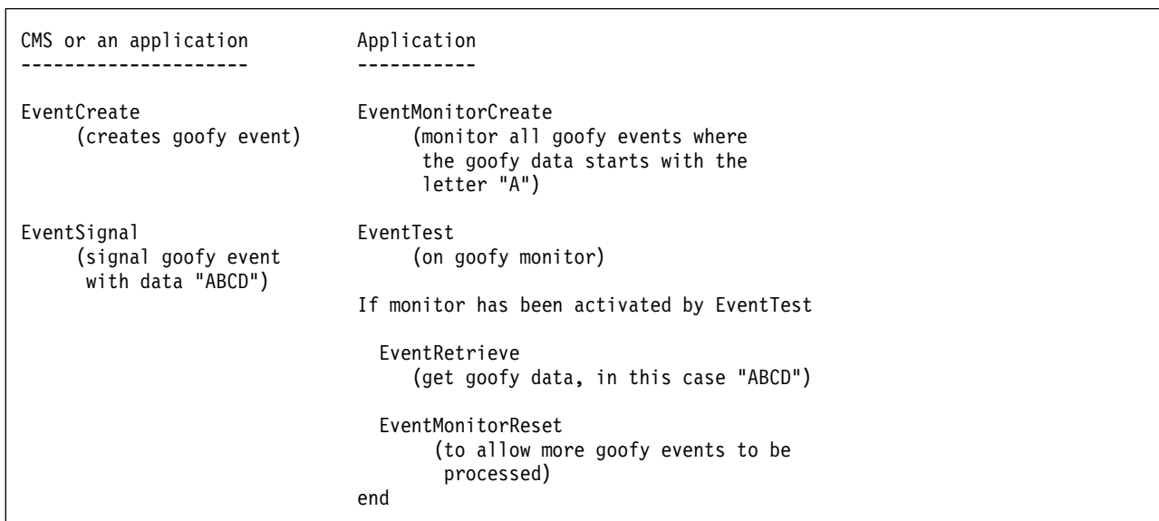
Figure 6. EventTest Example
