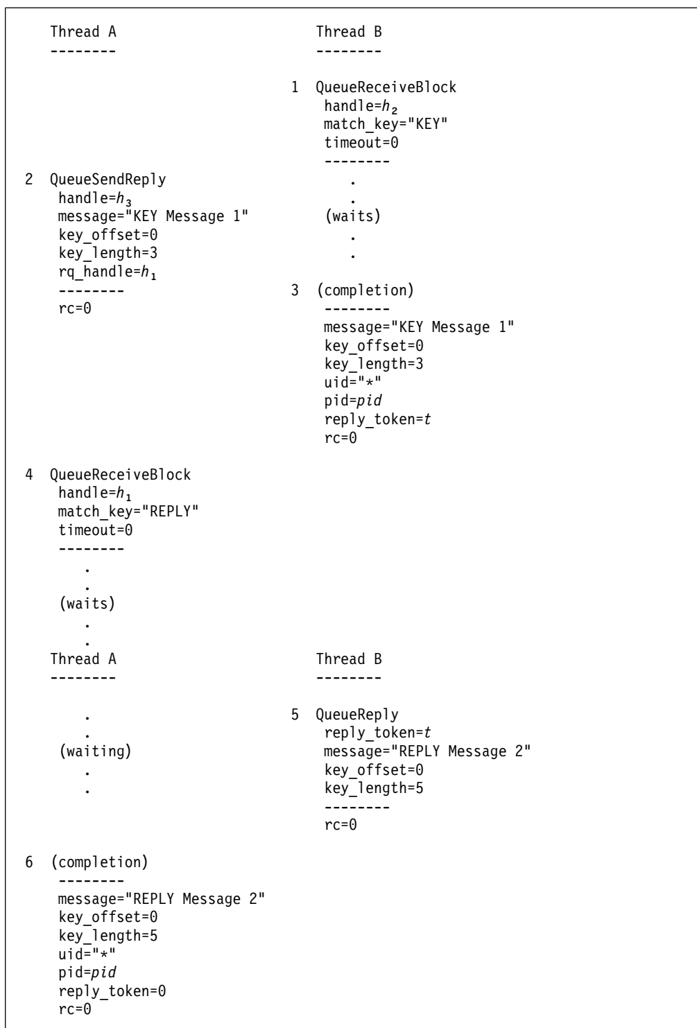
Figure 15. Using QueueReply
