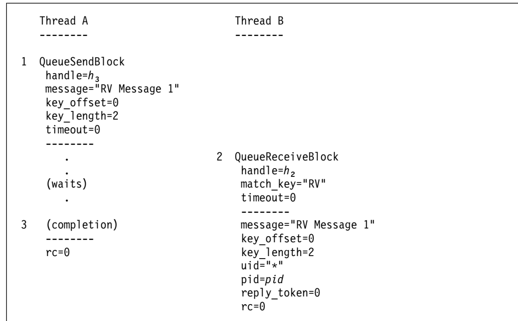
Figure 14. A Rendezvous
