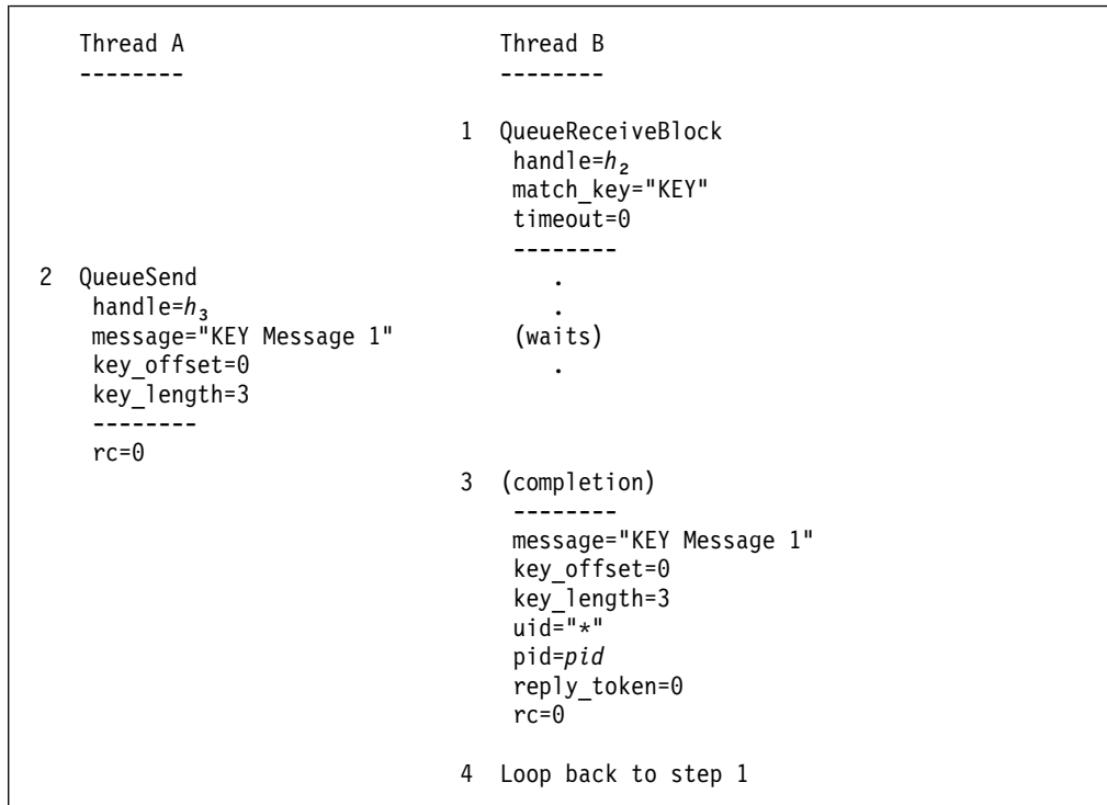
Figure 13. Simple Message Transmission
