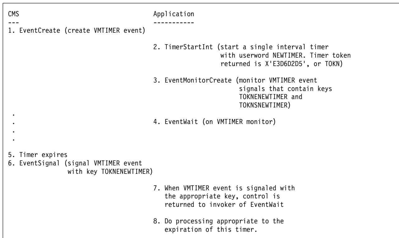
Figure 27. EventWait and Timer Services
