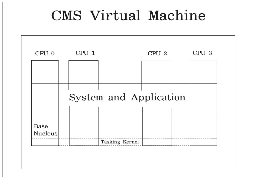
Figure 1. The CMS Multitasking, Multiprocessor Environment
