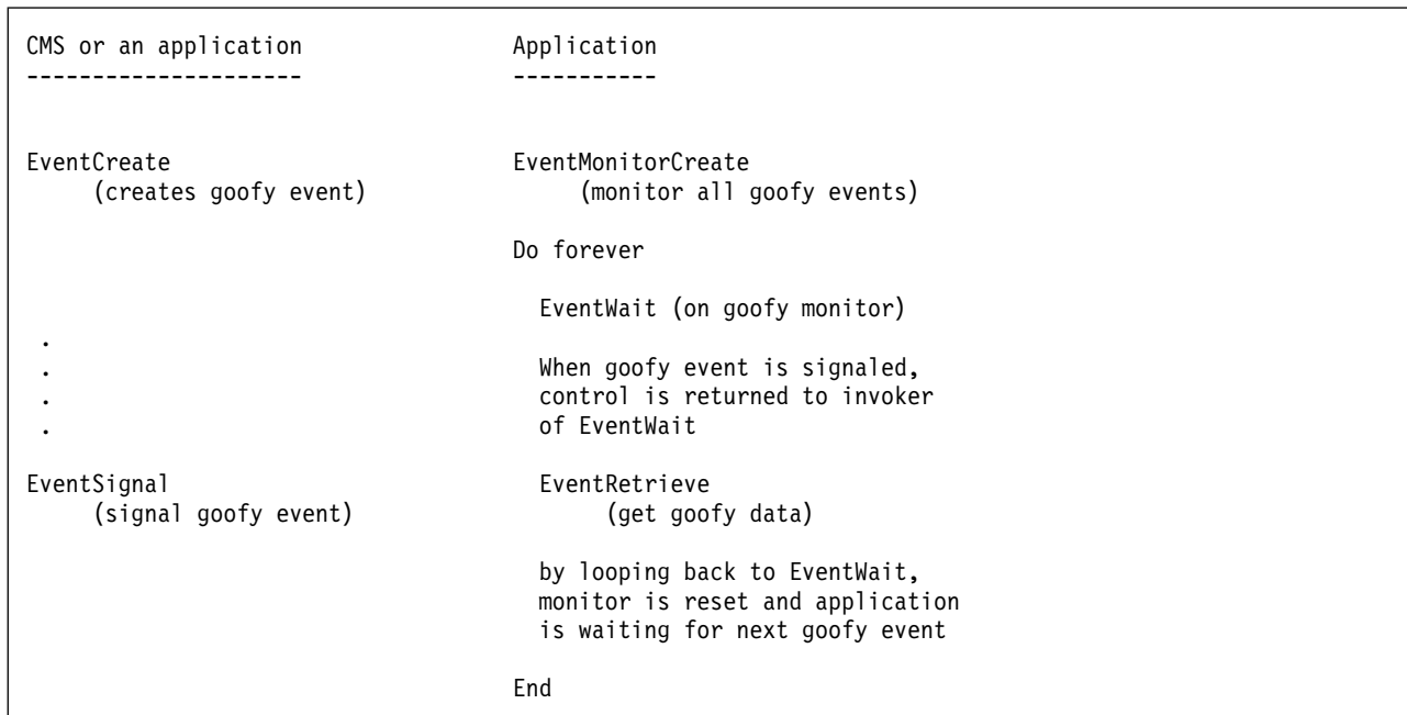
Figure 4. EventWait Example
