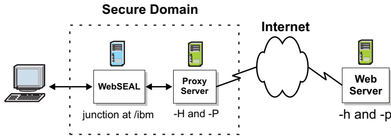
Figure 29. Example proxy junction
