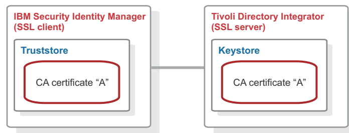
Figure 1. One-way SSL communication
