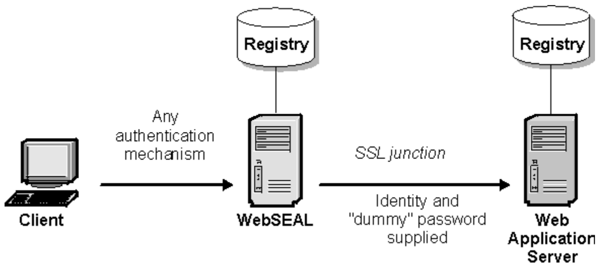
Figure 44. BA Header contains identity and dummy password
