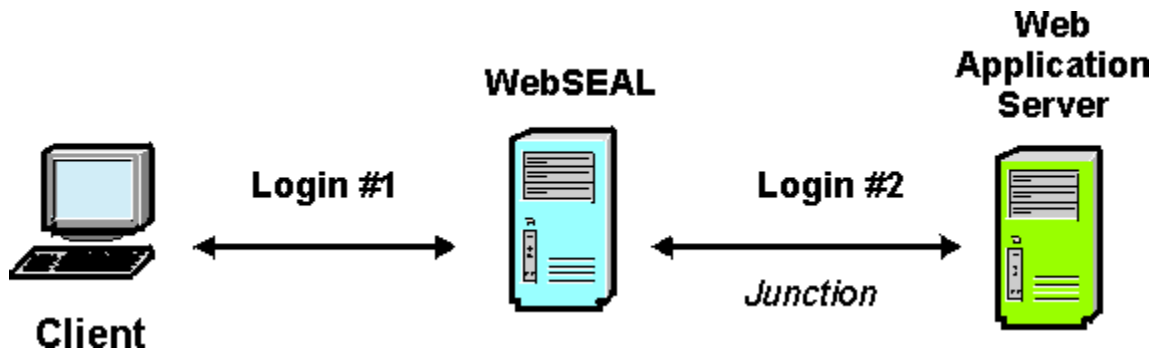
Figure 42. Multiple logins
