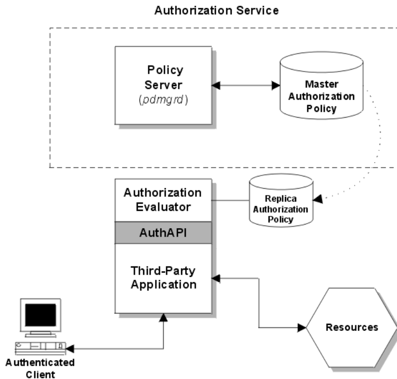
Figure 9. Authorization API: local cache mode
