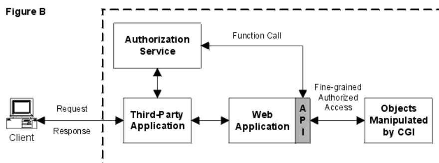
Figure 7. Example use of the authorization API
