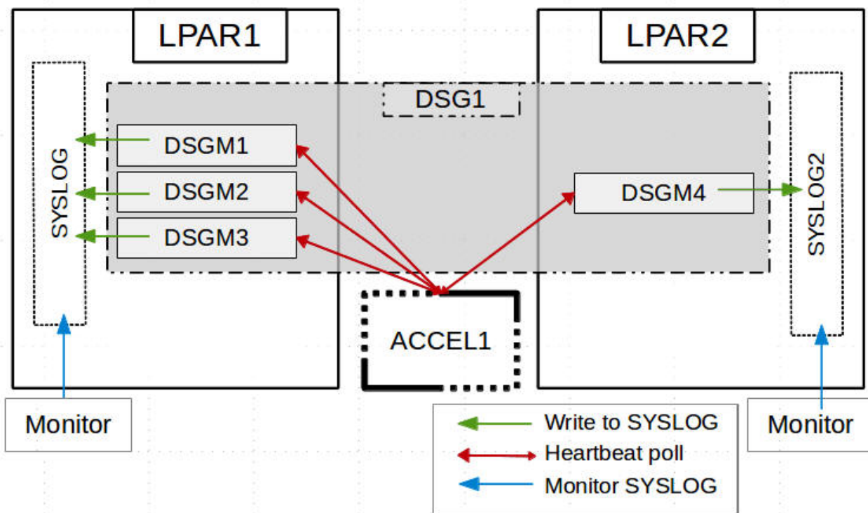
Figure 23. Members in two different LPARs
