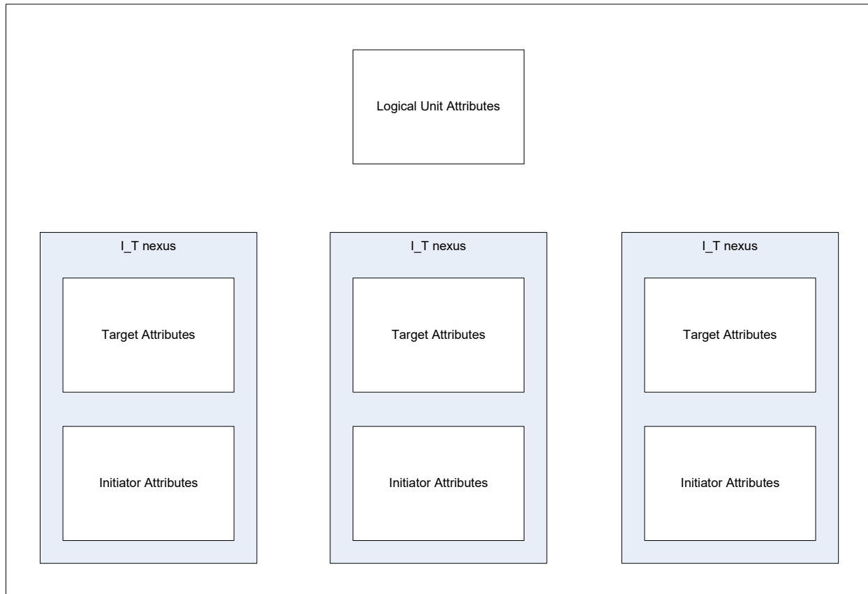
Figure 7 — Dynamic runtime attributes focus
