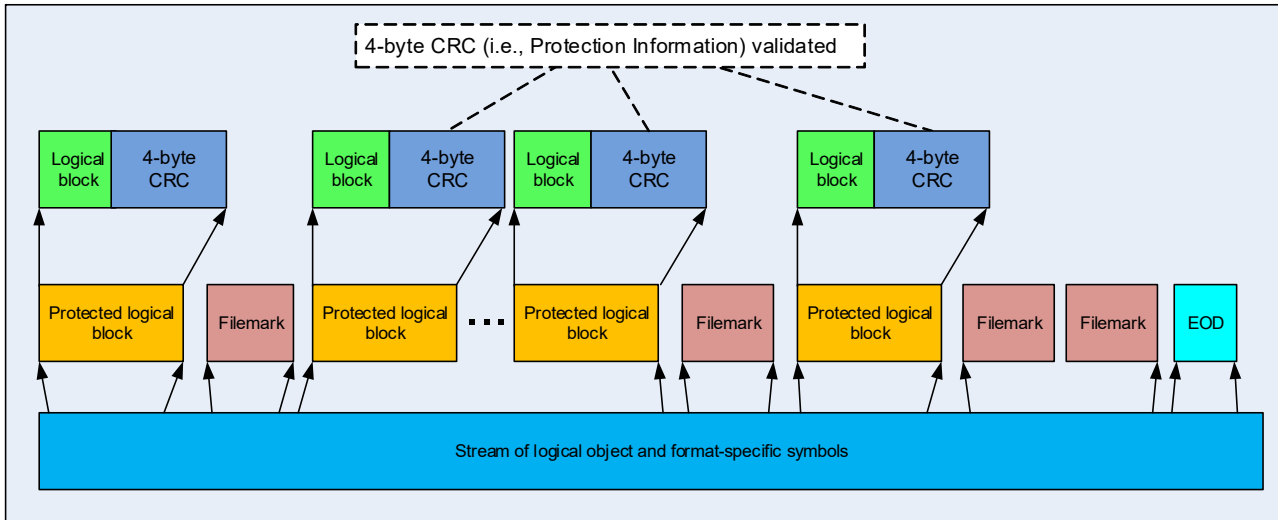
Figure 6 — Protection information shown in relation to logical objects and format specific symbols
