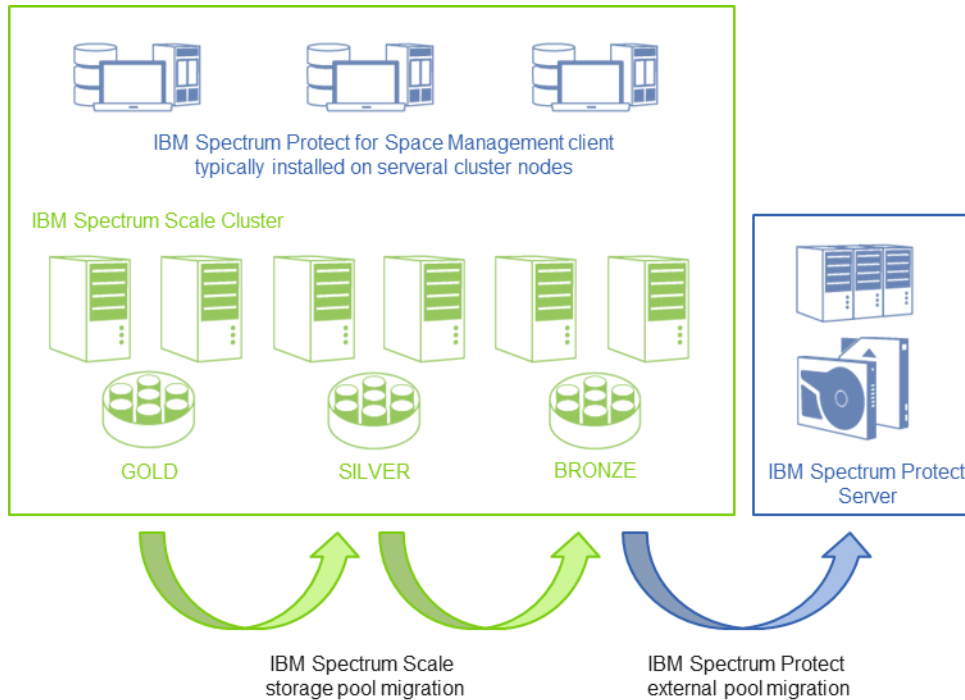
Figure 2. IBM Storage Protect for Space Management architecture
