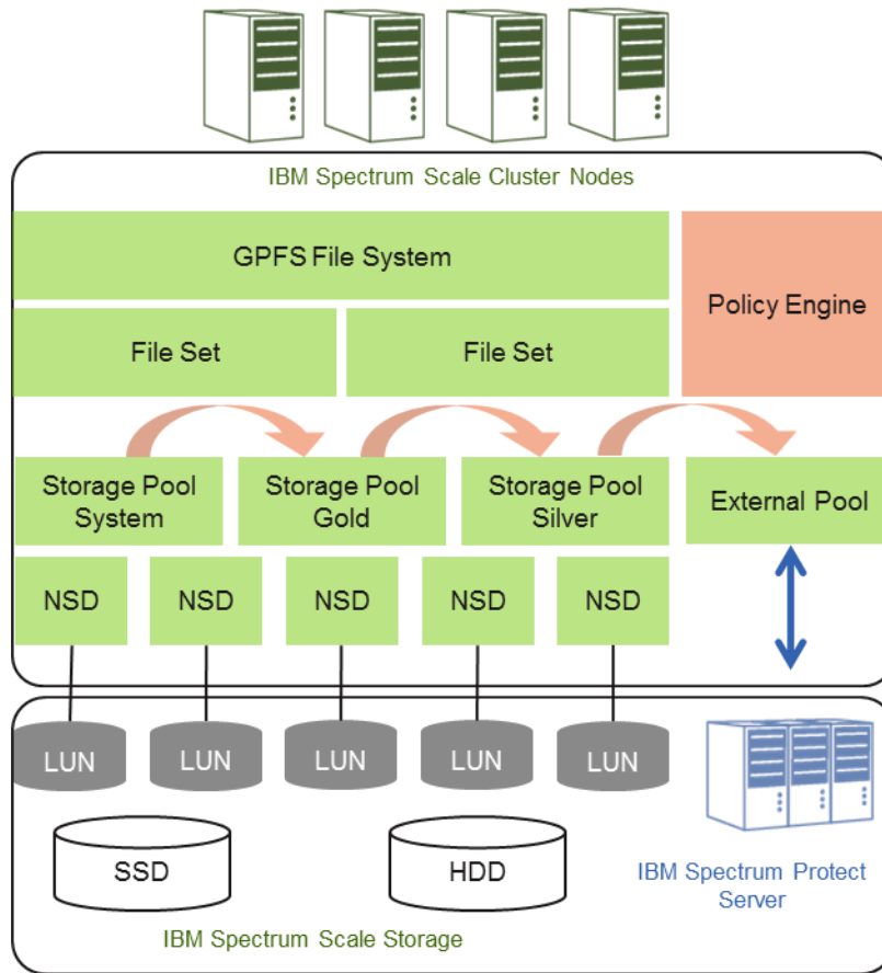
Figure 1. Basic concept of an IBM Storage Scale file system and pools
