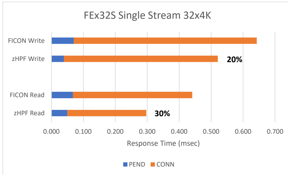
Figure 7 – FEx32S Response Time
