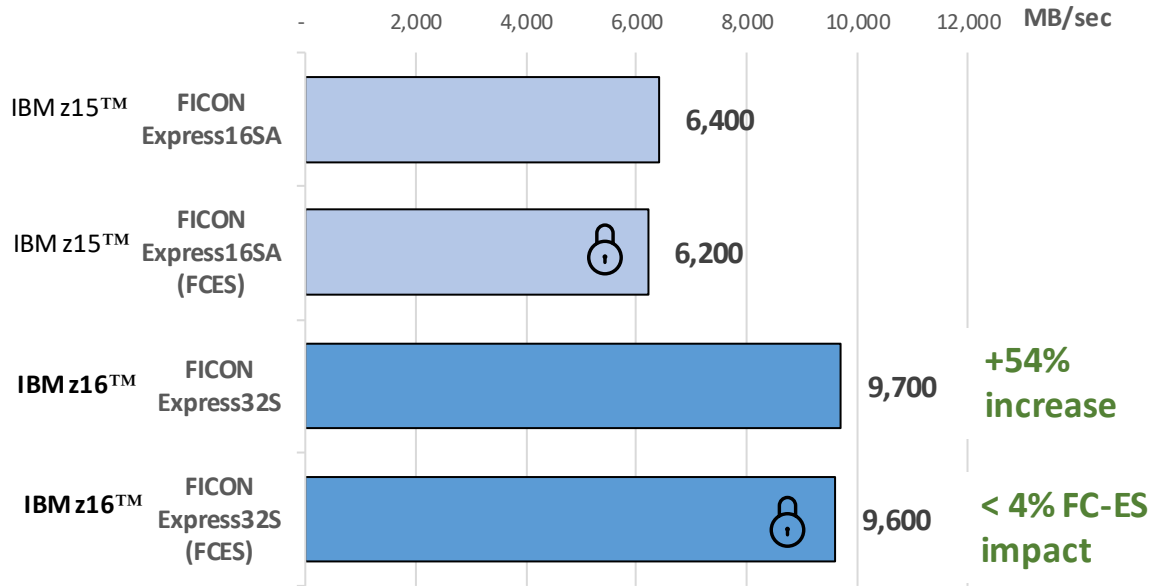
Figure 27 – Maximum FEx32S FCP Large Block Read/Write (mix) IO/sec (Combined Both Ports)
