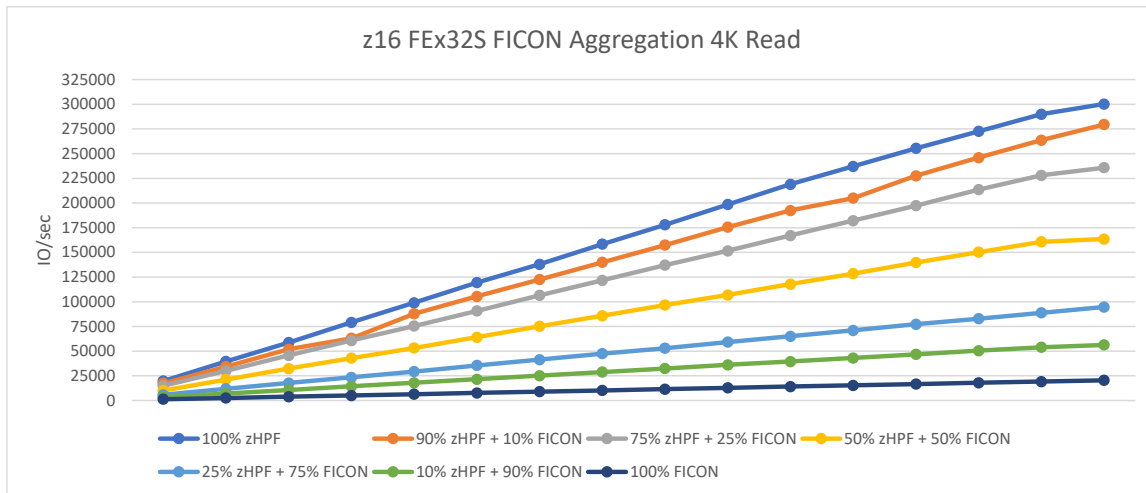
Figure 5 – FICON Aggregation
