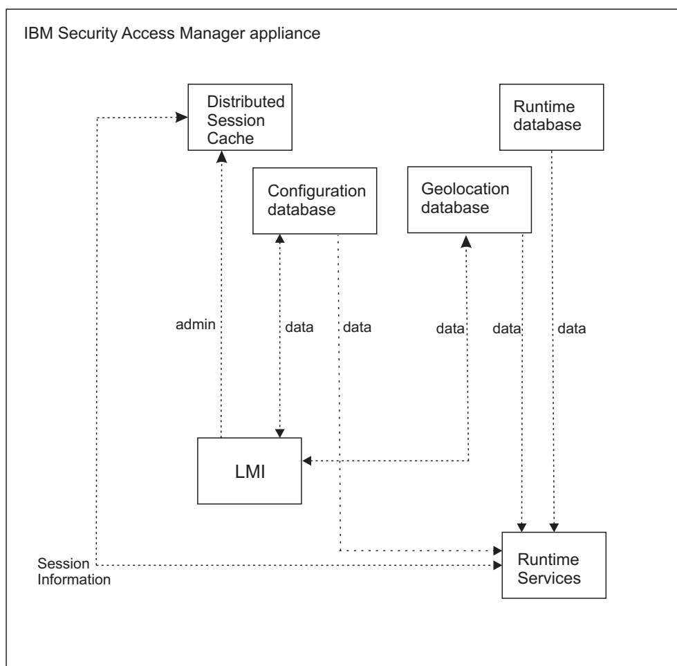
Figure 2. Services architecture
