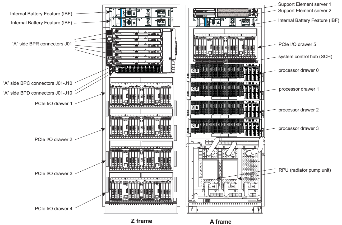
Figure 6. 3906 - front view - radiator-cooled
