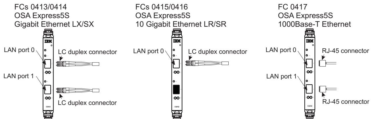
Figure 32. OSA-Express5S features
