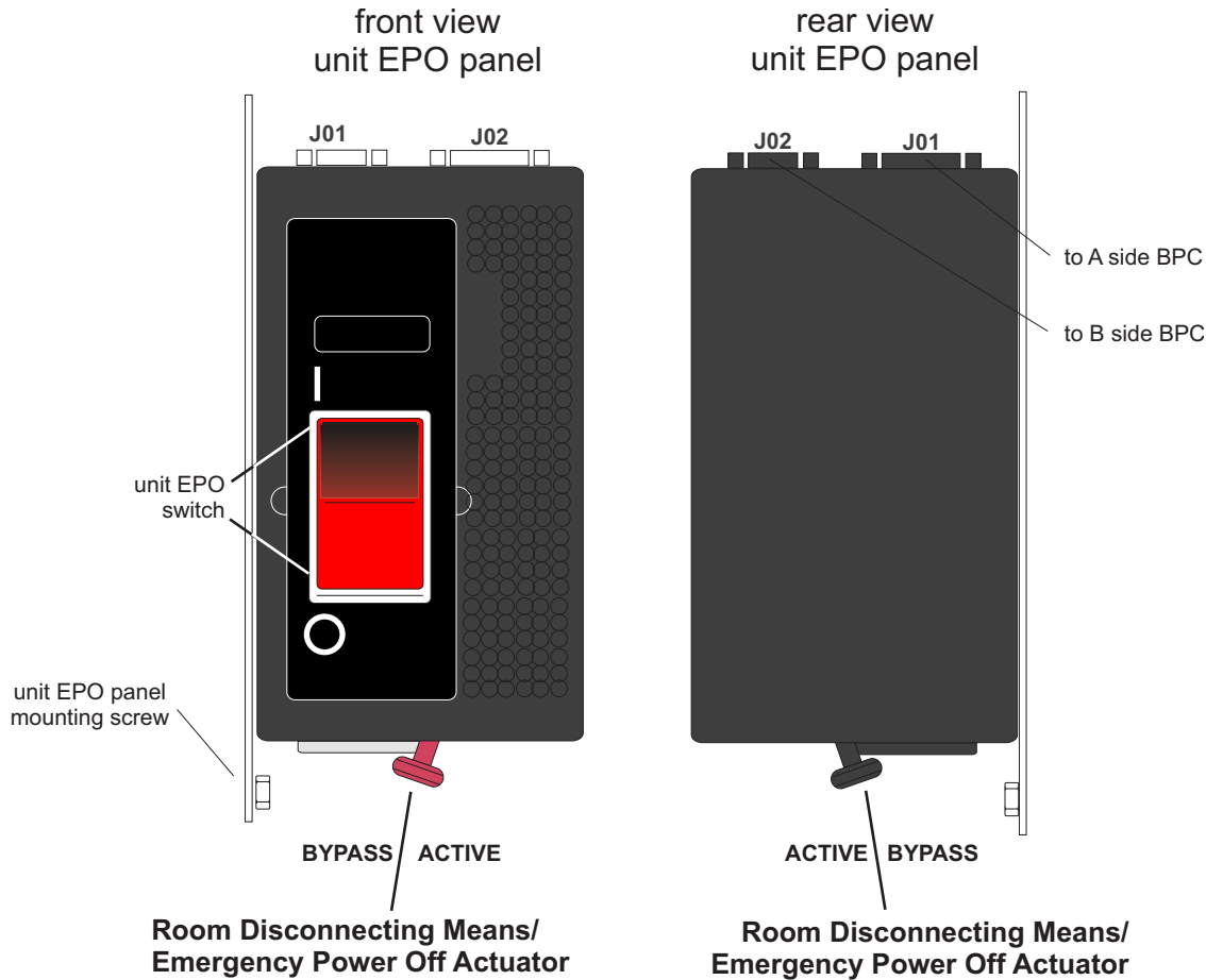
Figure 23. UEPO panels
