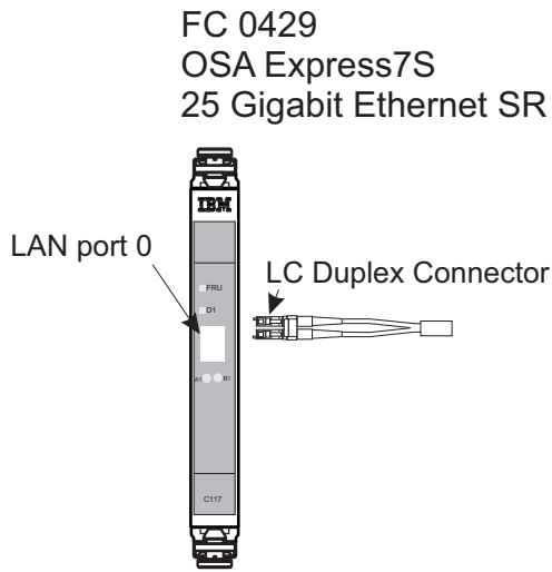
Figure 30. OSA-Express7S 25 GbE feature
