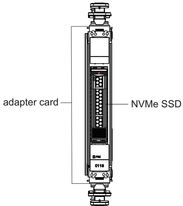
Figure 37. IBM Adapter for NVMe feature
