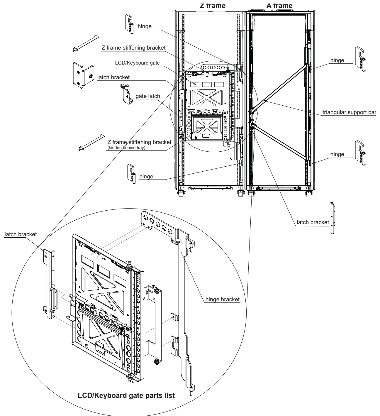
Figure 10. Frame stiffening and tie-down parts list - front frame
