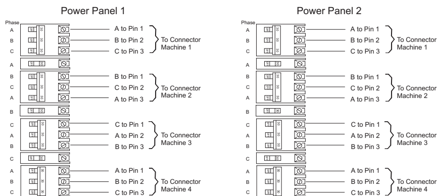
Figure 42. Power load balancing - alternating three-pole and single-pole breakers
