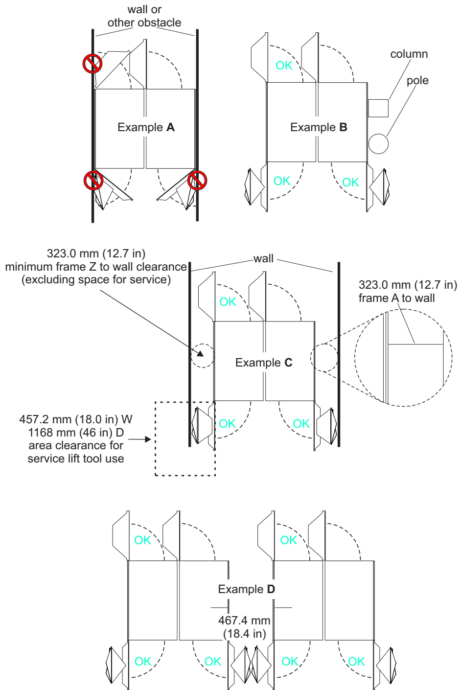
Figure 16. Detailed service clearances - 323.0 mm (12.7 in) cover
