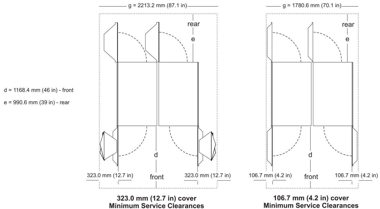
Figure 15. Minimum service clearances
