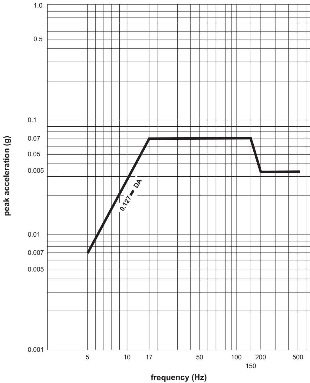
Figure 9. Continuous operational vibration
