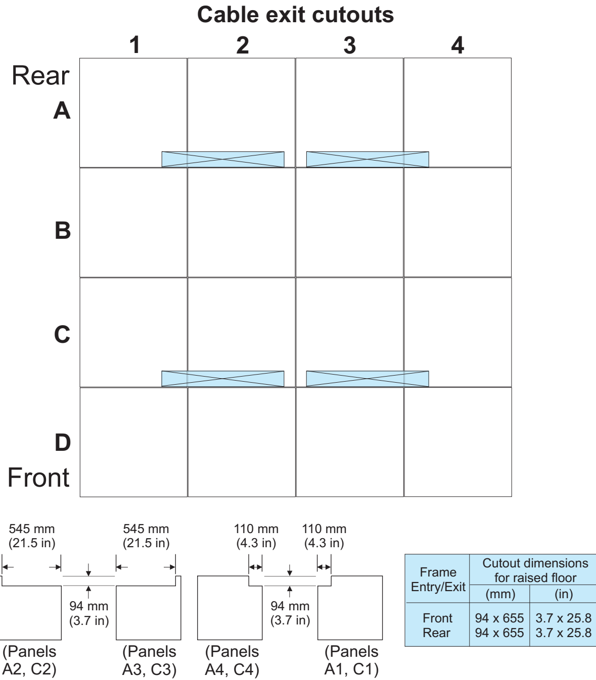
Figure 21. Raised floor with floor panels
