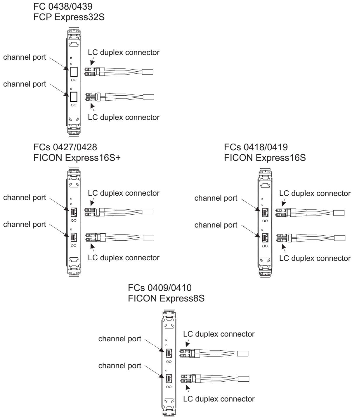
Figure 29. FICON Express features
