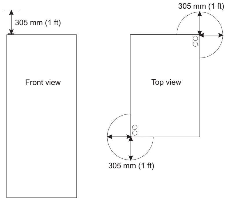
Figure 26. Receptacles for top exit power cords
