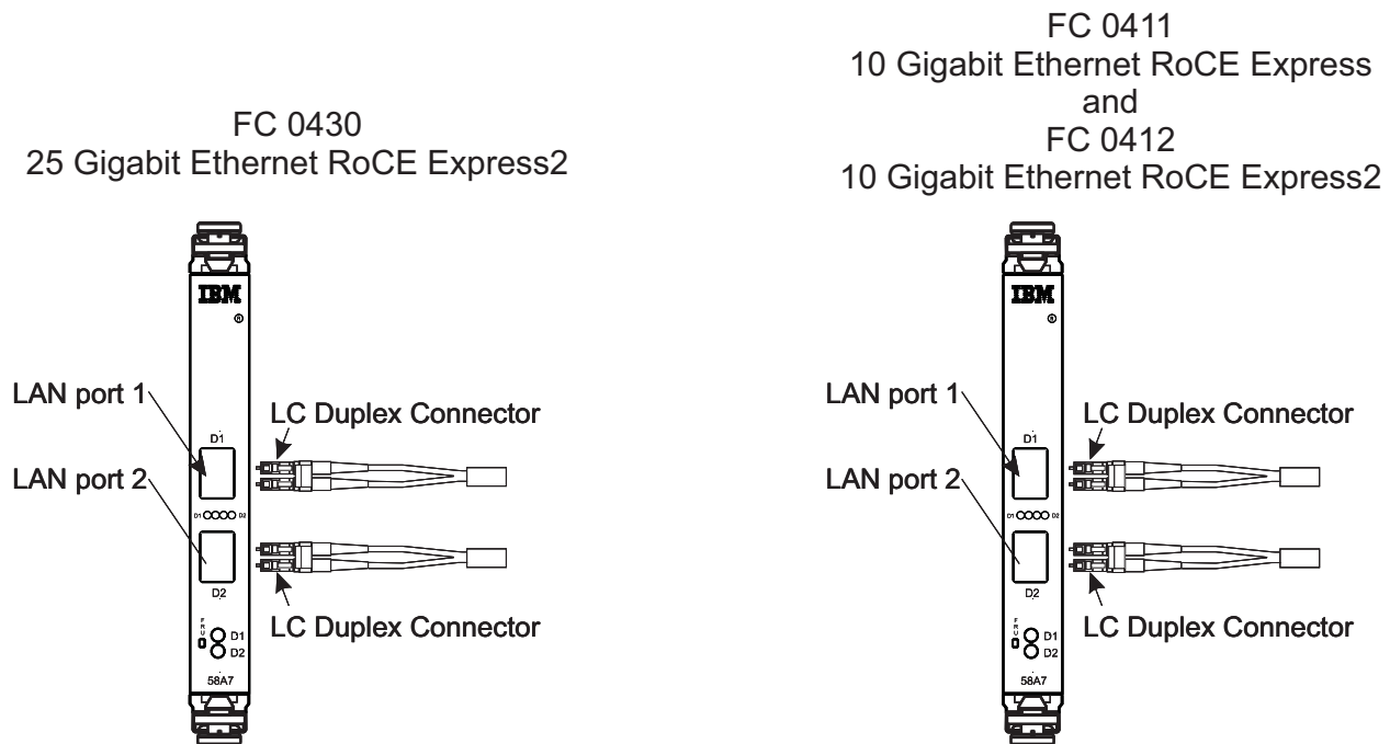
Figure 34. RoCE Express and RoCE Express2 features
