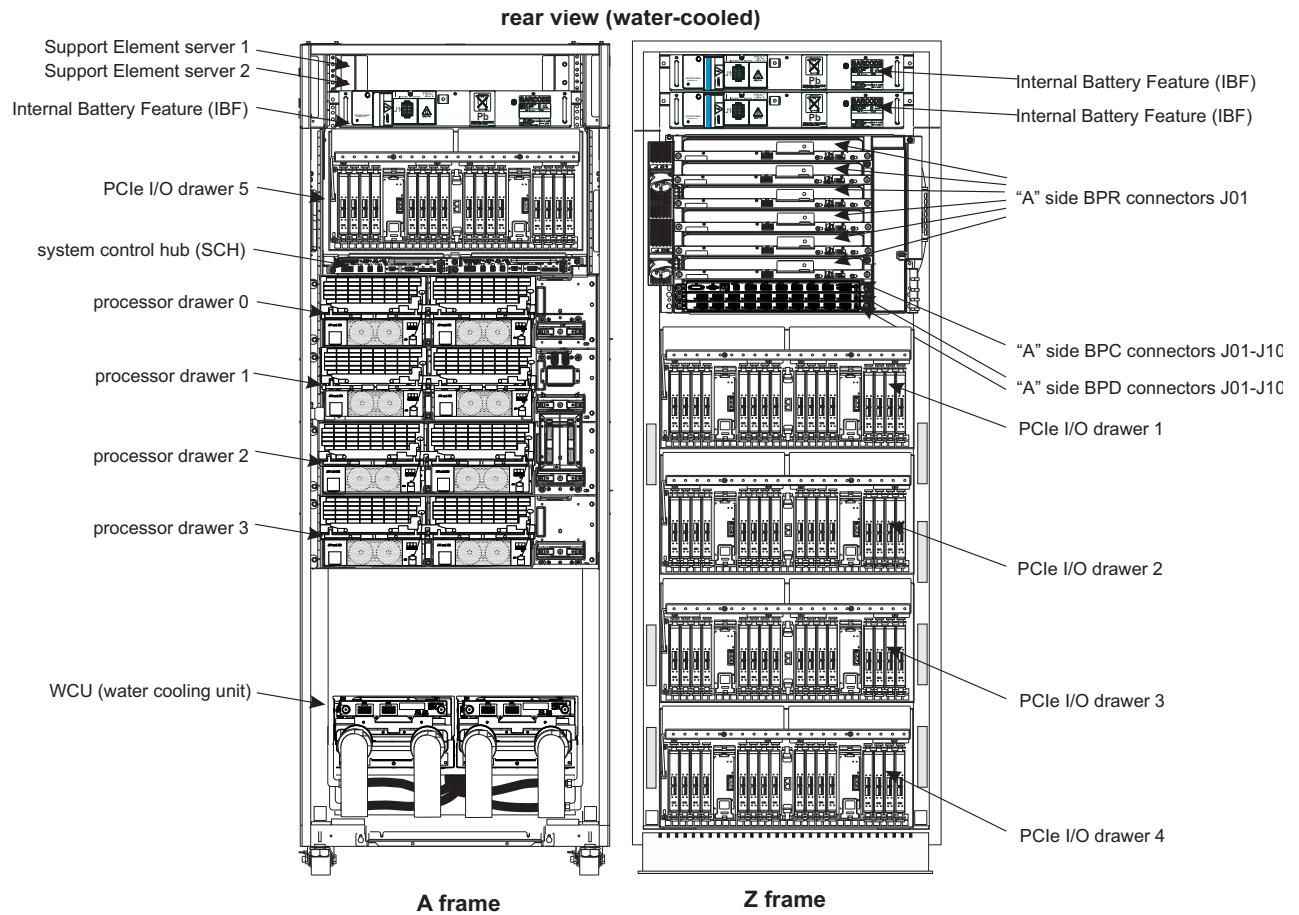
Figure 7. 3906 - rear view - water-cooled
