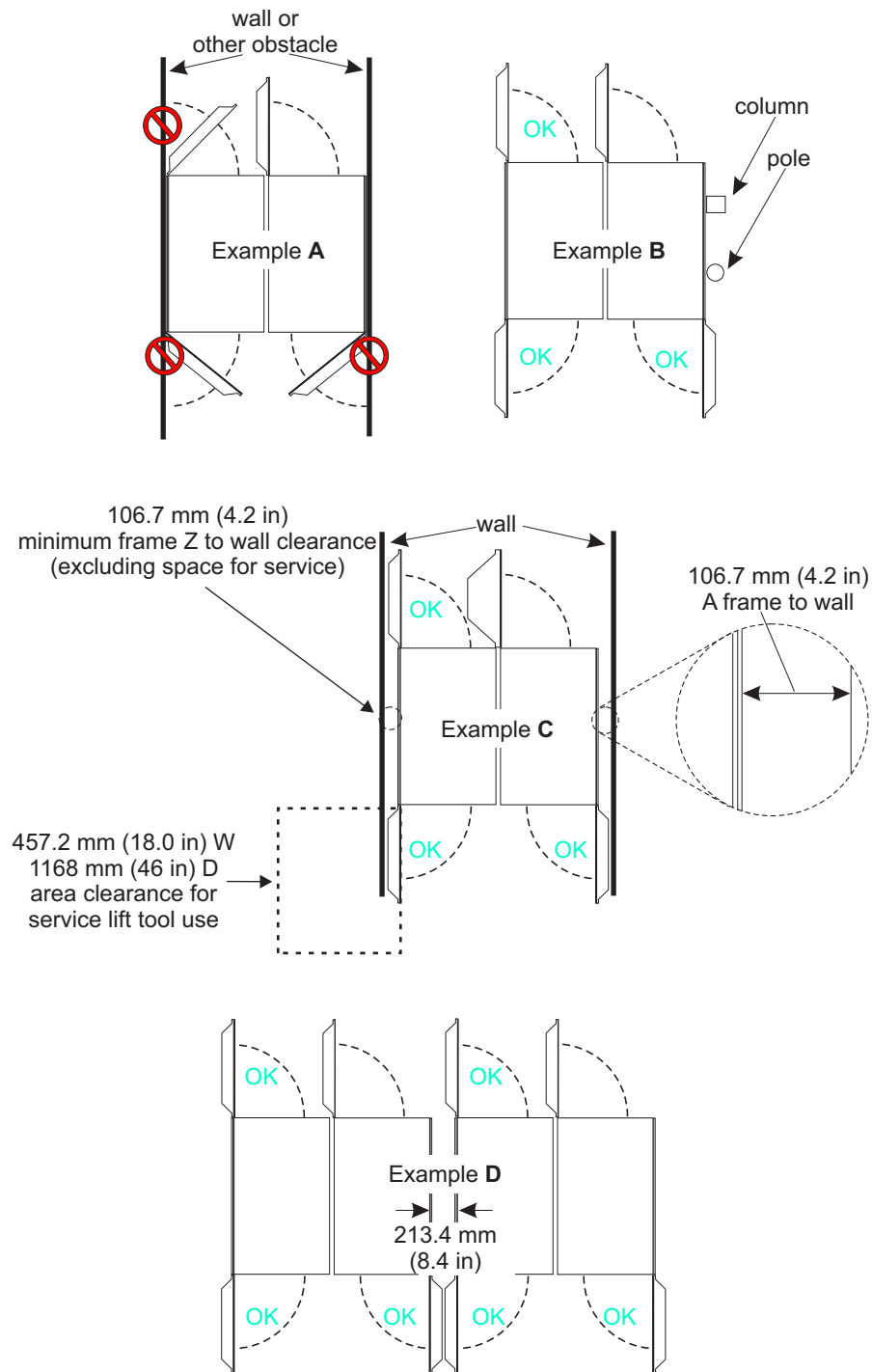
Figure 17. Detailed service clearances - 106.7 mm (4.2 in) cover
