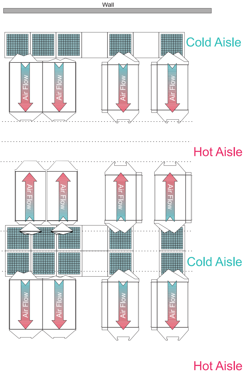
Figure 18. System airflow
