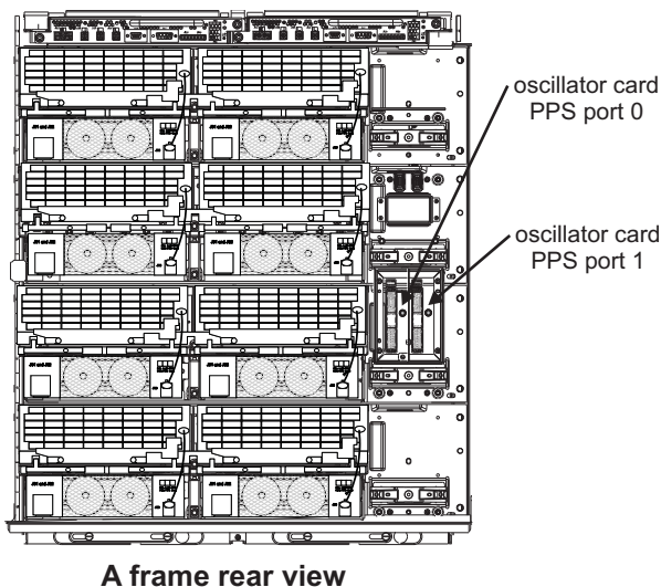
Figure 38. oscillator card location
