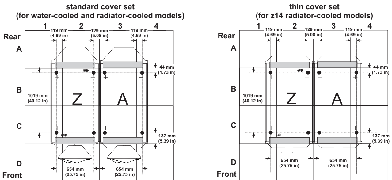
Figure 13. Frame tie-down hole cutouts 600 mm (23.5 in) floor tiles
