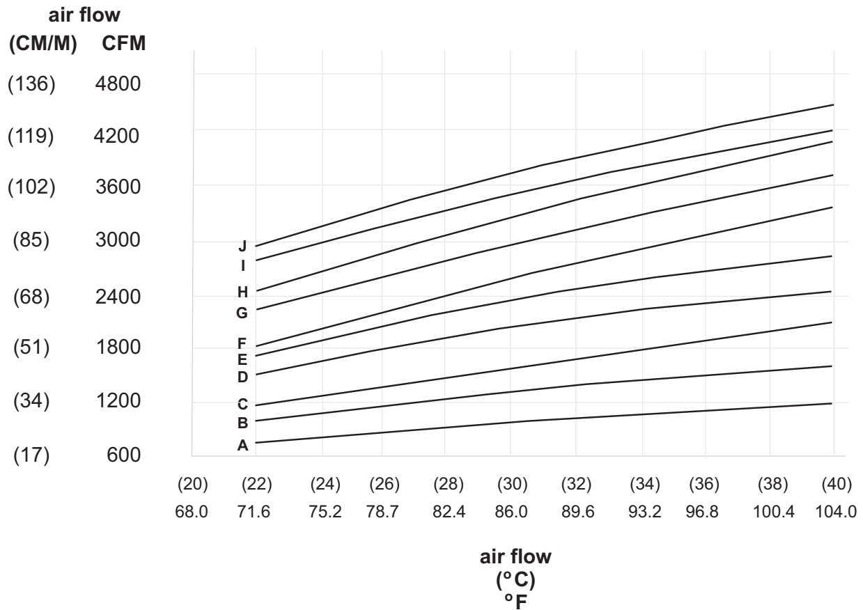
Figure 19. 3906 air flow requirements for data centers below 1500 feet elevation
