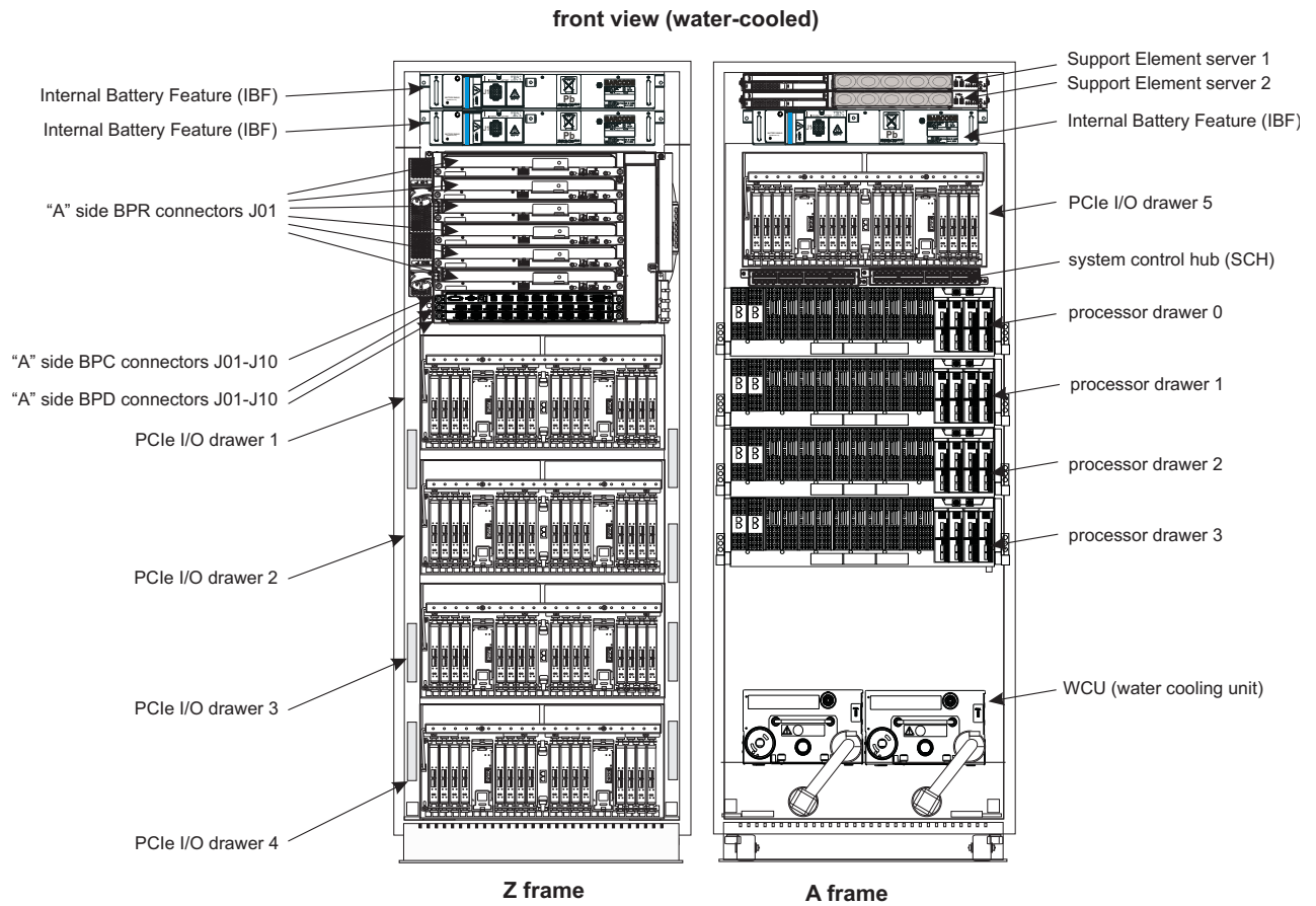
Figure 5. 3906 - front view - water-cooled
