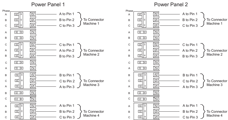
Figure 43. Power load balancing - alternating three-pole and double-pole breakers
