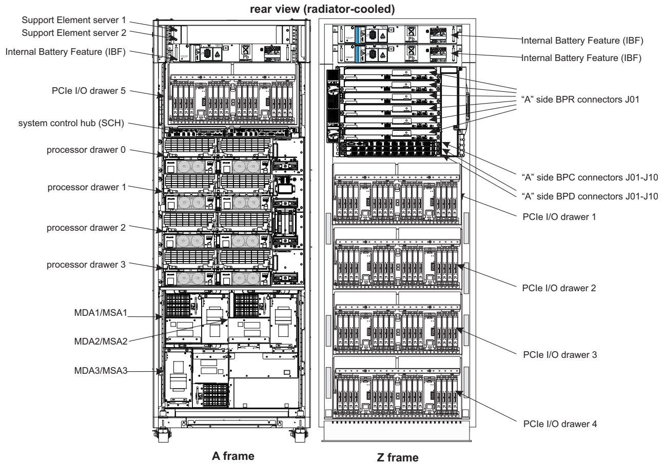
Figure 8. 3906 - rear view - radiator-cooled
