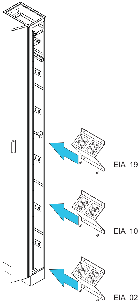
Figure 40. Fiber Quick Connect mounting brackets
