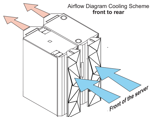
Figure 1. ASHRAE declarations - radiator-cooled
