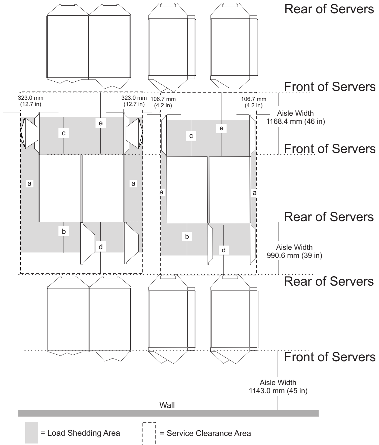
Figure 14. Aisle and service clearances
