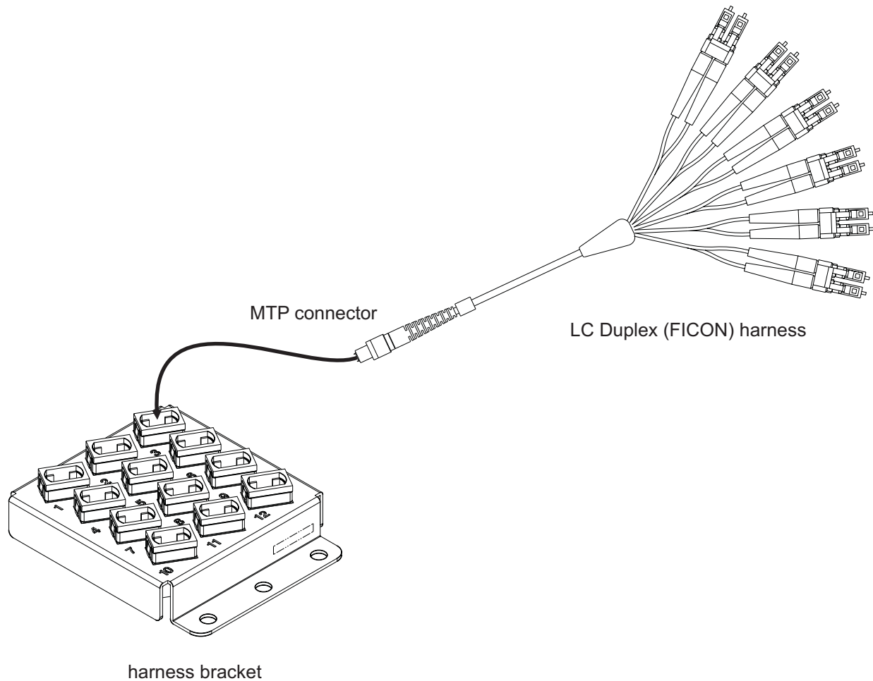
Figure 39. Fiber Quick Connect feature hardware
