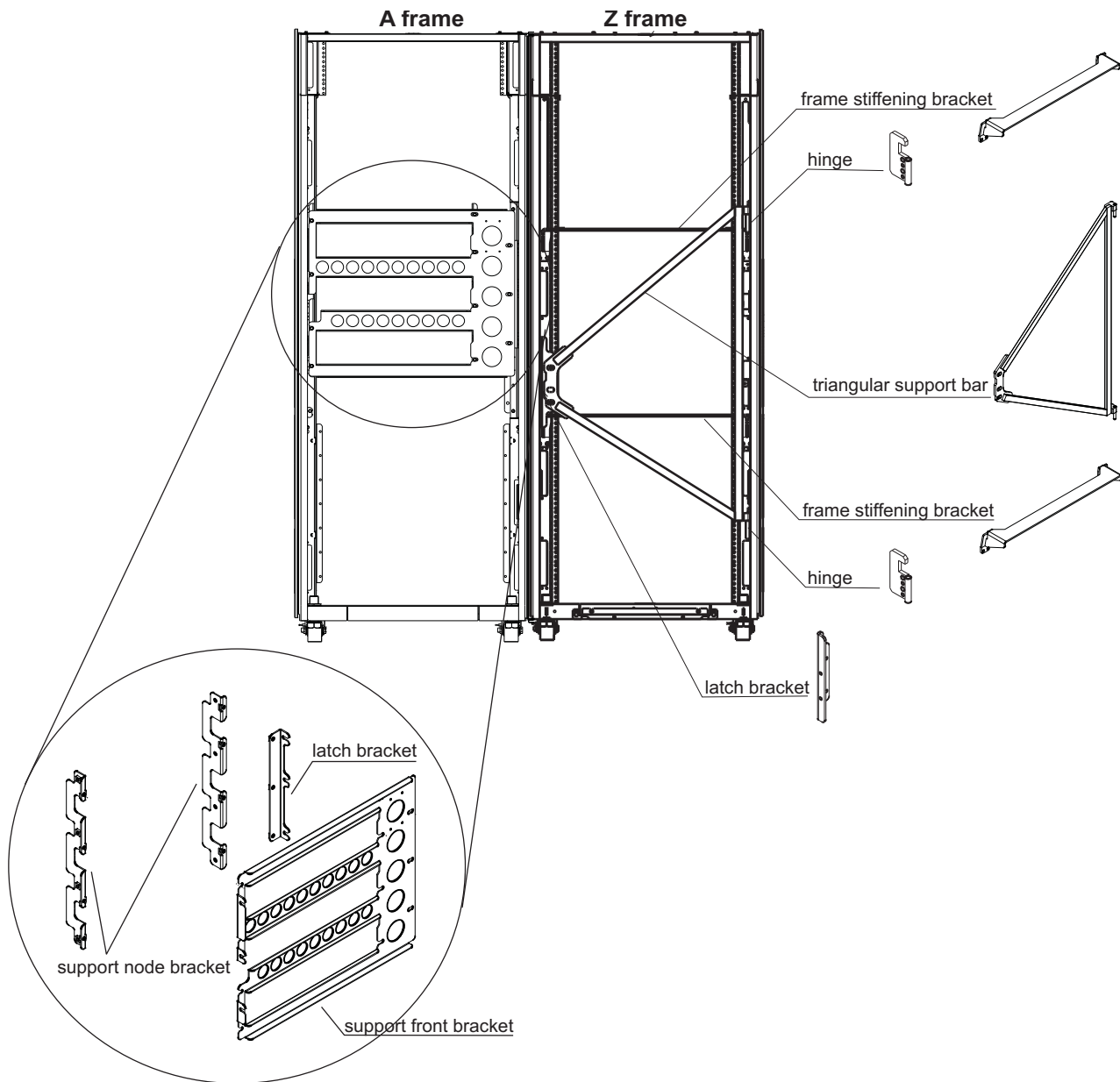
Figure 11. Frame stiffening and tie-down parts list - rear frame
