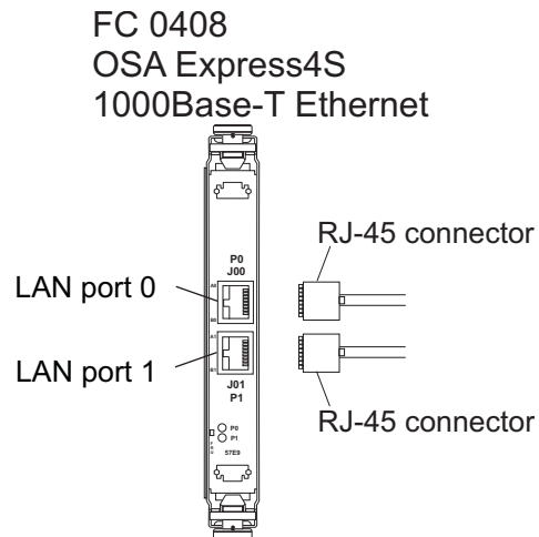
Figure 33. OSA-Express4S features
