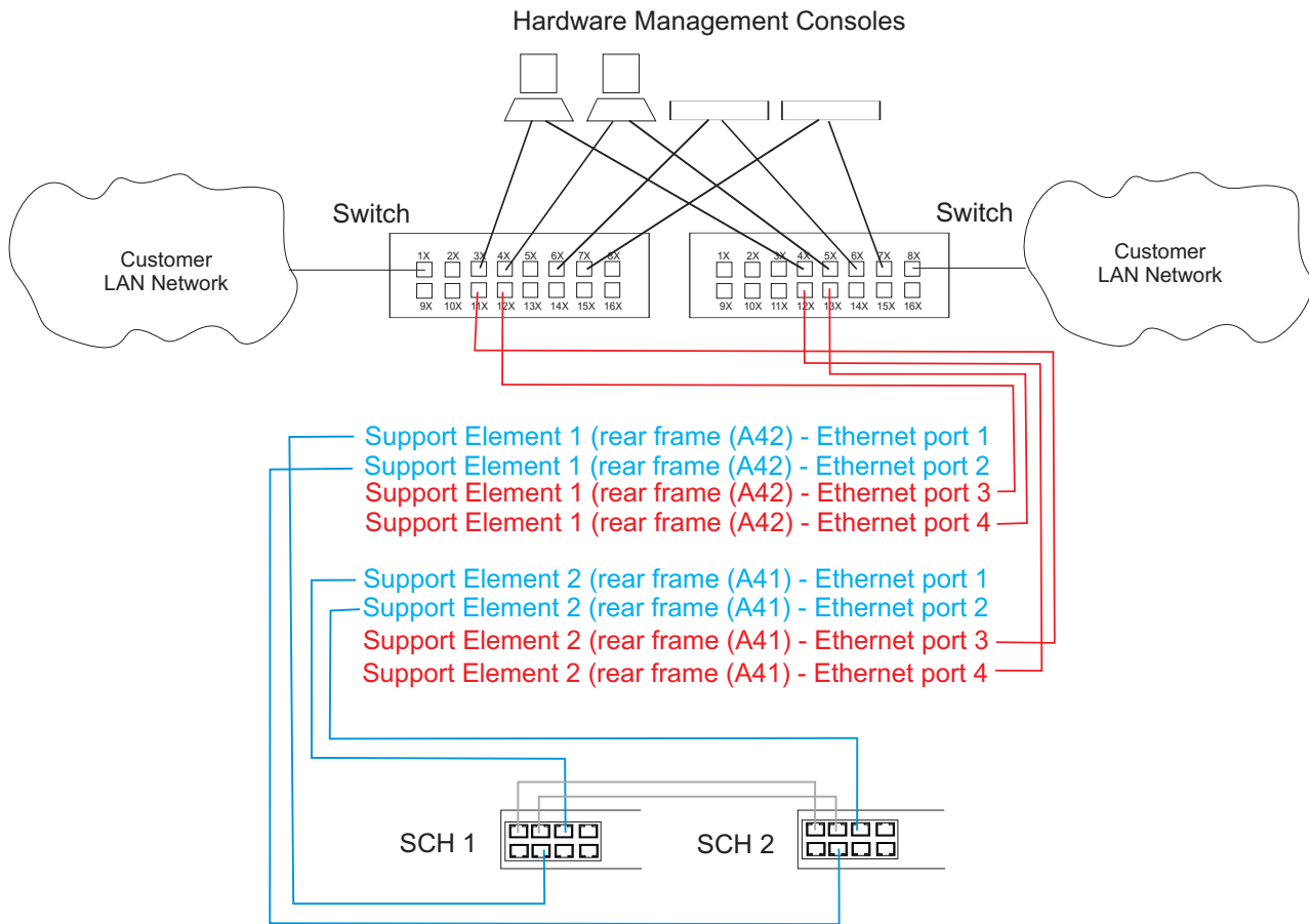
Figure 27. Two-switch configuration
