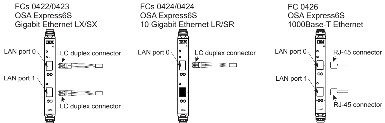
Figure 31. OSA-Express6S features
