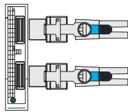
PCIe Interconnect
