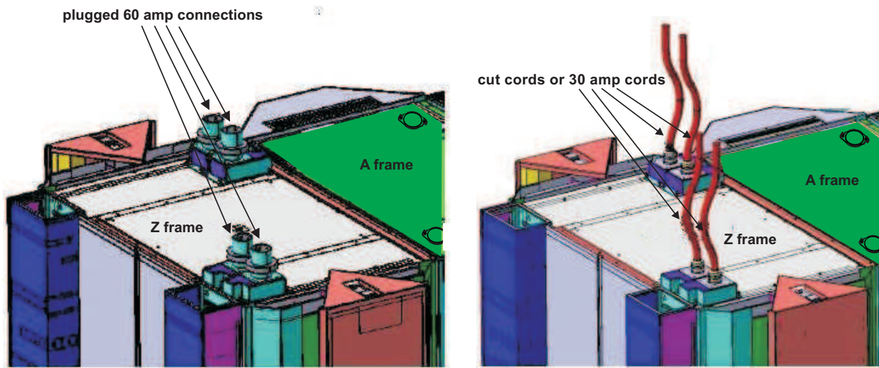
Figure 25. Top exit power cords - plugged 60 amps connection, cut cord or 30 amp cord connection
