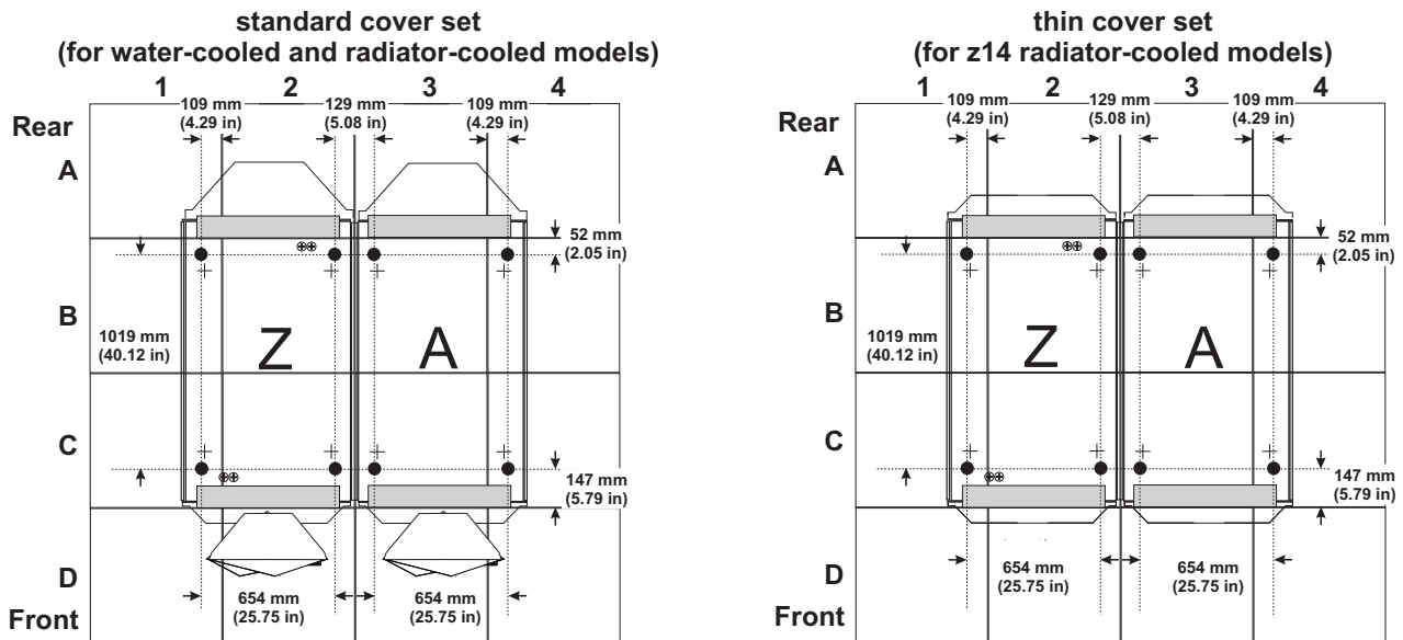
Figure 12. Frame tie-down hole cutouts 610 mm (24 in) floor tiles
