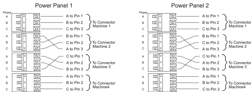
Figure 41. Power load balancing - three-pole breakers
