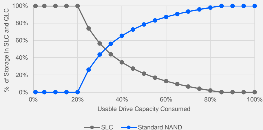
SLC vs. Standard NAND Used for Storage
