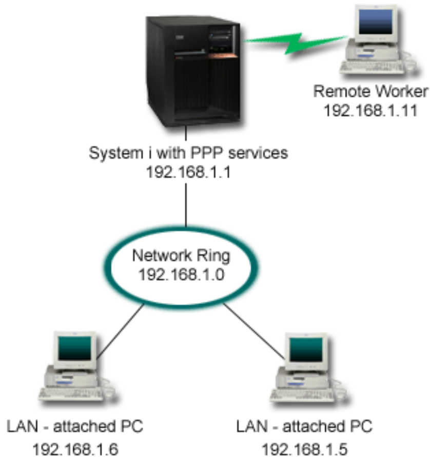
Figure 4. Connecting remote clients to your system
