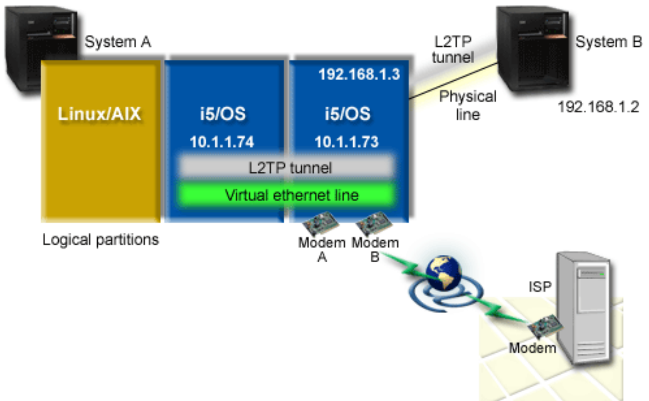
Figure 9. Multiple systems sharing the same modem for dial-up connections
