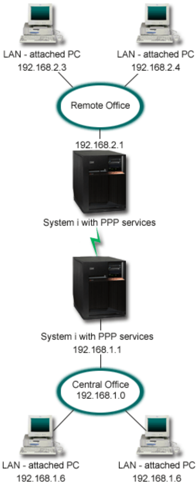
Figure 6. Connecting your corporate and remote networks with a modem
