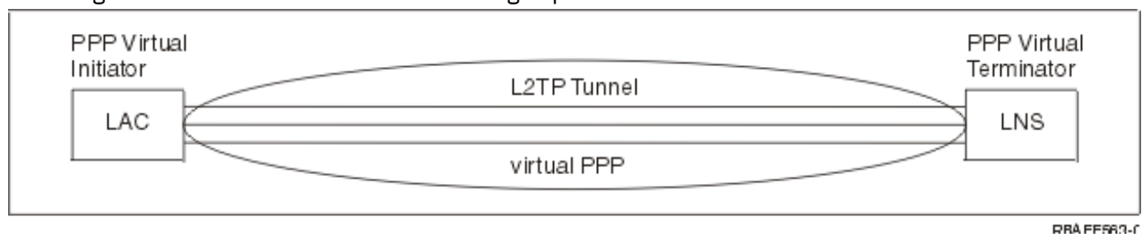
Figure 10. PPP virtual initiator or PPP virtual terminator
