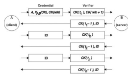
Figure 16. Authentication Process
