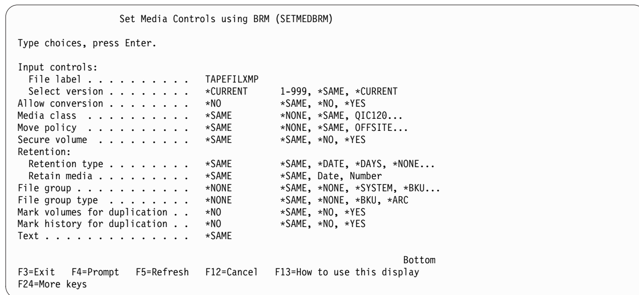
Figure 18. SETMEDBRM Command Prompt Screen for Program Input
