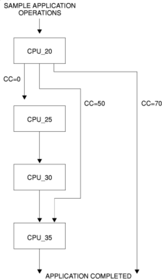
Figure 66. Completion Code Driven Application Flow
