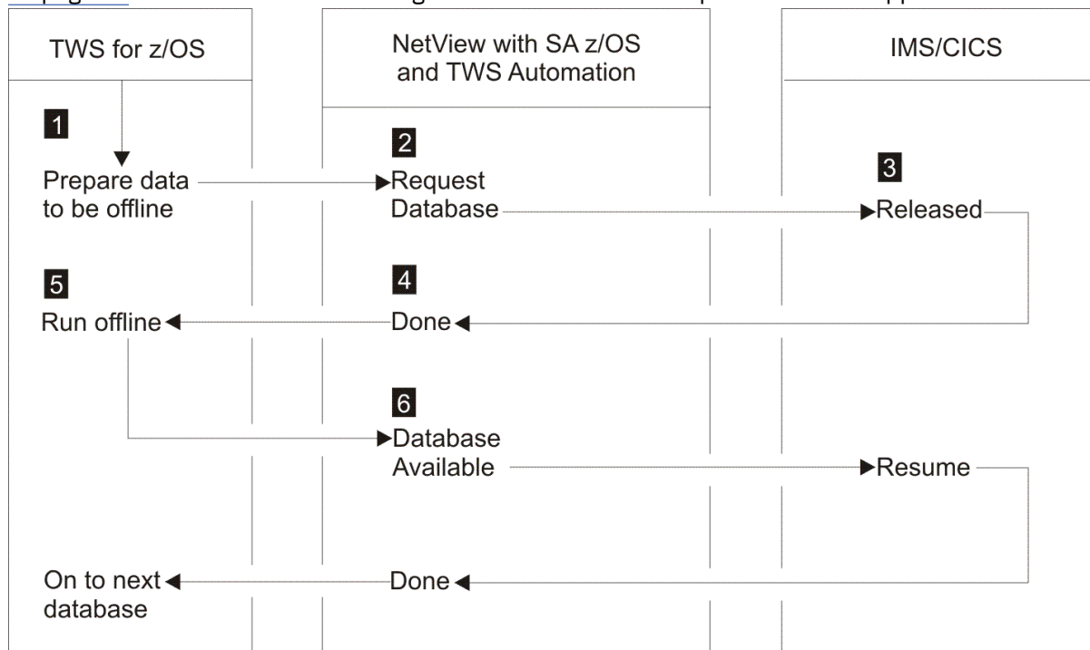
Figure 2. Example of Cycling Individual Online Databases
