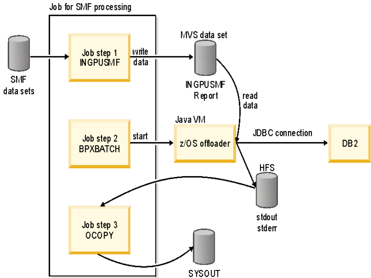
Figure 22. SMF Processing with z/OS Offloader
