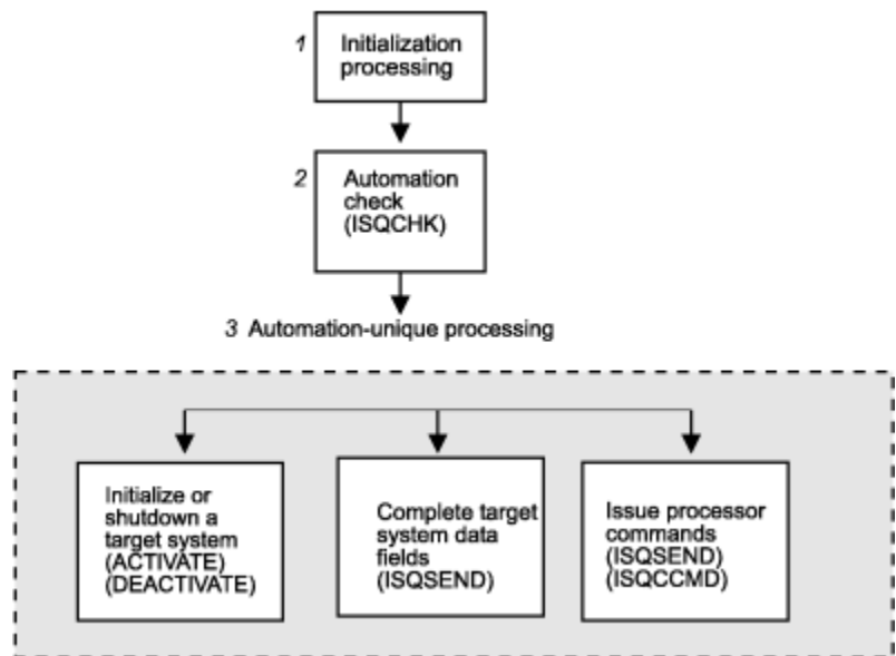
Figure 3. Automation Procedures for Processor Operations
