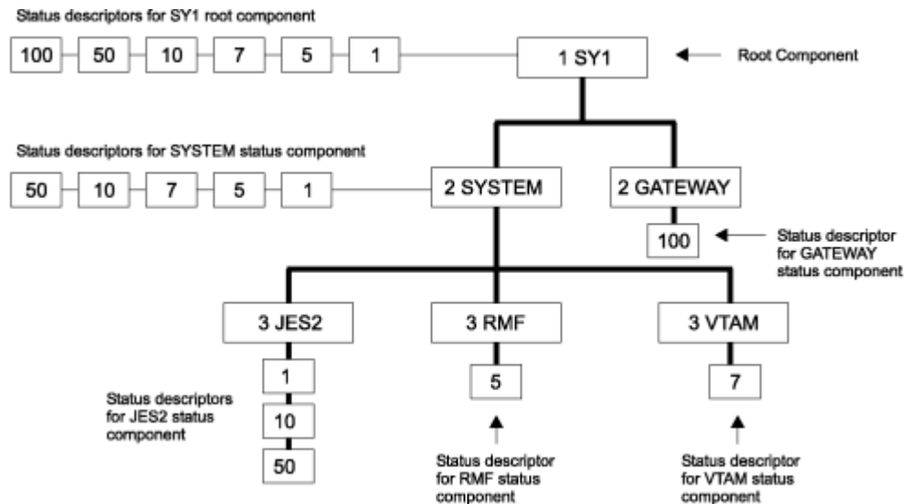
Figure 55. Status Descriptors Chained to Status Components
