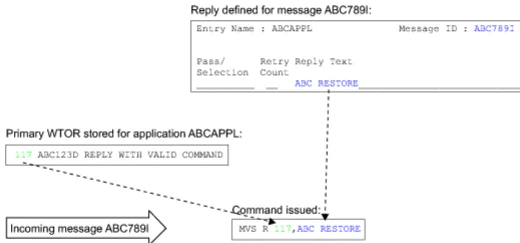
Figure 31. Example Processing of a Primary WTOR
