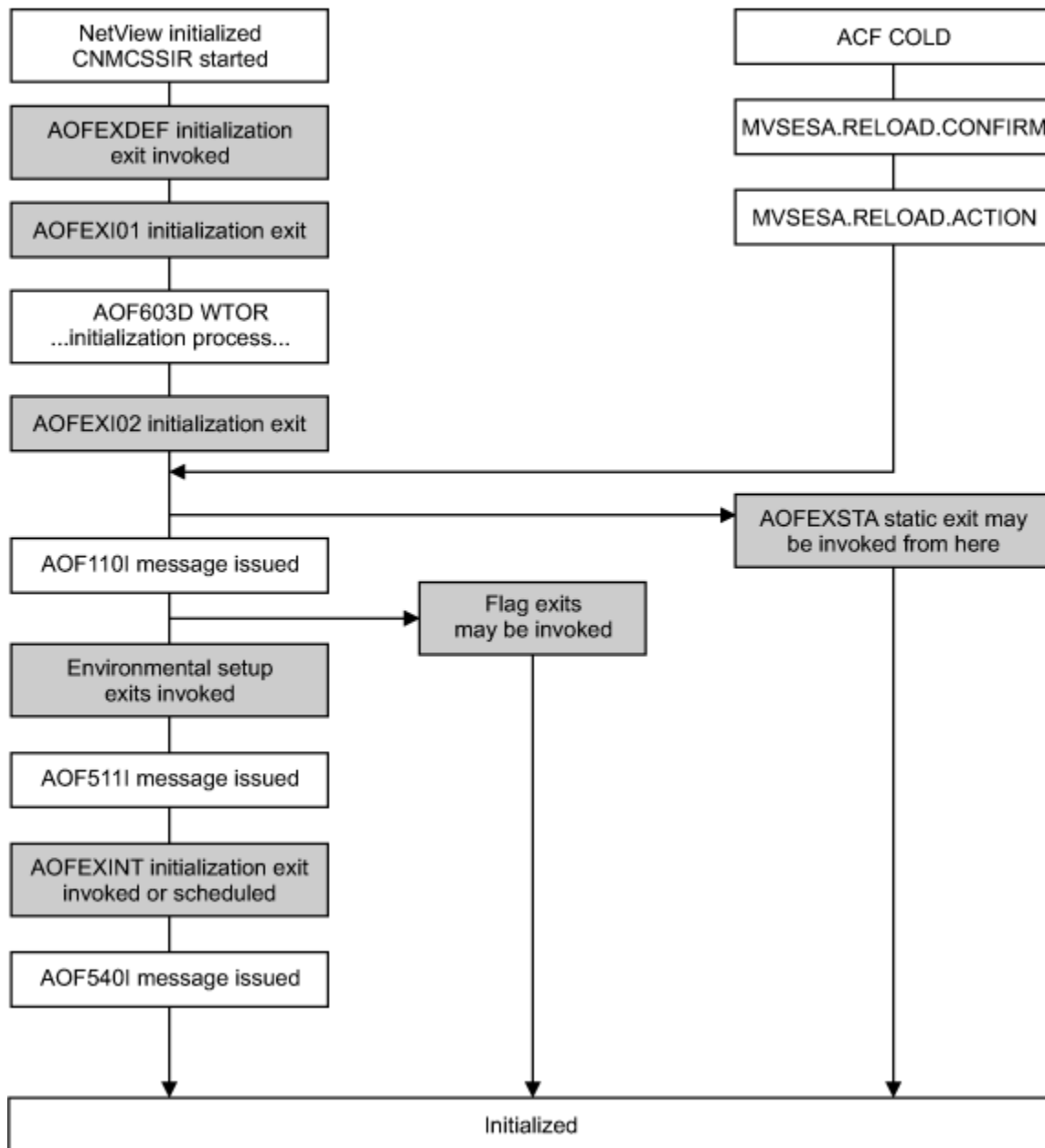
Figure 32. SA z/OS Exit Sequence during SA z/OS Initialization
