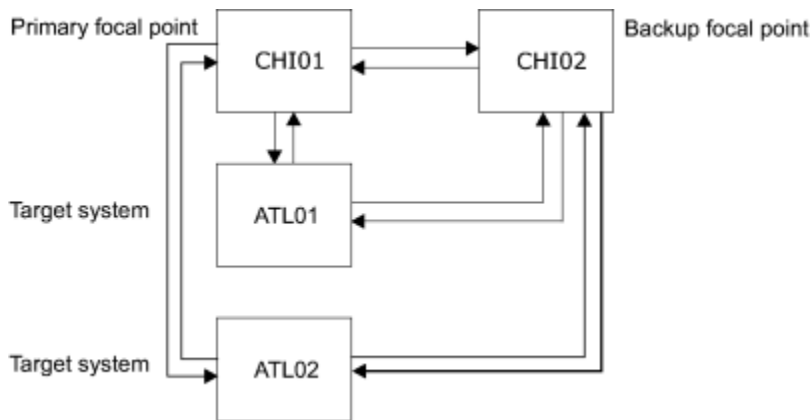
Figure 29. Focal Point Forwarding Definitions for Systems
