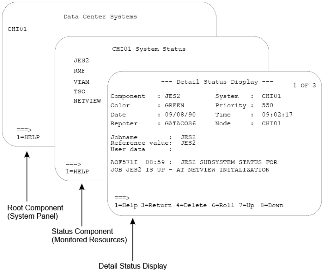
Figure 53. Example SDF Panels
