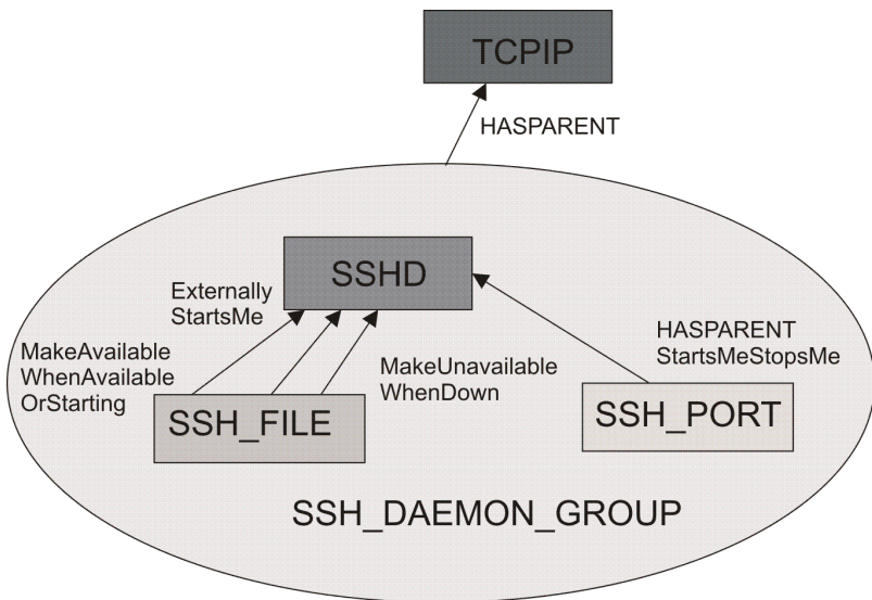
Figure 25. SSH Daemon Listening
