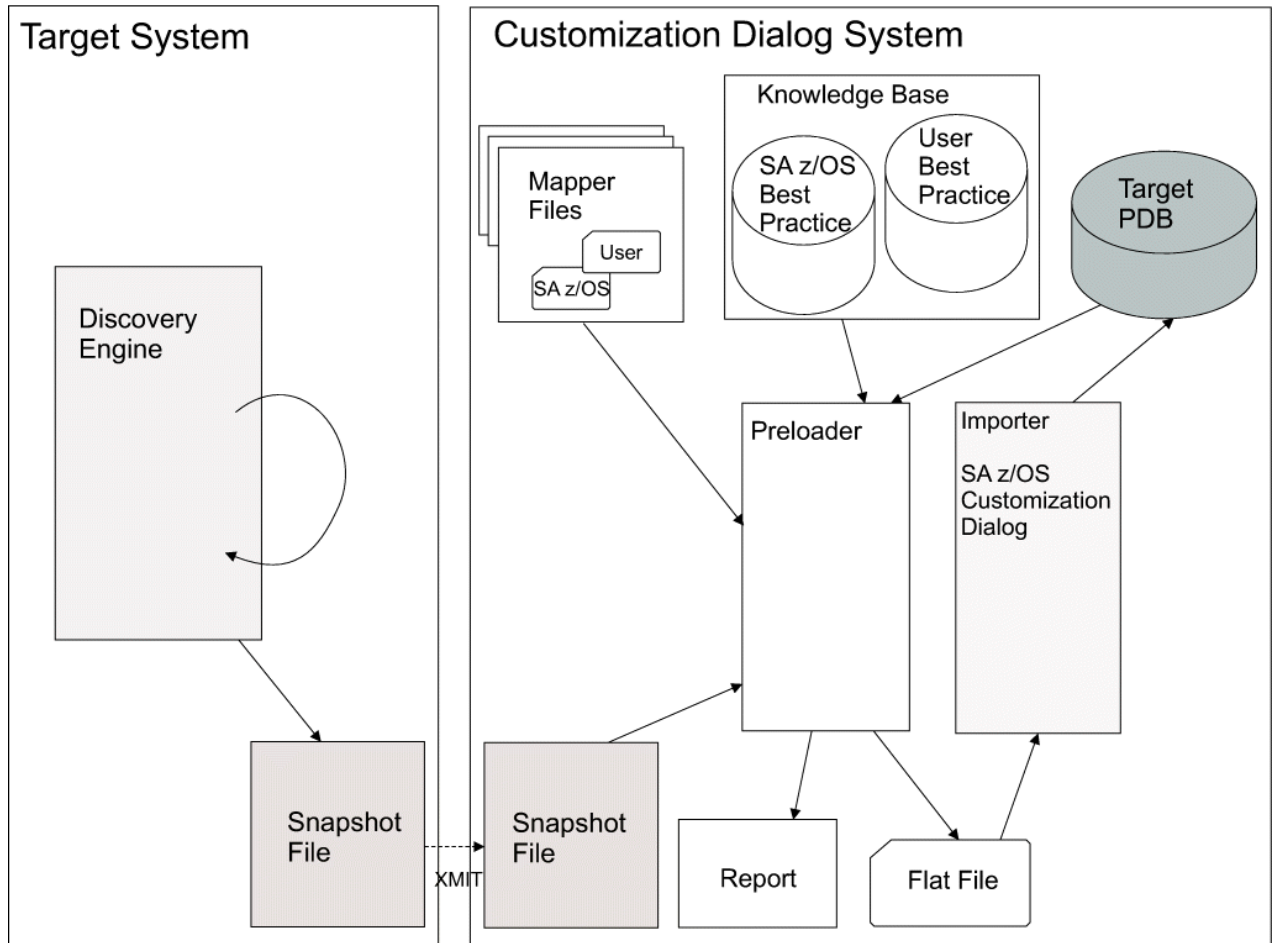
Figure 49. Automated Discovery Overview
