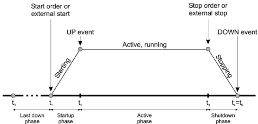
Figure 21. Events in the Lifecycle of an Application
