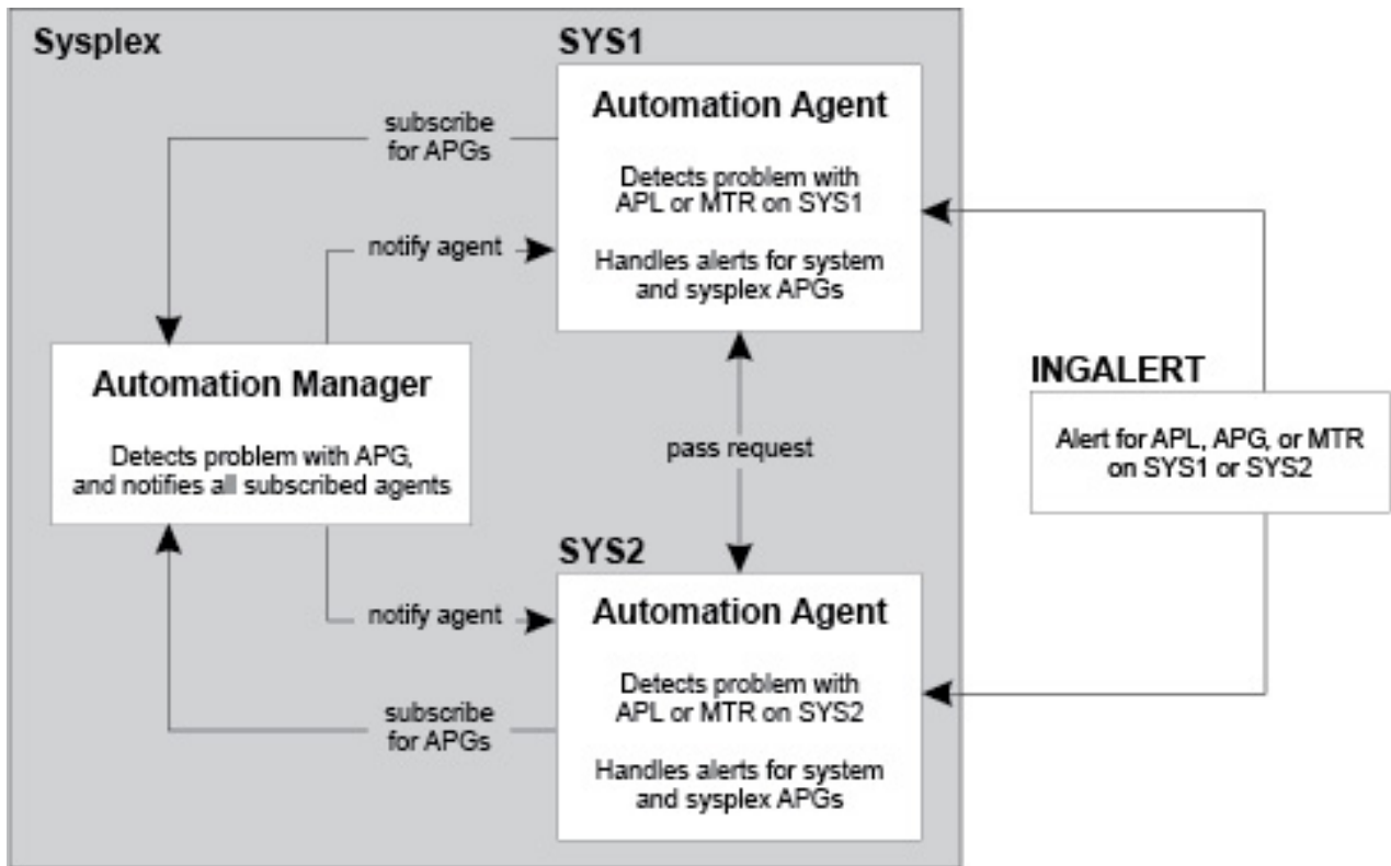
Figure 20. Alert Communication Flow
