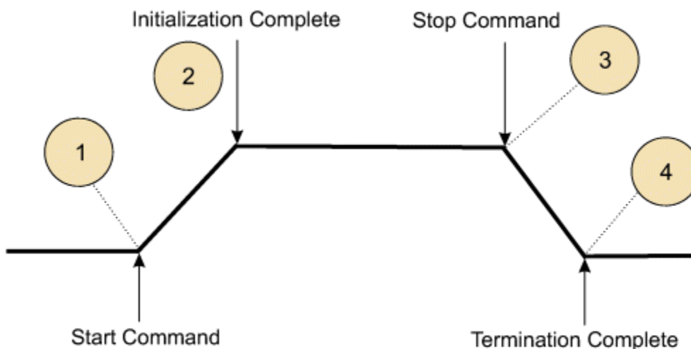
Figure 1. Application Lifecycle
