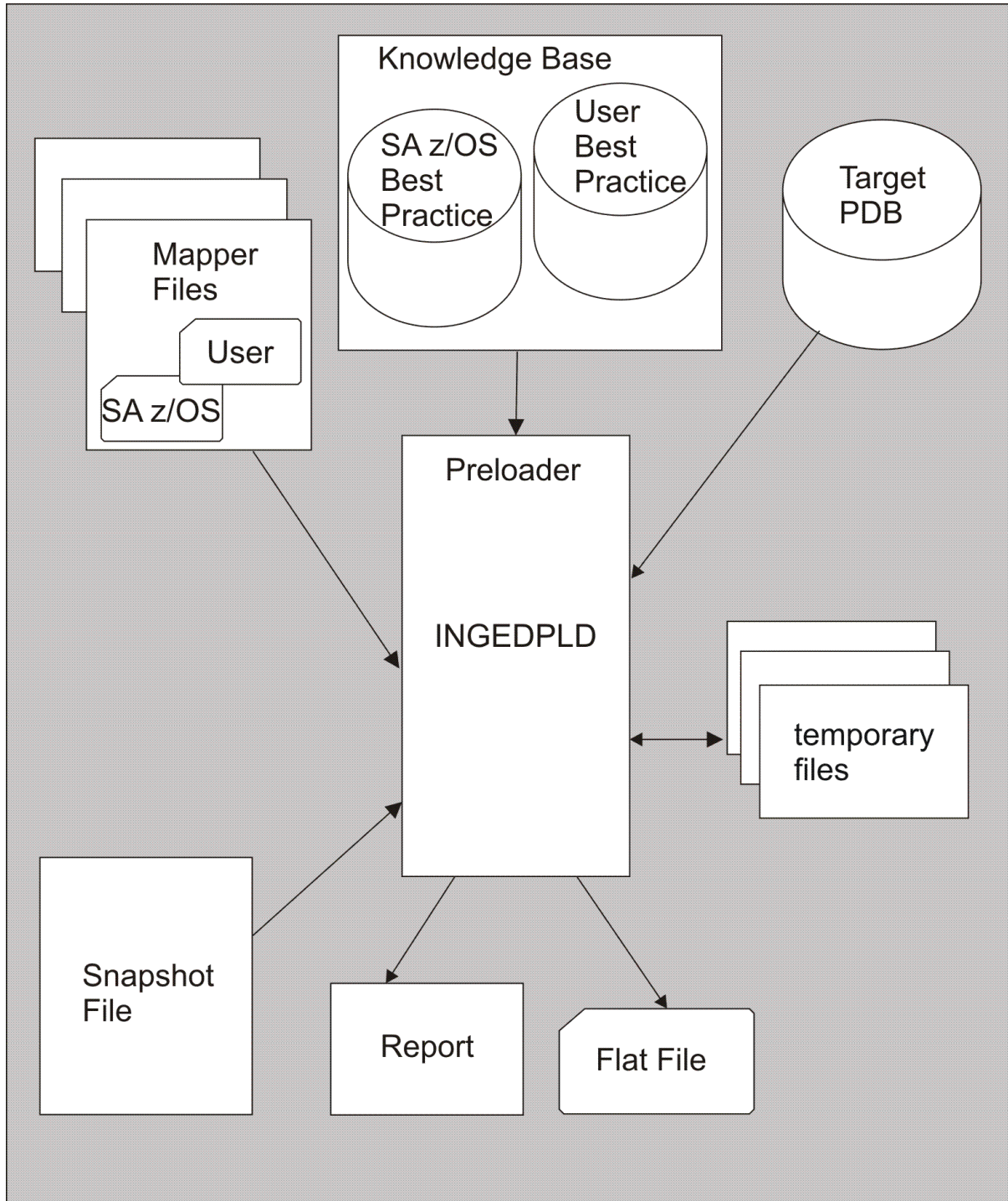
Figure 51. Preloader Processes
