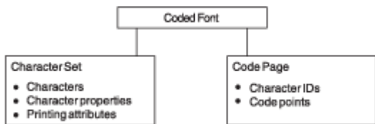
Figure 9. Font components
