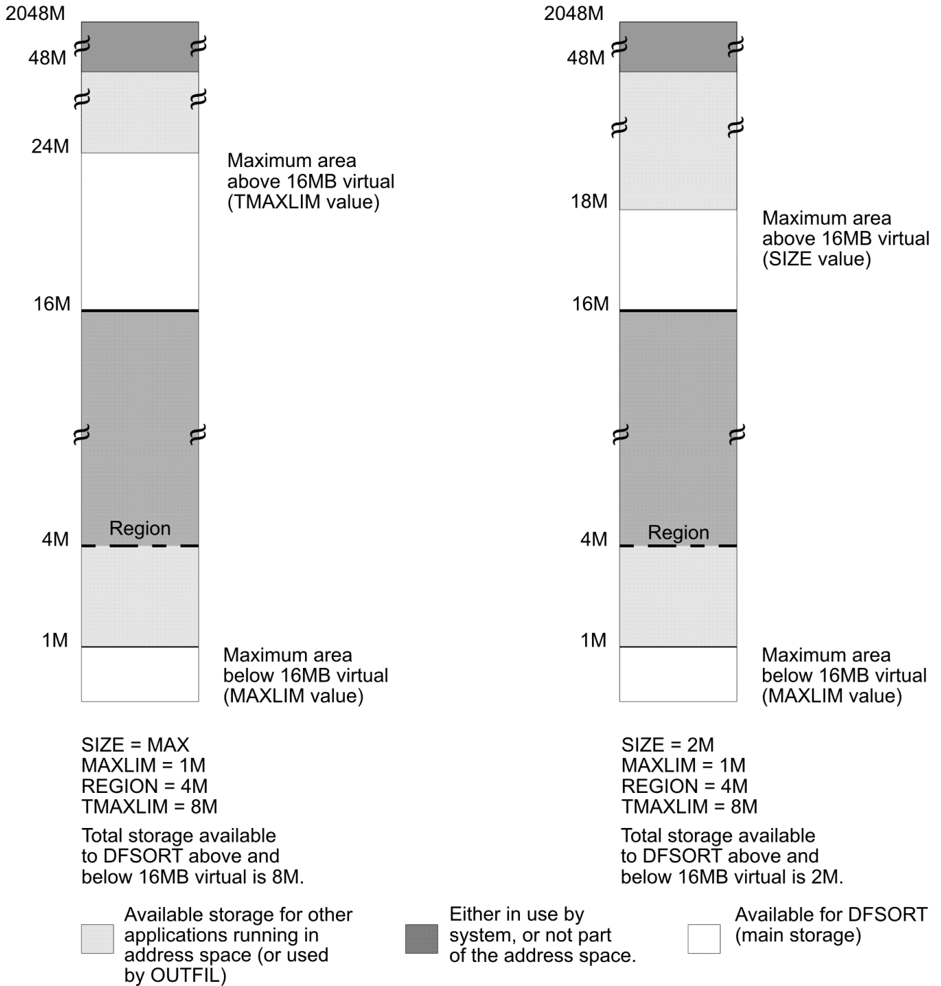
Figure 7: Effect of TMAXLIM Option on Storage
