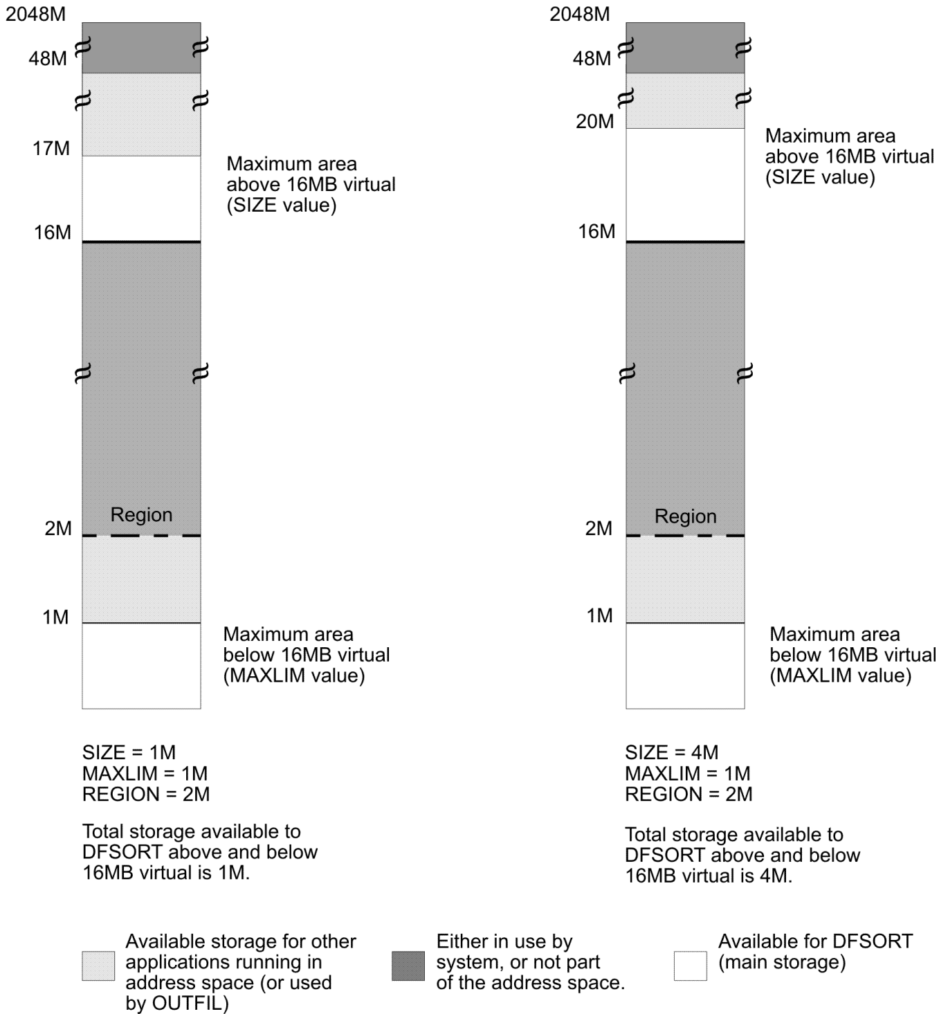
Figure 6: Storage Comparisons for SIZE and REGION
