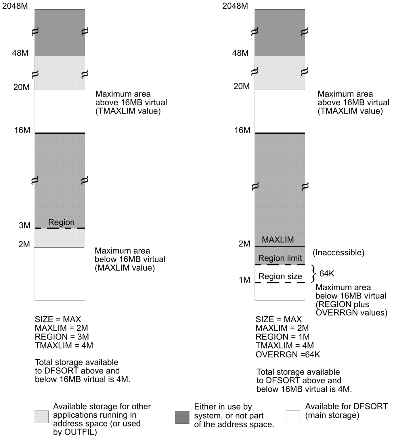
Figure 8: Effects of MAXLIM Option on Storage
