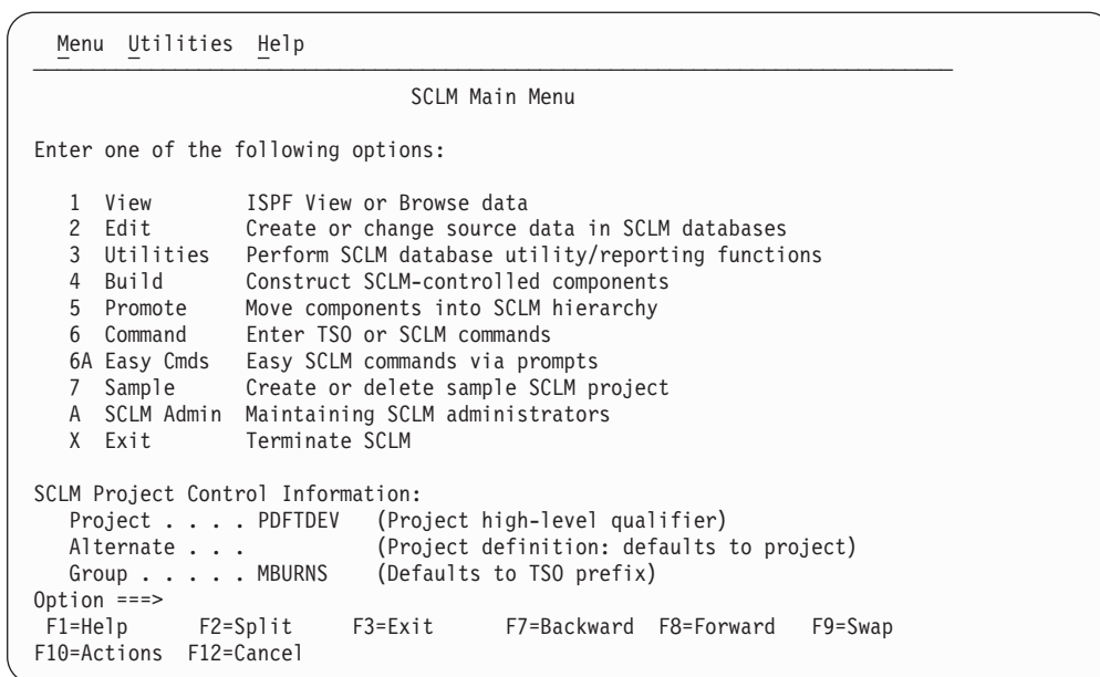
Figure 67. SCLM Main Menu Panel (FLMDMN)
