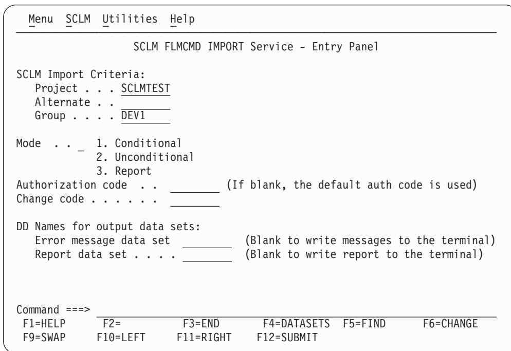
Figure 199. IMPORT Service panel
