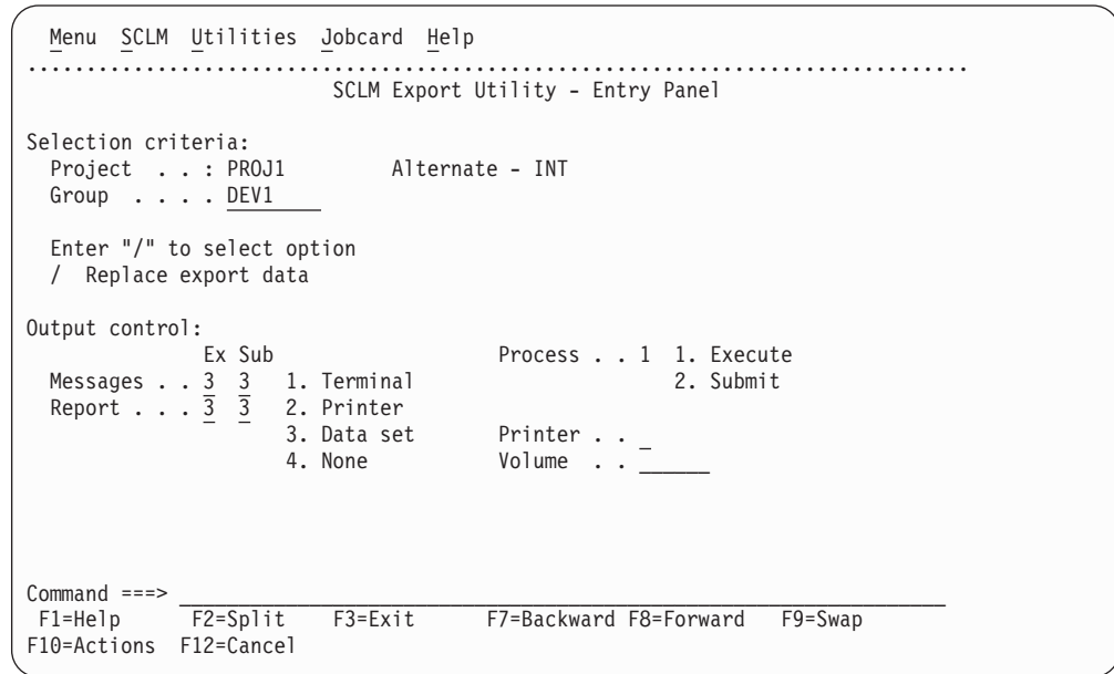
Figure 101. SCLM Export Utility (FLMDXE#P)
