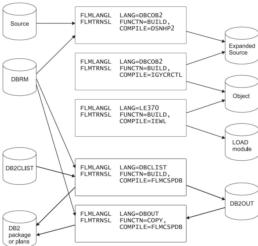
Figure 155. DB2CLIST: flow of processing through the translators
