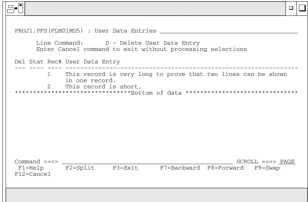
Figure 79. User Data Entries (FLMUSE#P)
