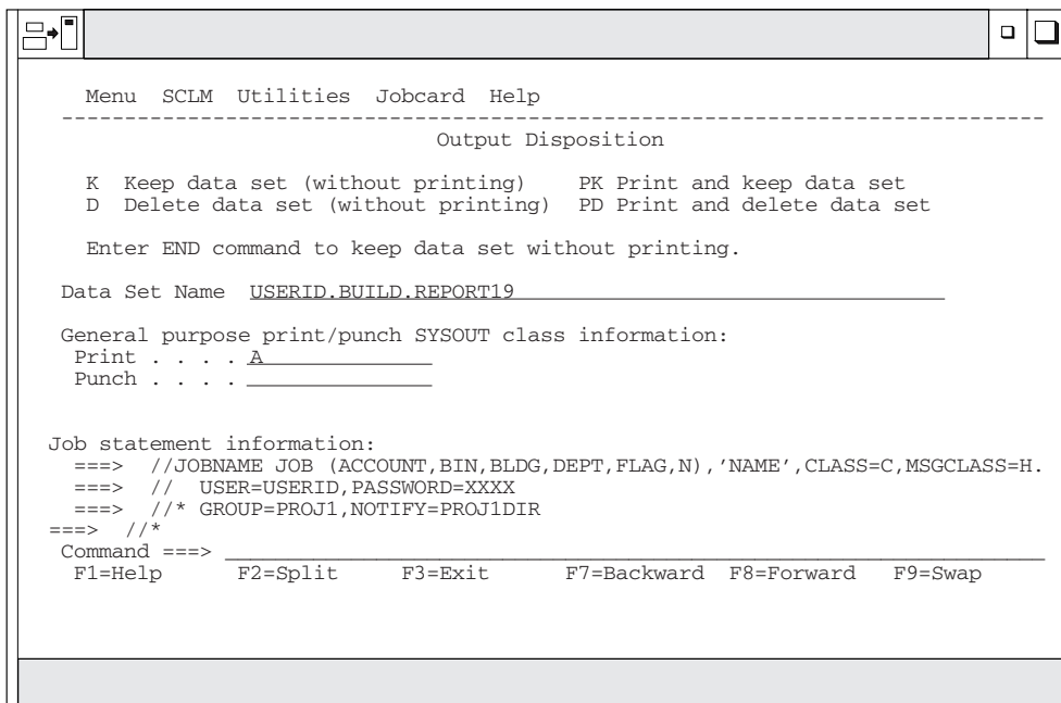
Figure 143. Output Disposition (FLMDEXT)
