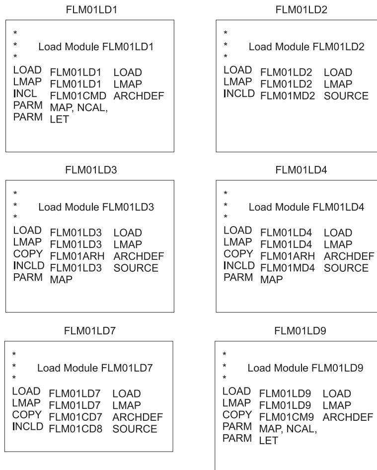
Figure 149. Architecture Members for Application Sample FLM01AP1 (Part 1 of 2)
