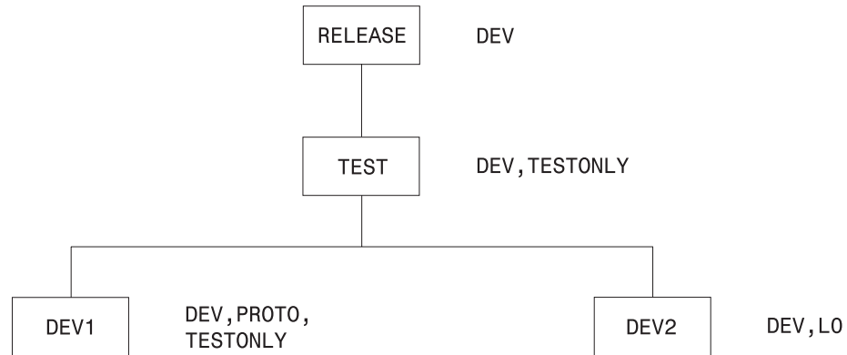
Figure 6. Sample Hierarchy with Authorization Codes
