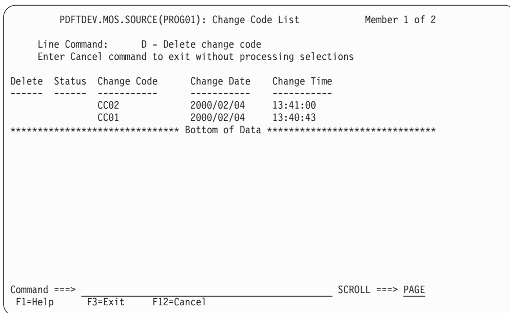
Figure 77. Change Code List - Records That Can Be Deleted (FLMUSC#P)
