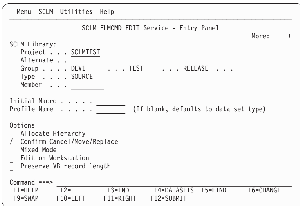
Figure 196. EDIT Service panel
