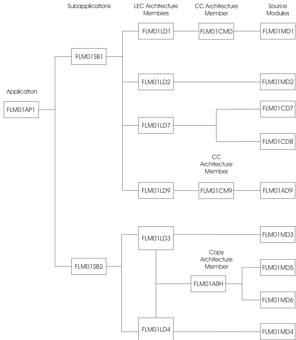
Figure 21. Example Project Architecture
