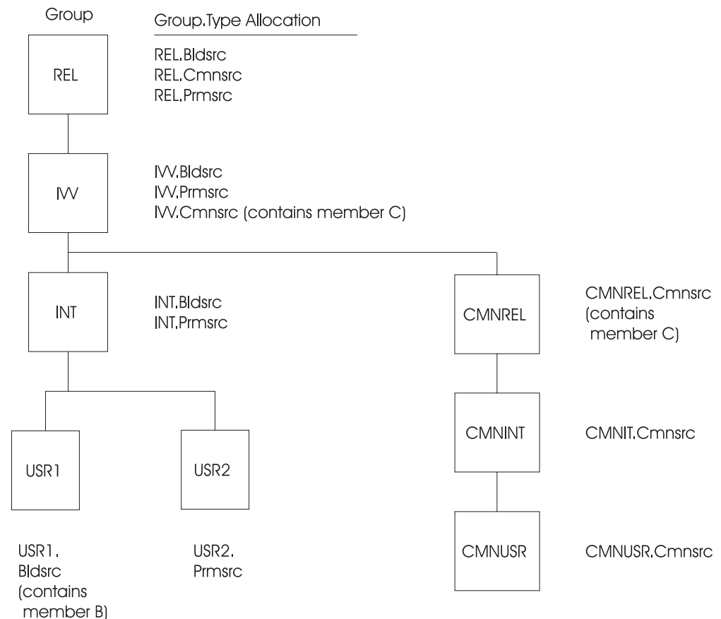
Figure 7. Valid Hierarchy with Unallocated Data Sets
