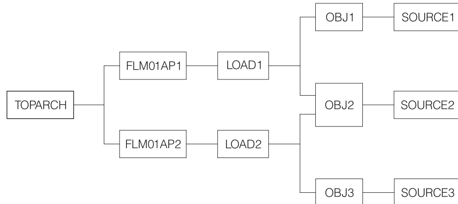
Figure 151. Example of Synchronization
