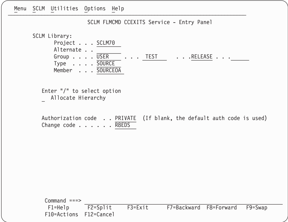
Figure 191. ISPF Interface Panel
