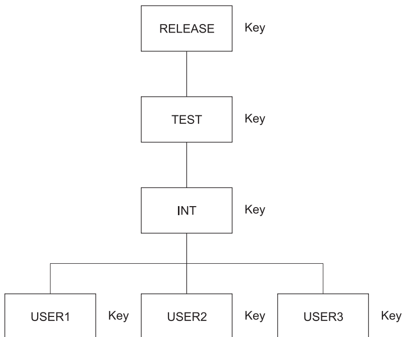
Figure 4. Default (Primary) Project Hierarchy Structure
