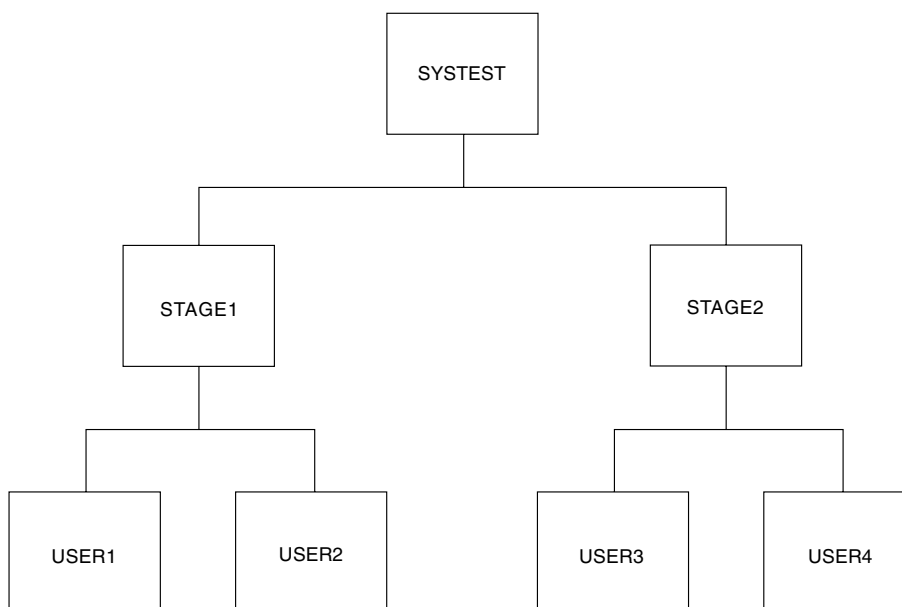
Figure 3. Example of SCLM Hierarchies
