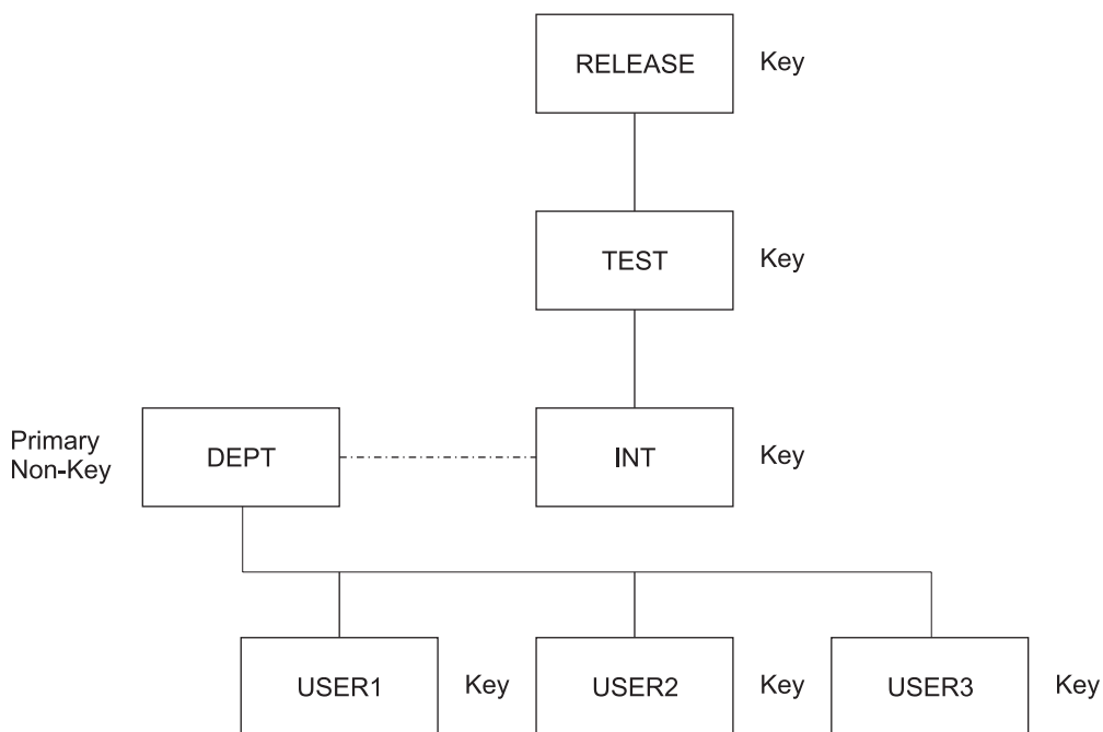
Figure 5. Alternate Project Hierarchy Structure with Primary Non-key Integration Group
