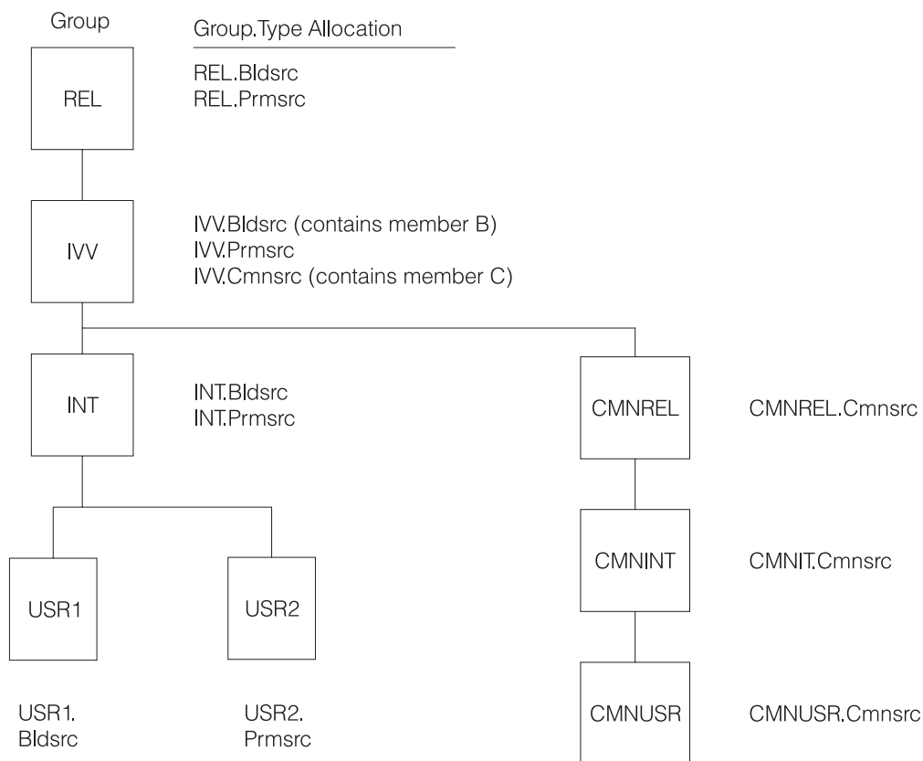
Figure 8. Invalid Hierarchy for Intended Operation
