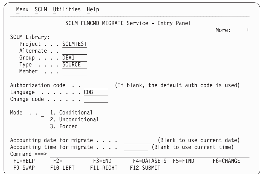
Figure 201. MIGRATE Service panel
