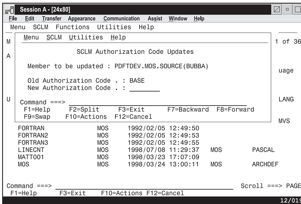
Figure 82. Authorization Code Update (FLMUSU#P)
