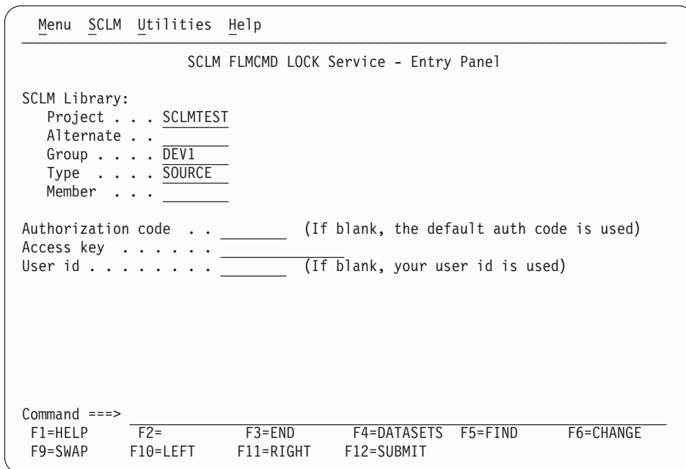
Figure 200. LOCK Service panel
