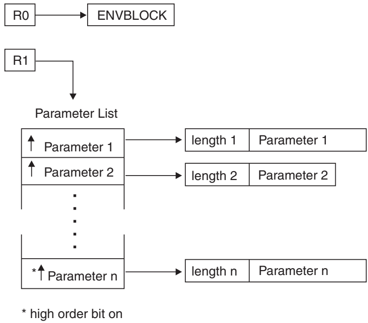
Figure 5. Parameters for LINKMVS and ATTCHMVS environments
