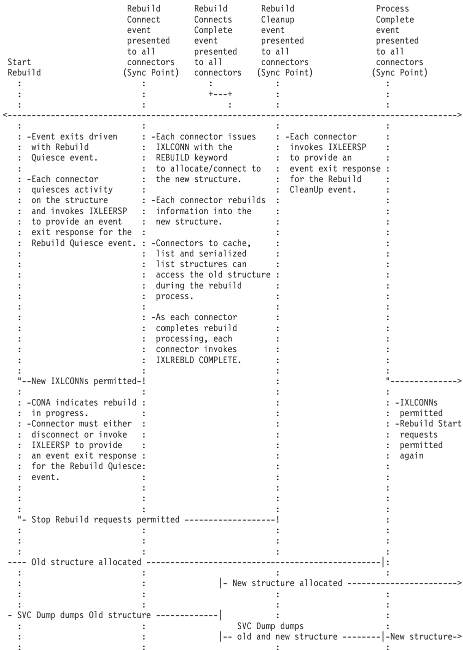
Figure 27. Rebuild Timeline
