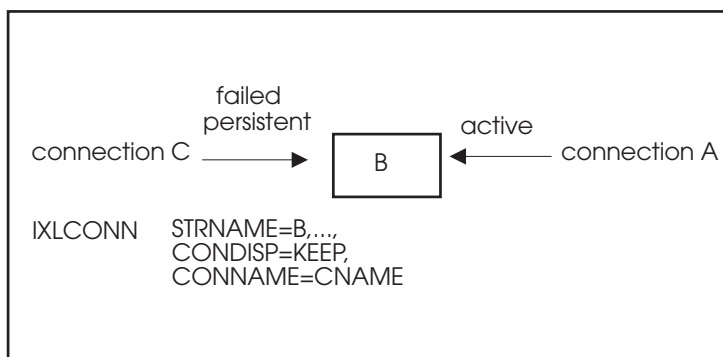
Figure 22. Active Connections
