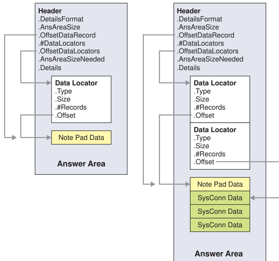
Figure 84. Answer areas for query note pad
