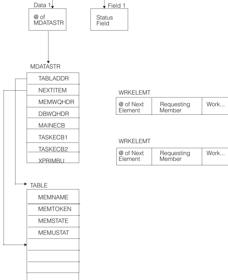
Figure 15. Data Structures Used by PHONBOOK Routine
