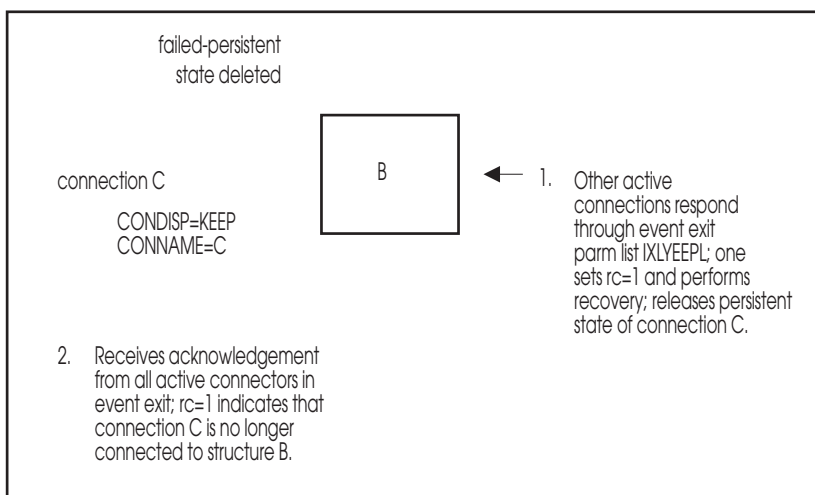
Figure 26. Deleting a Failed-Persistent Connection using IXLYEEPL
