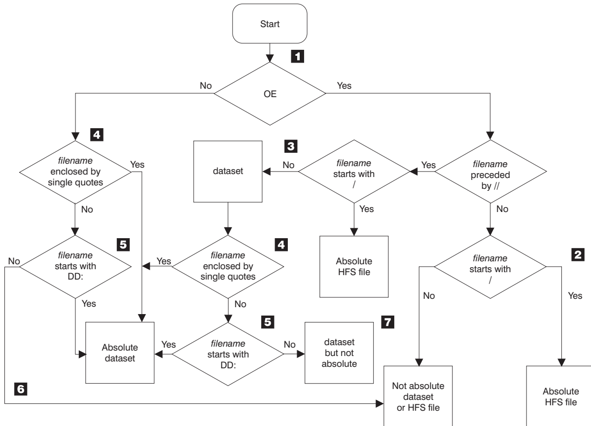
Figure 22. Testing if filename is in absolute form
