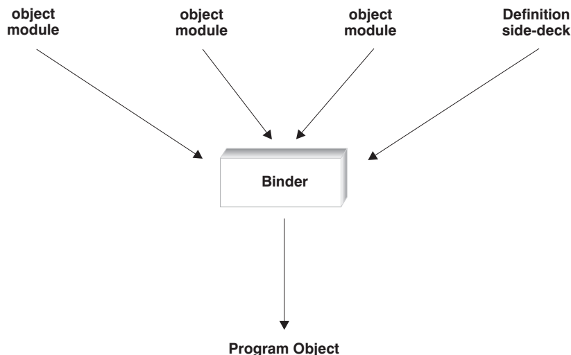
Figure 31. Build an application that uses a DLL
