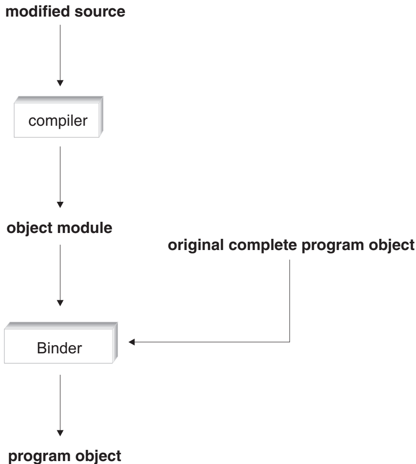
Figure 32. Rebinding a changed compile unit
