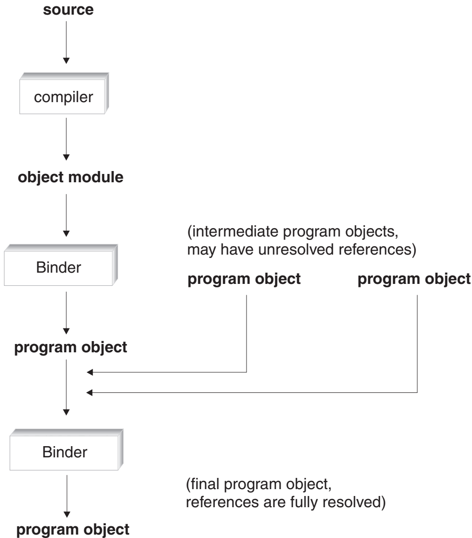
Figure 29. Bind each compile unit
