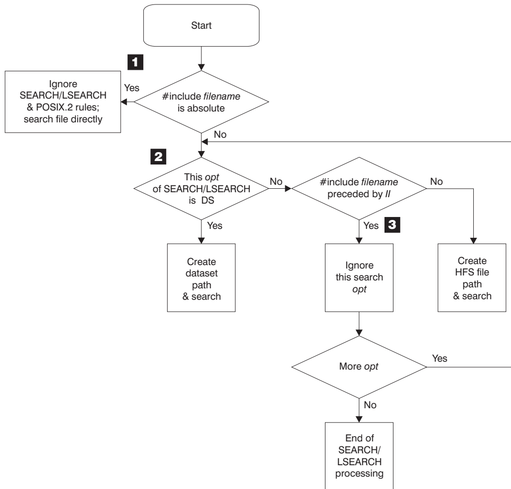
Figure 21. Overview of include file searching
