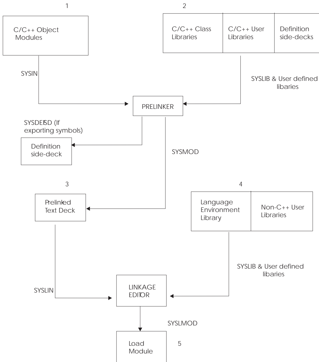
Figure 48. Basic prelinker and linkage editor processing
