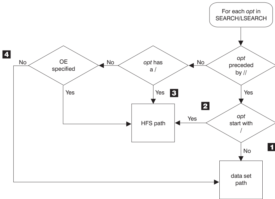
Figure 23. Determining if the SEARCH/LSEARCH opt is a z/OS UNIX path
