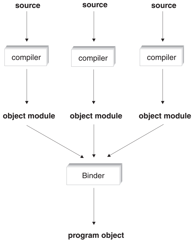
Figure 28. Single final bind
