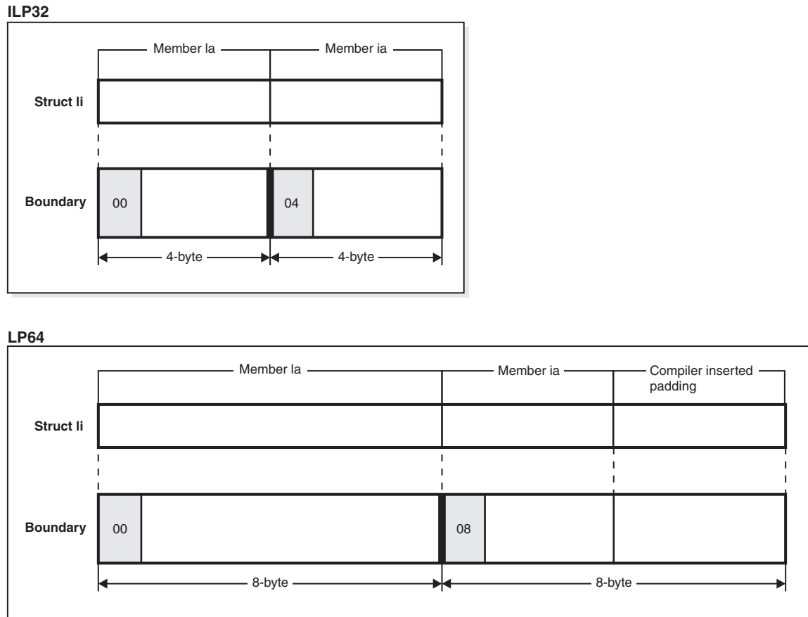
Figure 94. Comparison of struct li, alignments under ILP32 and LP64
