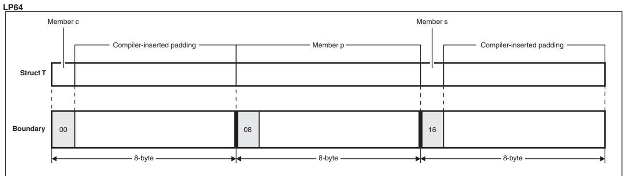
Figure 97. Example of potential alignment problems when a struct is shared or exchanged among 32-bit and 64-bit processes.
