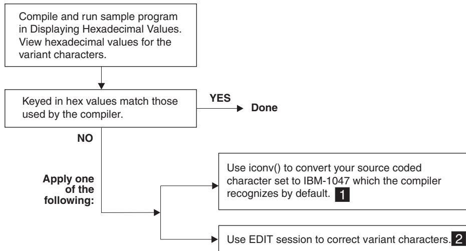
Figure 271. Variant characters
