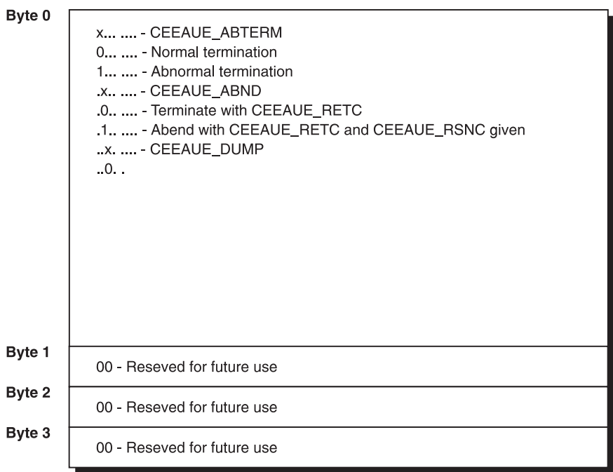
Figure 194. CEEAUE_FLAGS format
