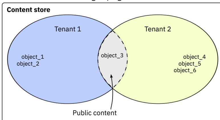
Figure 12. Content store configured to use the Cognos Analytics multitenancy capabilities
