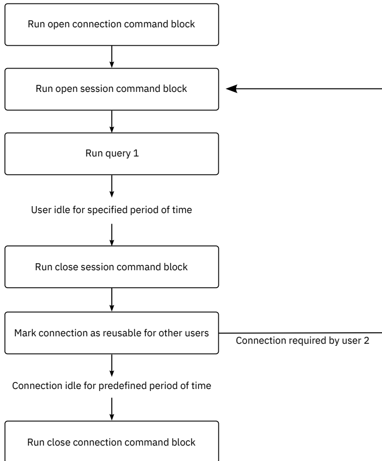
Figure 2. Example of interaction between command blocks
