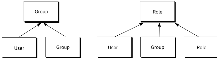
Figure 6. Structure of groups and roles
