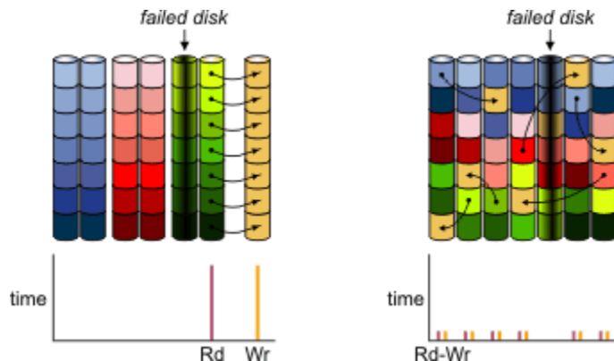
Figure 3. Lower rebuild overhead in declustered RAID versus conventional RAID
