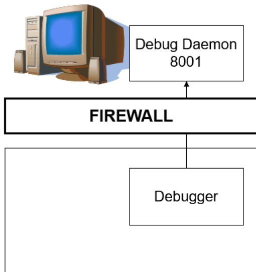
Figure 7. TCP/IP port for the usage of z/OS Debugger without Debug Manager
