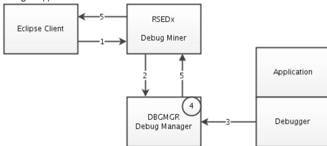
Figure 2. Debug Manager
