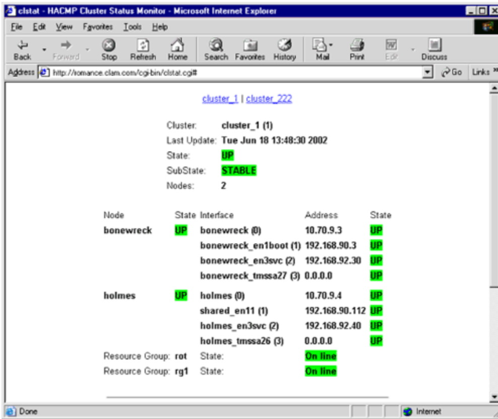
Figure 3. clstat web browser display
