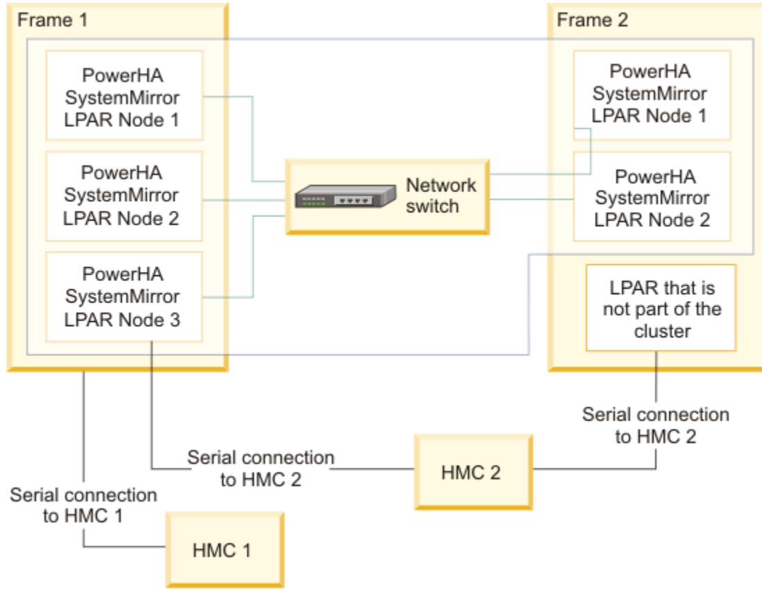
Figure 11. PowerHA SystemMirror cluster configuration with LPARs
