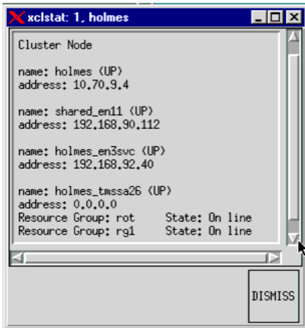
Figure 2. clstat node information display
