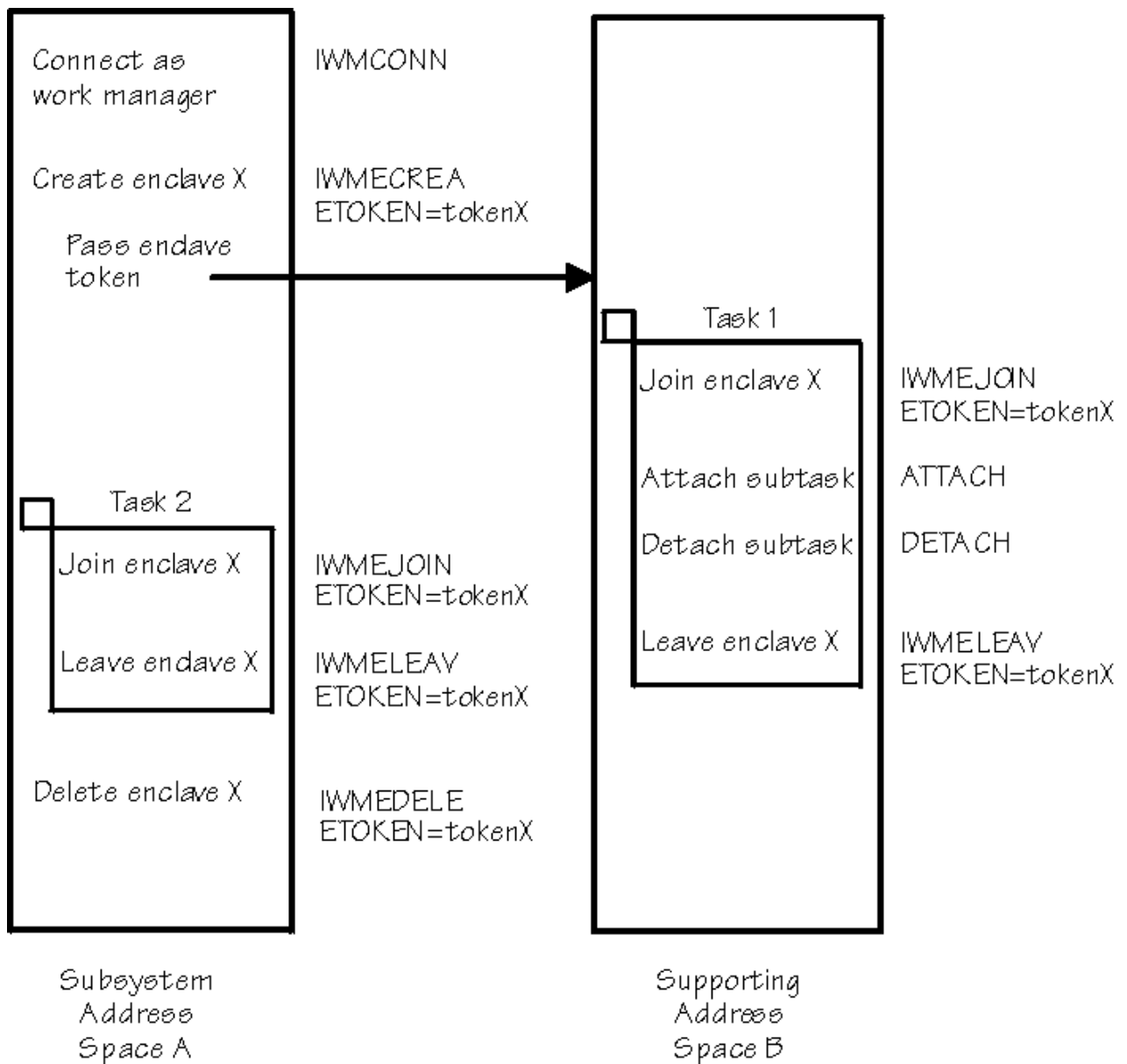
Figure 8. Creating an enclave and joining tasks to it
