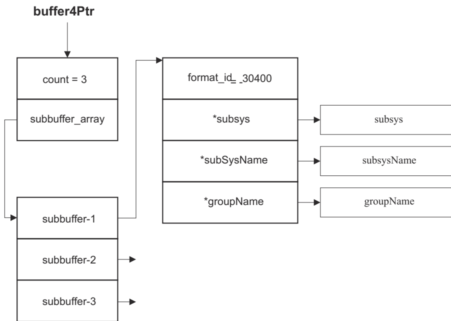
Figure 13. Sub-buffer arm_subbuffer_zos_connect_t)
