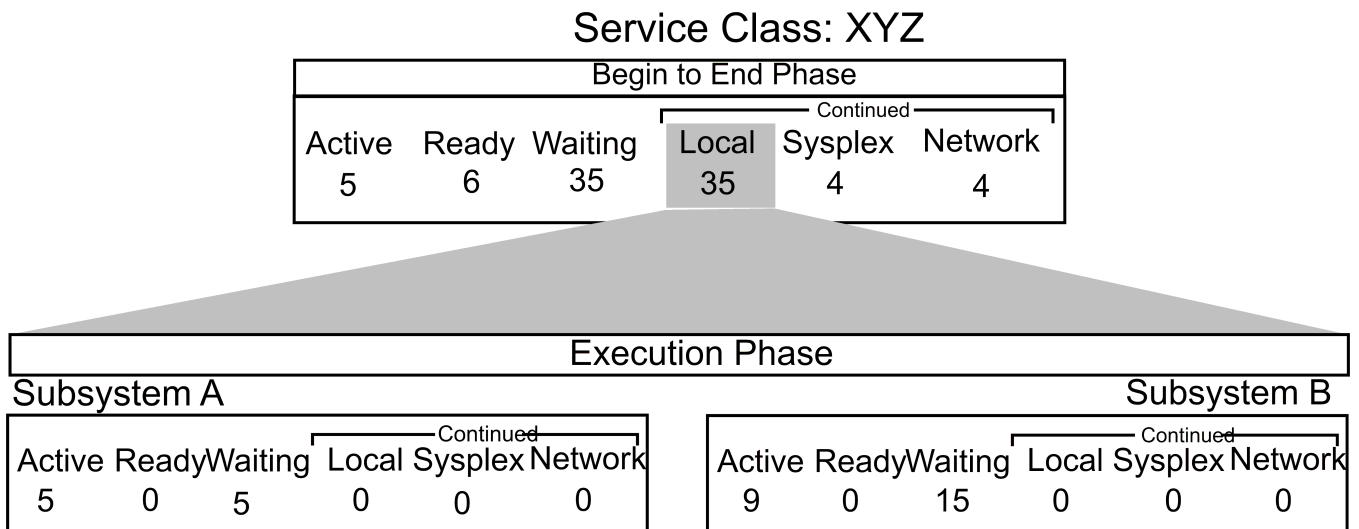
Figure 27. Combining state information across subsystems
