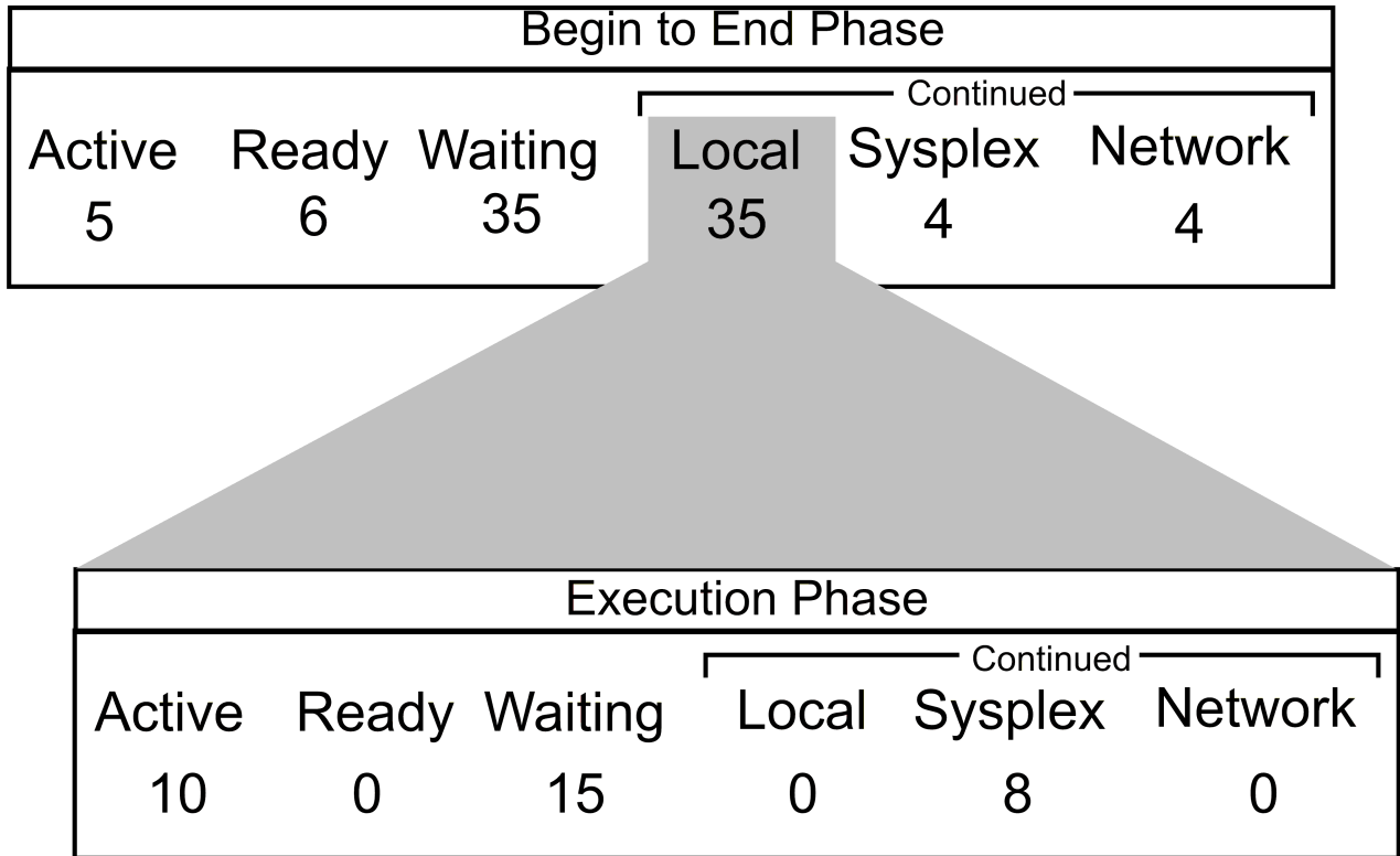
Figure 26. Combining state information for a service class
