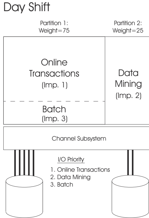
Figure 28. Intelligent Resource Director example – Day shift
