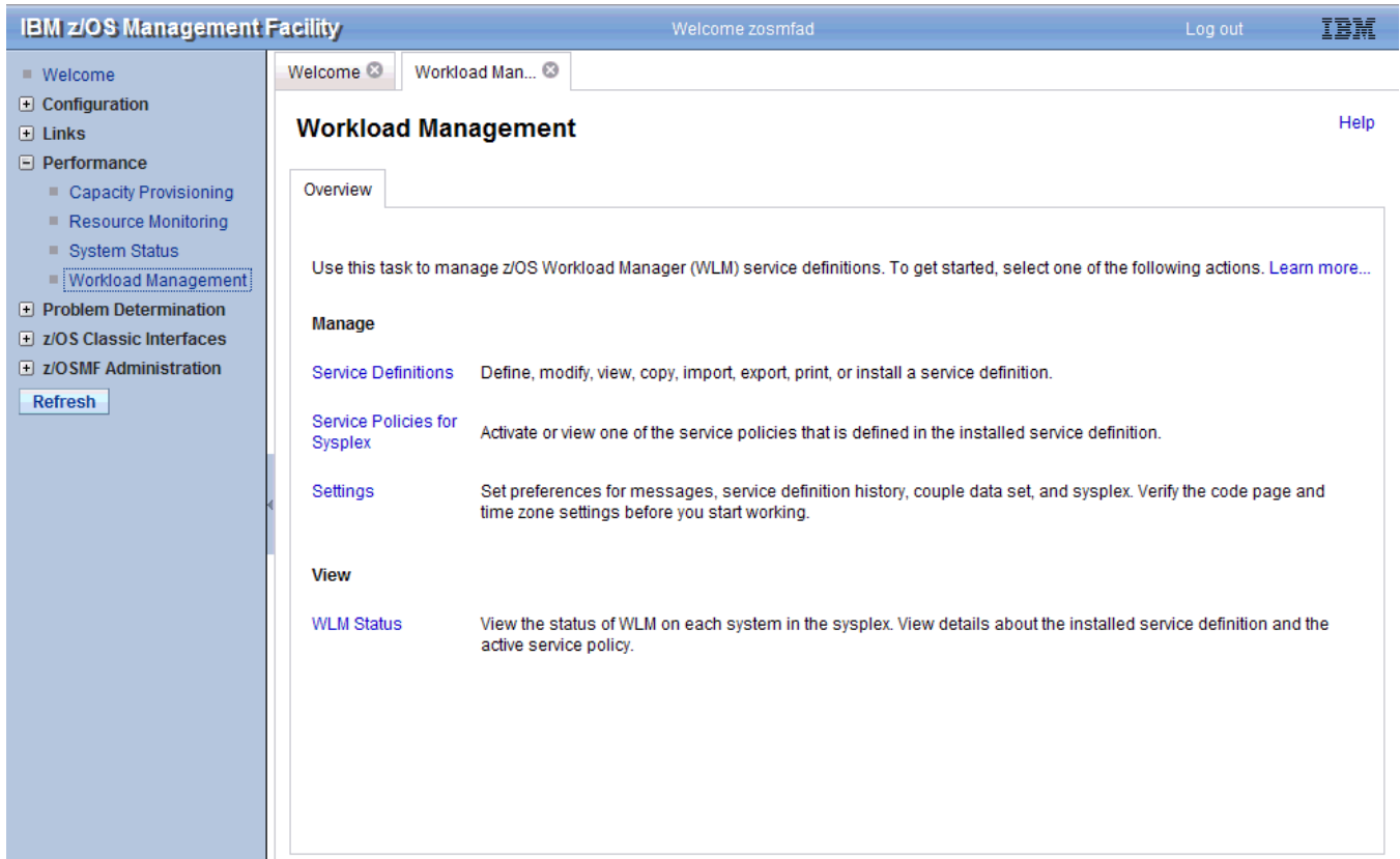
Figure 90. z/OS Management Facility - Overview Panel
