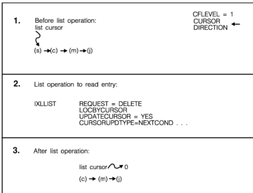
Figure 60. List Cursor When Moved Conditionally Before First Entry
