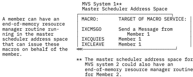
Figure 3. Address Space Restrictions for XCF Macros
