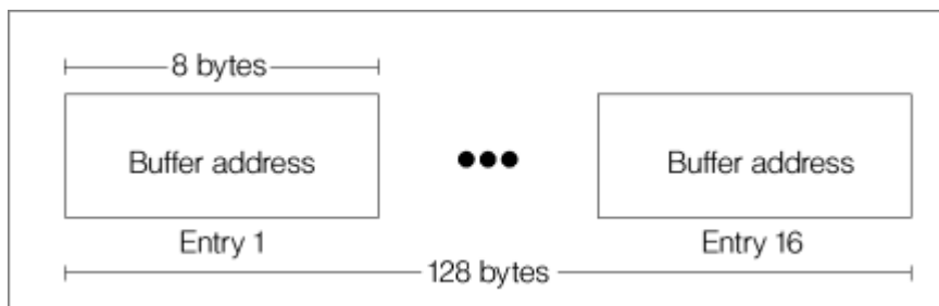
Figure 63. Format of Buffer List - 64-bit Addresses
