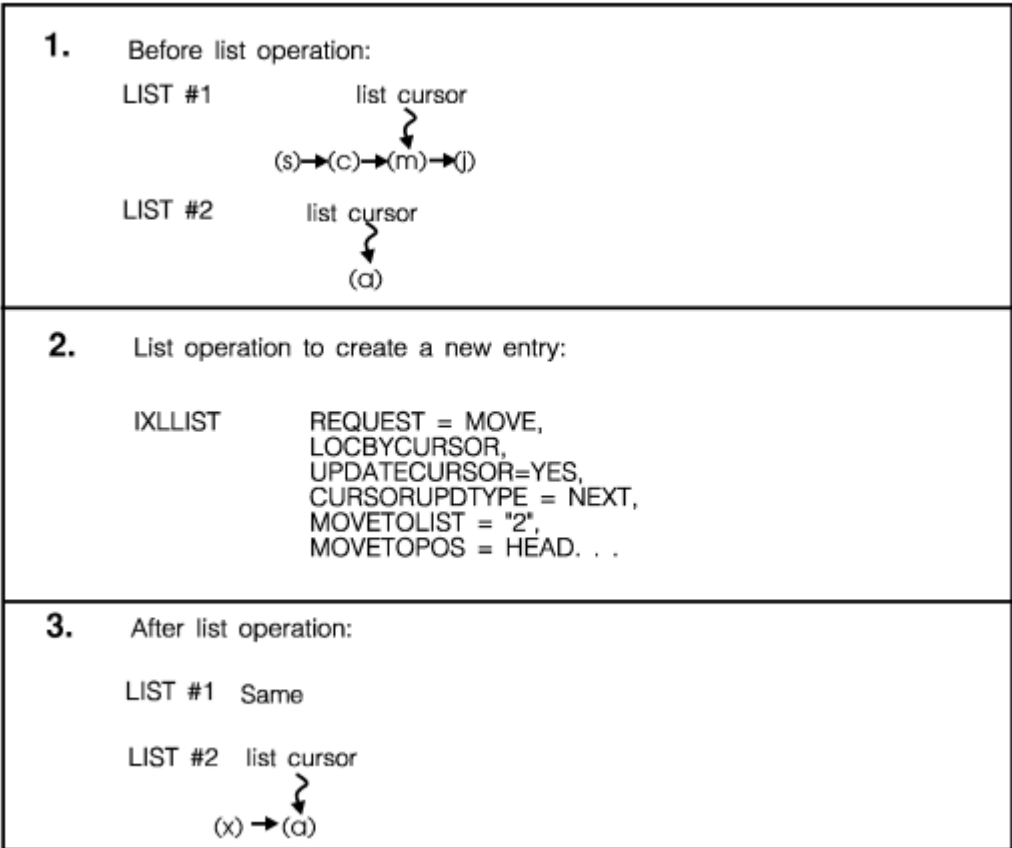
Figure 56. Updating the List Cursor when Creating an Entry with MOVE
