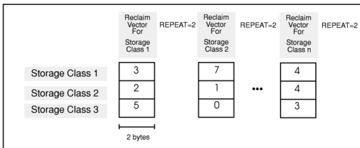
Figure 37. Three Reclaim Vectors
