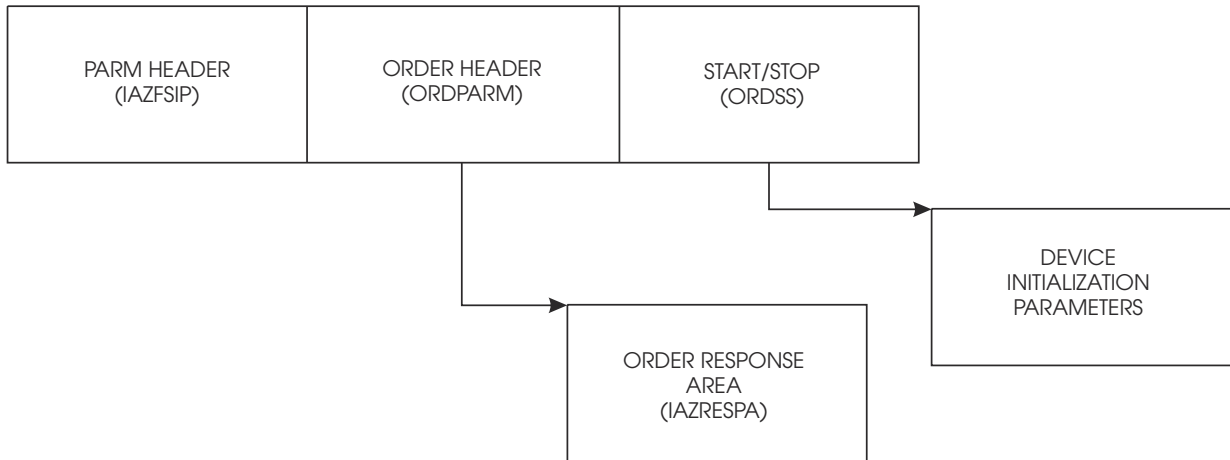
Figure 13. FSIREQ parameter lists for the START FSA order
