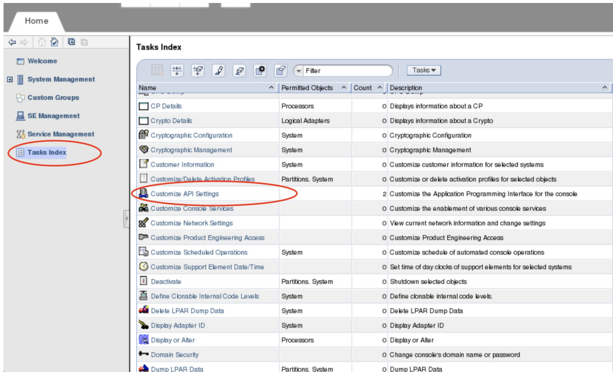
Figure 22. Tasks index
