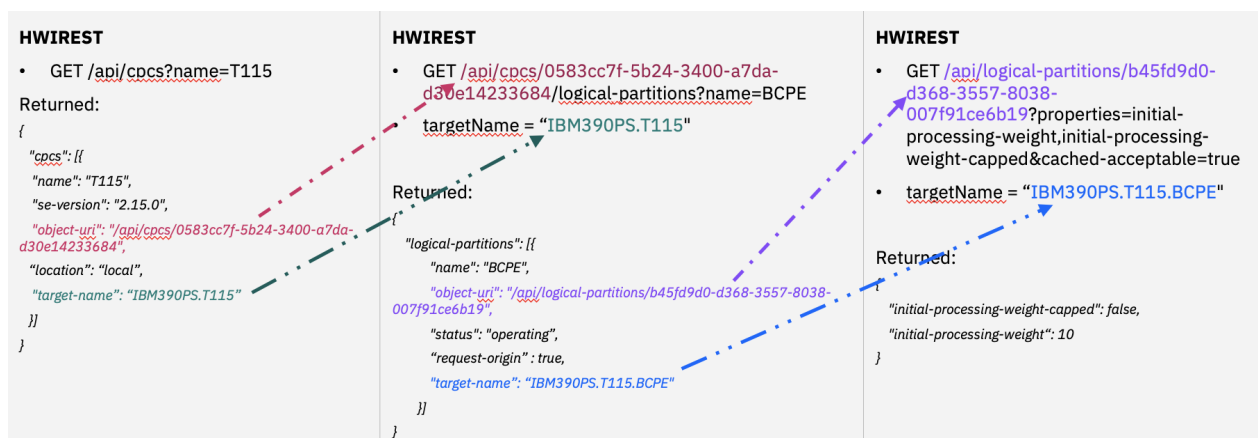
Figure 24. Retrieve LPAR GPP weight
