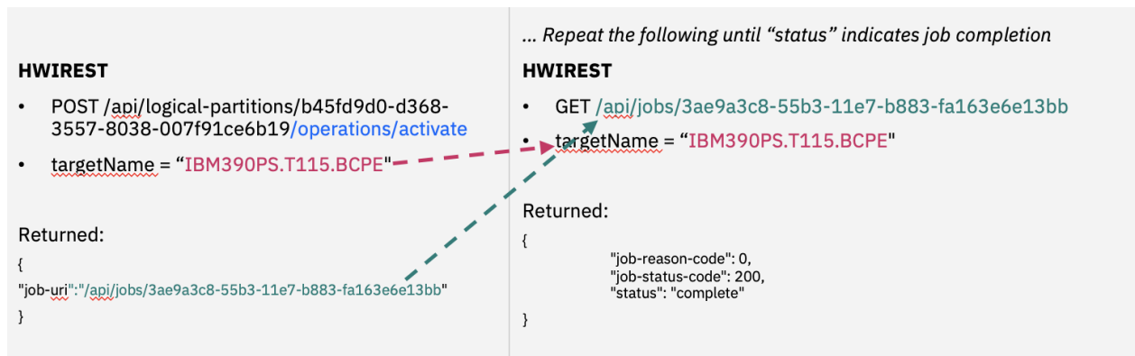
Figure 25. POLLing result of an asynchronous operation
