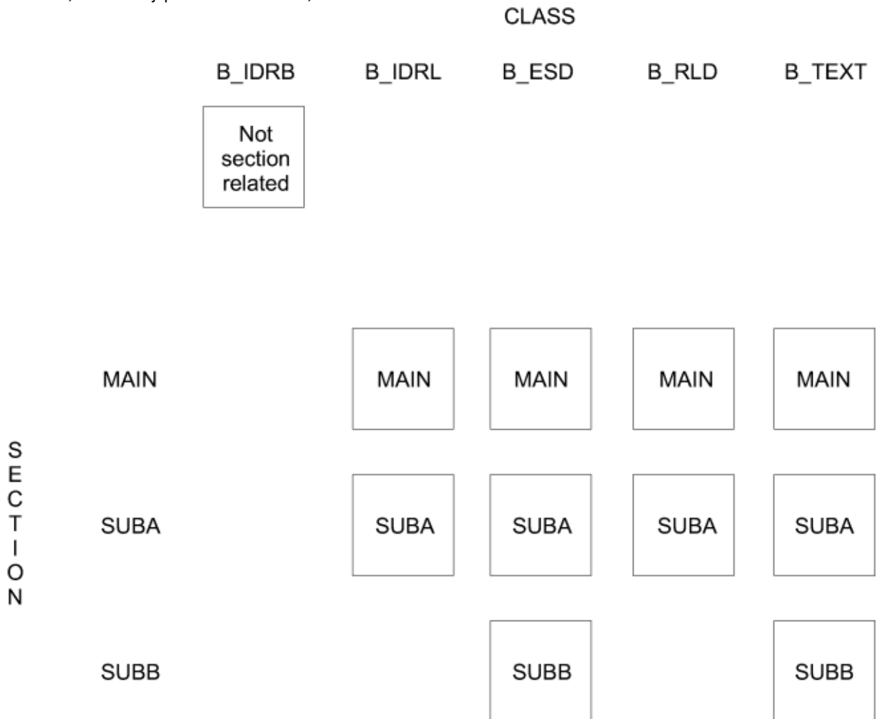
Figure 1. Data items
