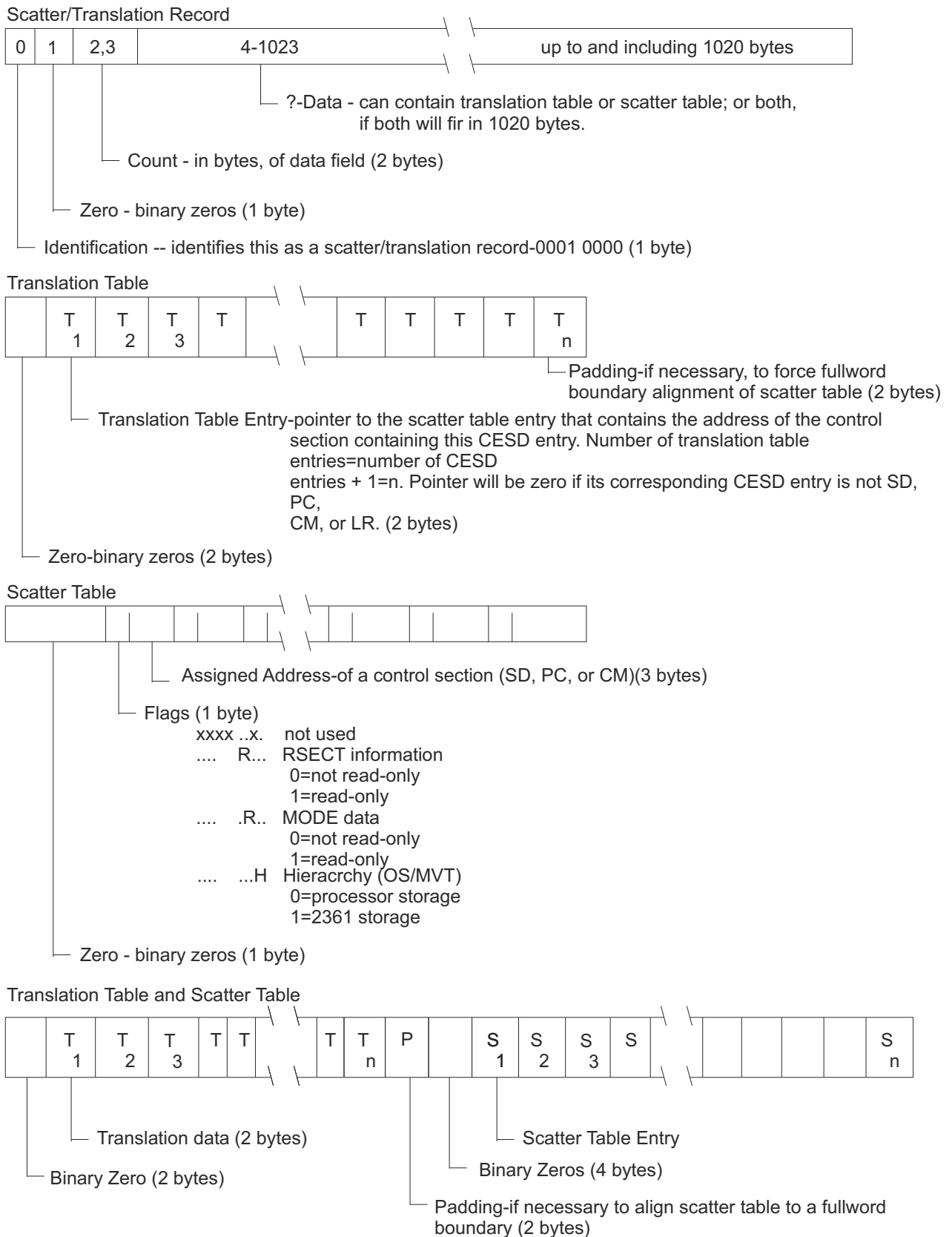
Figure 14. Scatter/Translation record
