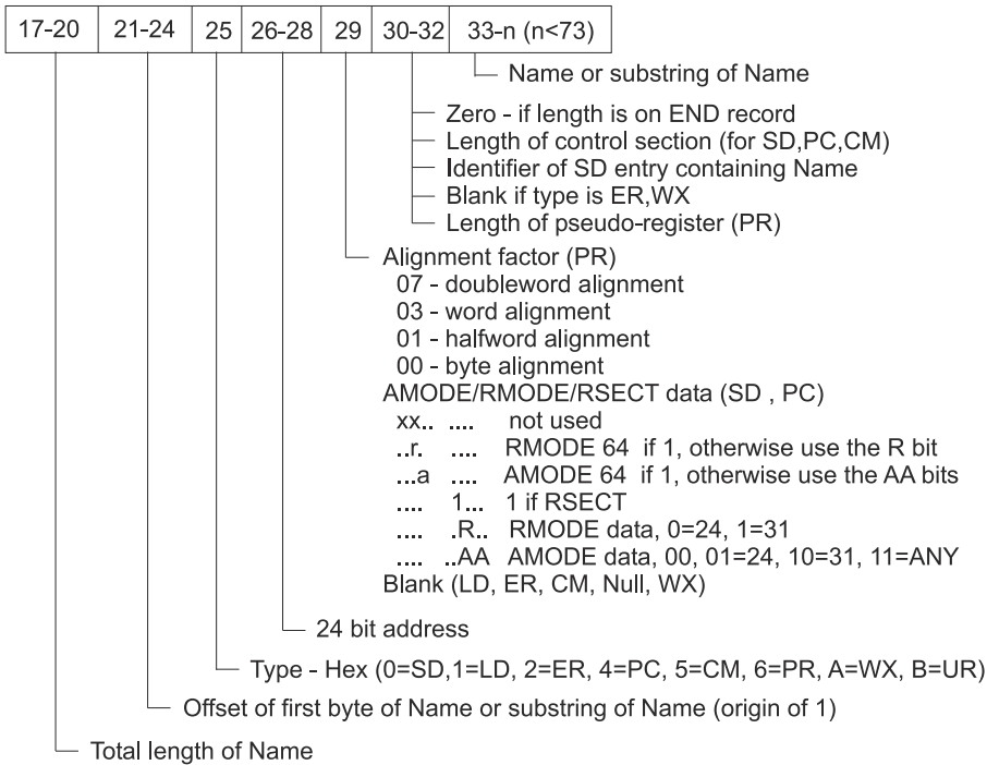
XSD Data
