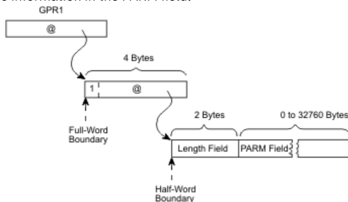
Figure 6. Primary Mode Parameter List EXEC PGM=
