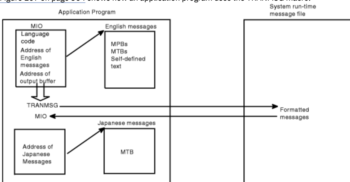
Figure 107. Using the TRANMSG Macro
