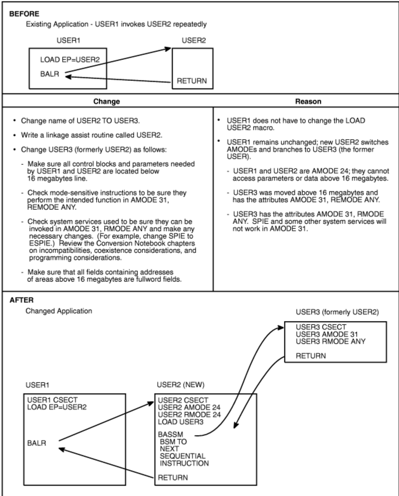
Figure 41. Example of a Linkage Assist Routine
