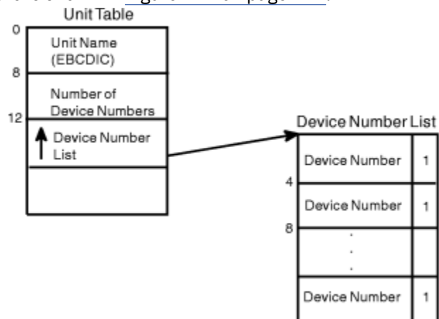
Figure 121. Requesting function code 1 (check units)
