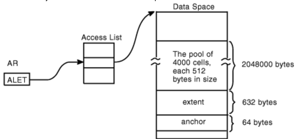
Figure 72. Example of Using Callable Cell Pool Services for Data Spaces
