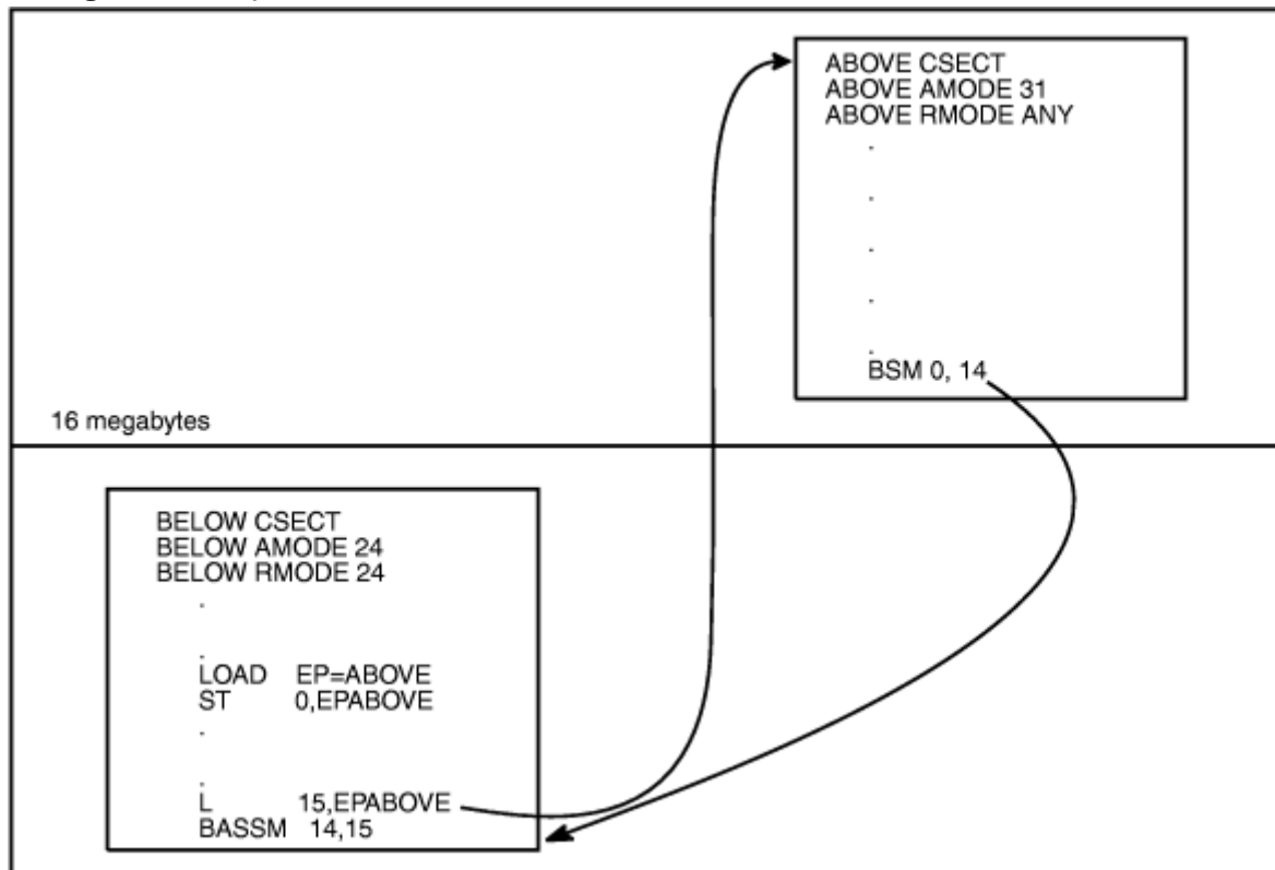
Figure 38. Using BASSM and BSM
