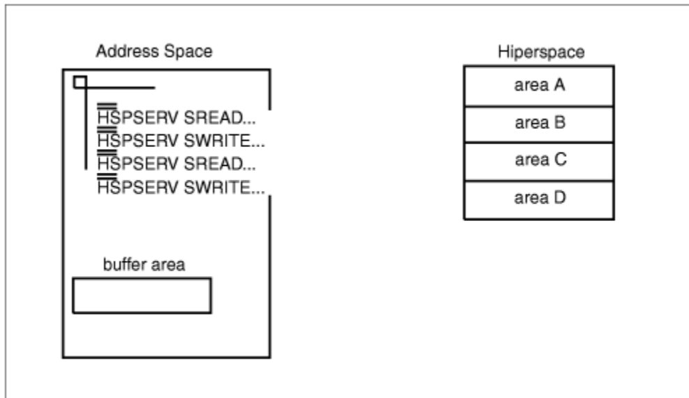
Figure 74. Example of Scrolling through a Standard Hiperspace
