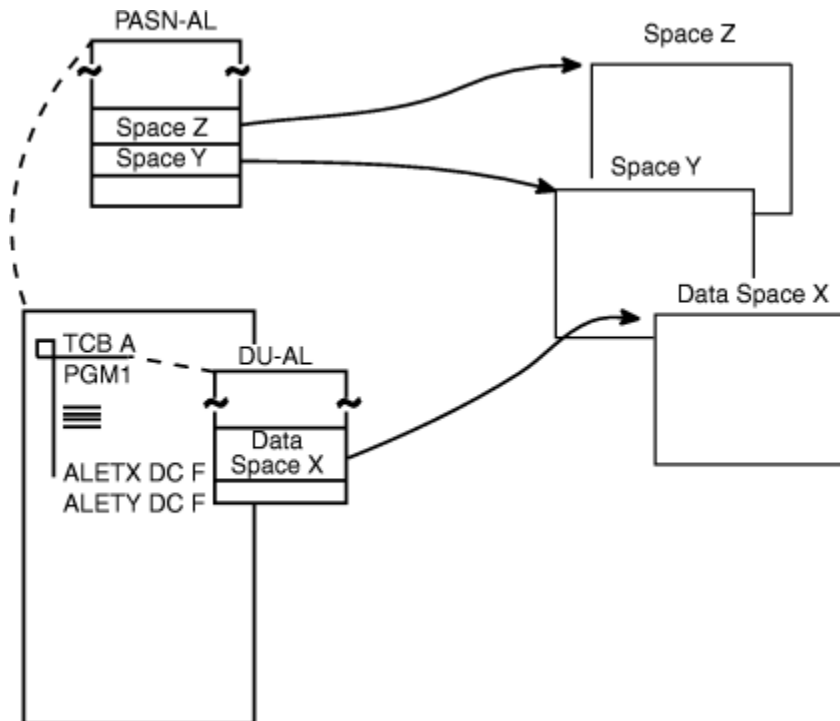
Figure 66. An Illustration of a DU-AL
