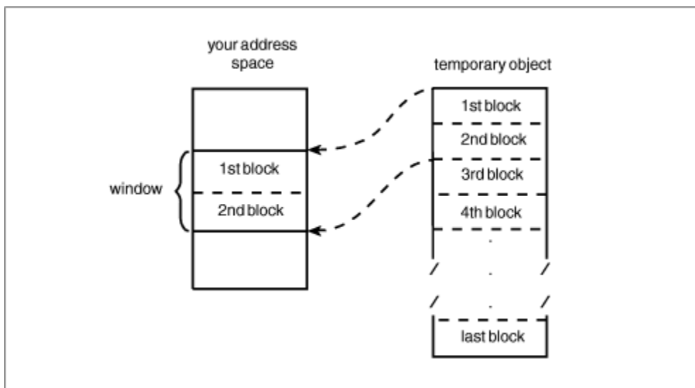
Figure 82. Mapping a Temporary Object
