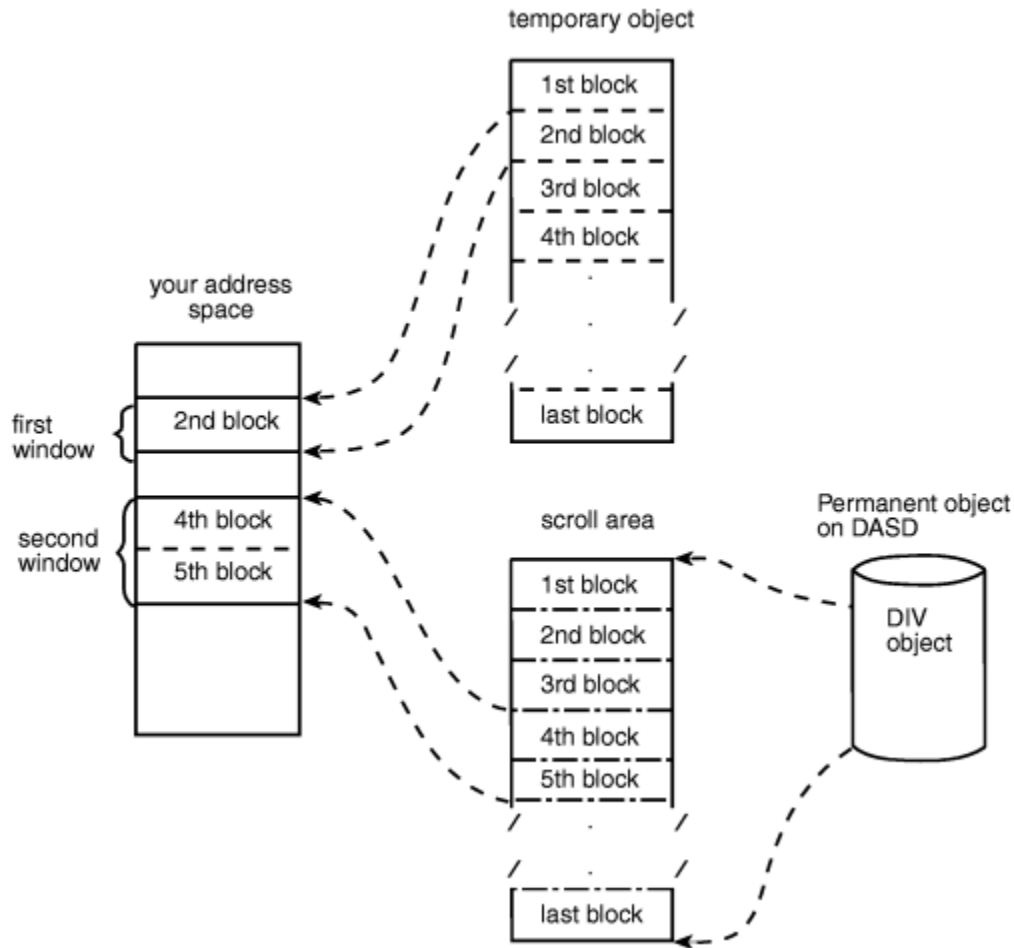
Figure 84. Mapping Multiple Objects
