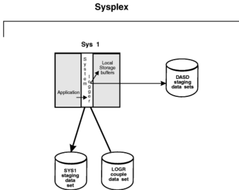
Figure 114. A DASD-Only Configuration
