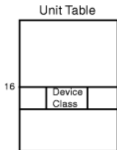
Figure 135. Requesting Function Code 11 (Return Unit Names for a Device Class)
