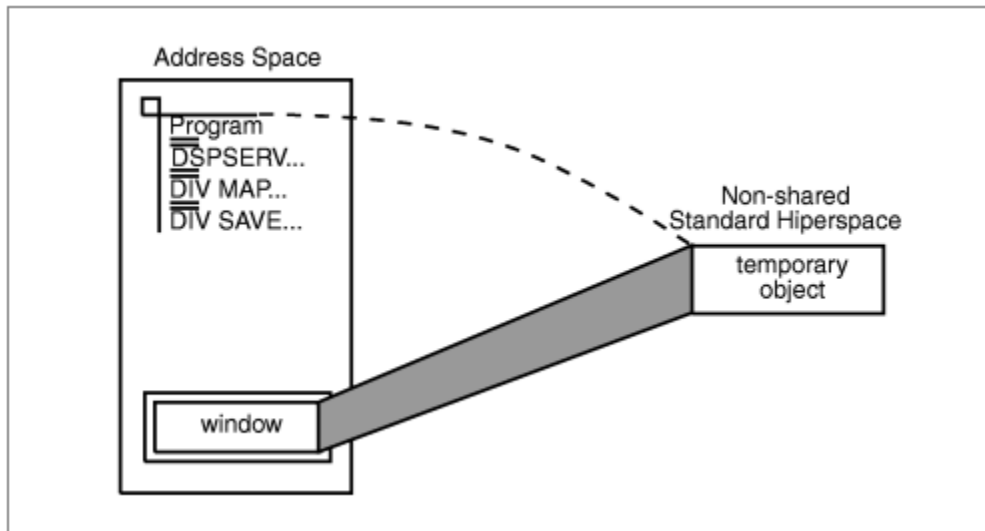
Figure 78. A Standard Hiperspace as a Data-in-Virtual Object
