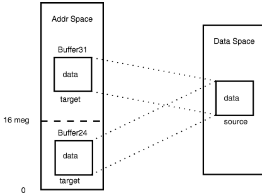
Figure 95. Sharing Storage with IARVSERV
