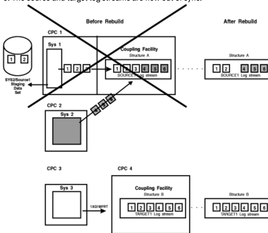
Figure 118. How Source and Target Log Streams Can Get Out of Sync
