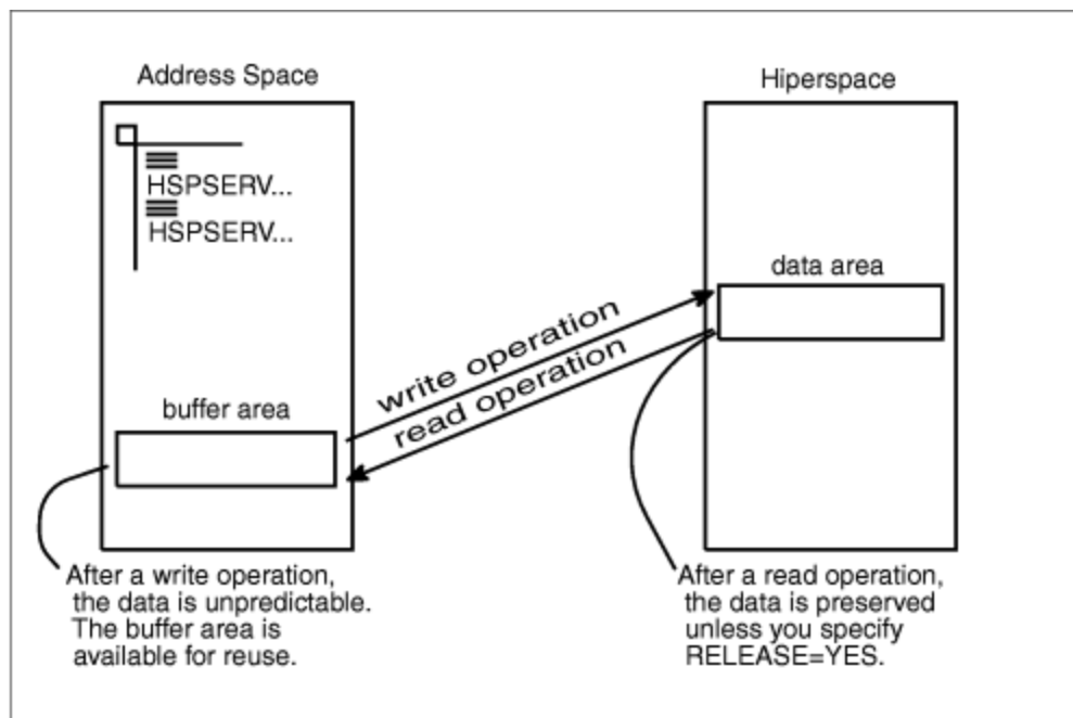
Figure 75. Illustration of the HSPSERV Write and Read Operations
