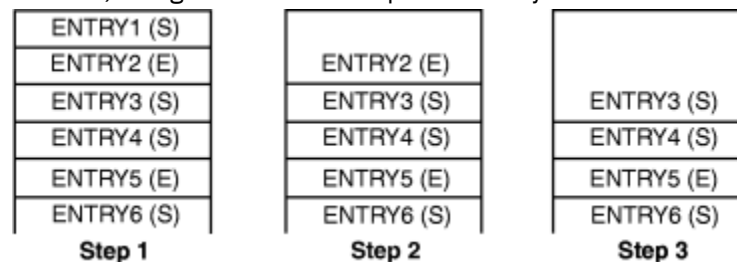
Figure 49. ISGENQ Macro Processing
