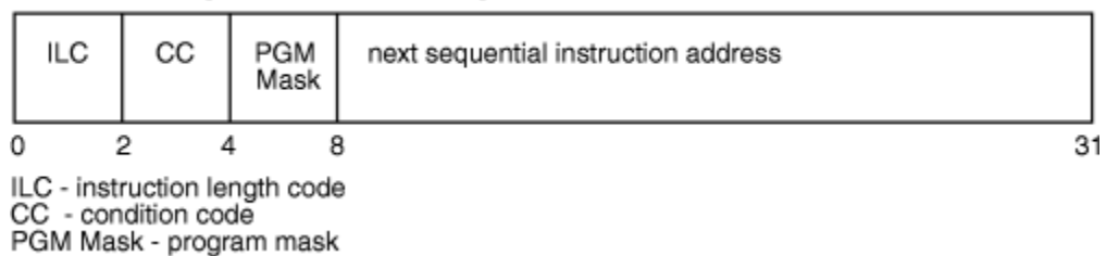
First operand register (24-bit addressing mode)
