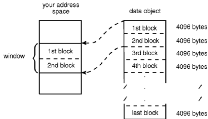
Figure 79. Structure of a Data Object
