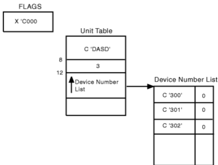
Figure 137. Input for Function Codes 0 and 1
