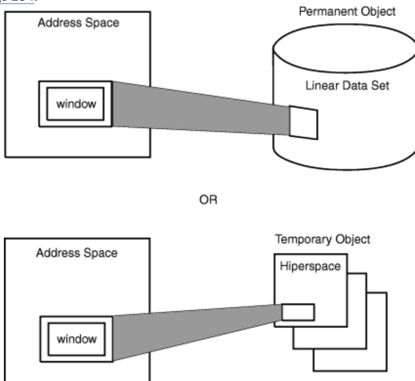
Figure 62. Mapping from an address space
