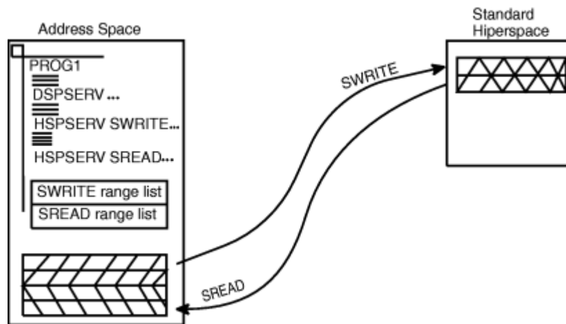
Figure 76. Example of Creating a Standard Hiperspace and Transferring Data
