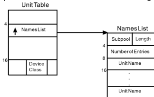
Figure 136. Output from Function Code 11 (Return Unit Names for a Device Class)
