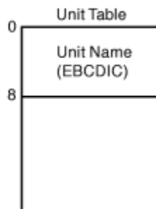
Figure 123. Output from Function Code 2 (Return Unit Name)
