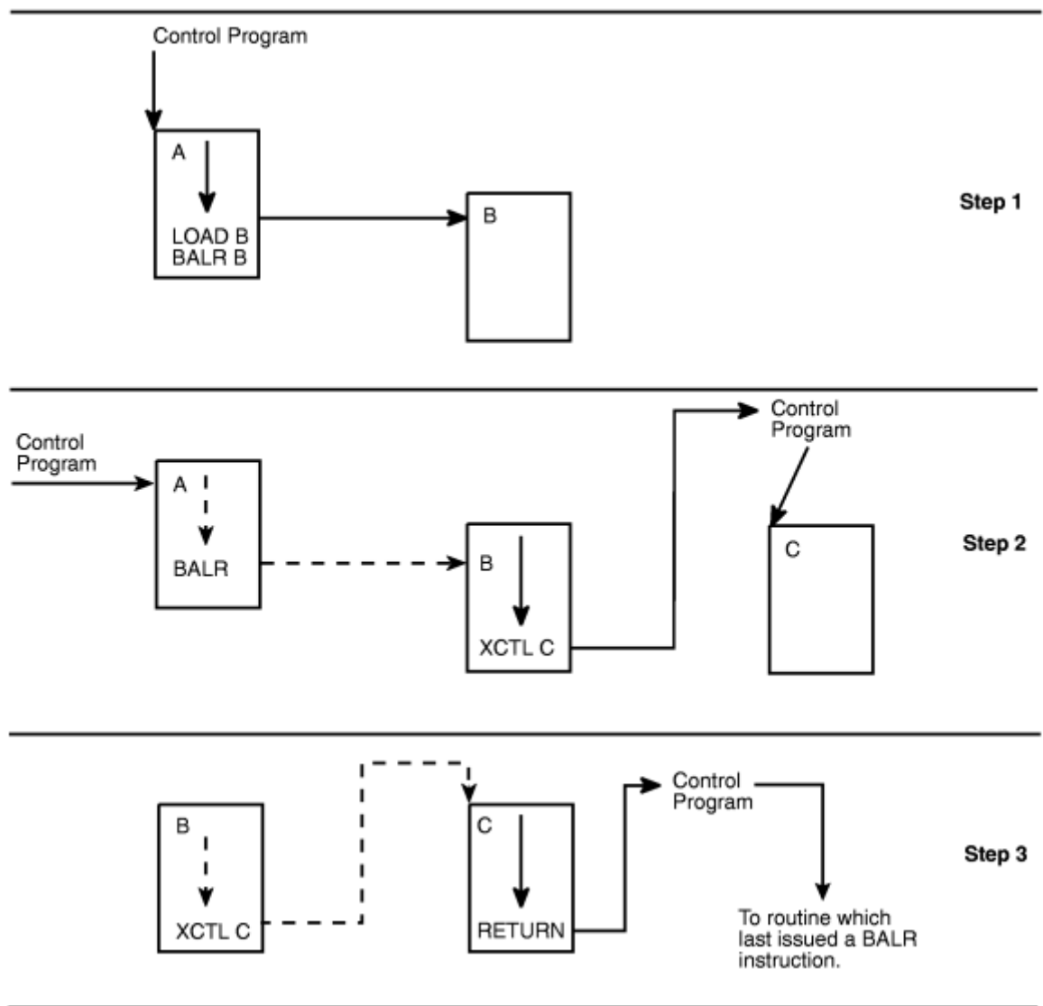
Figure 27. Misusing Control Program Facilities Causes Unpredictable Results
