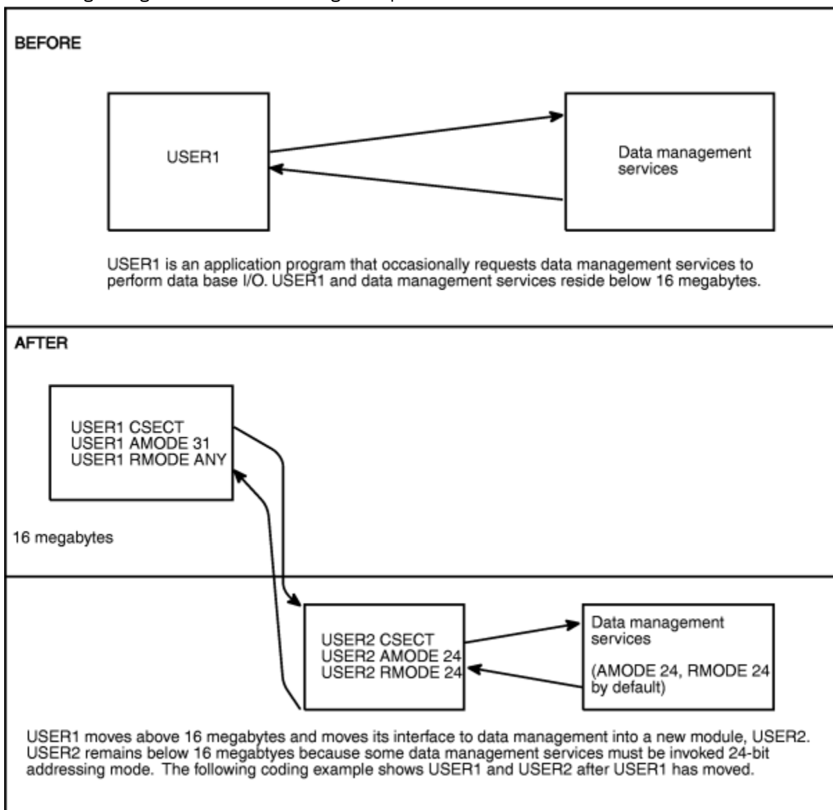
Figure 43. Performing I/O while residing above 16 megabytes
