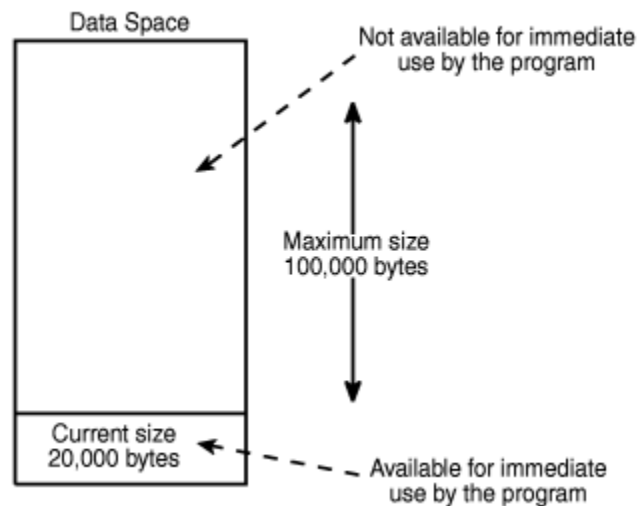
Figure 70. Example of Specifying the Size of a Data Space
