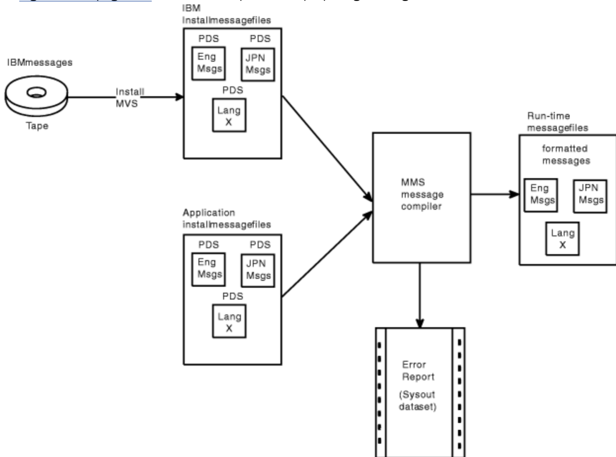
Figure 99. Preparing Messages for Translation
