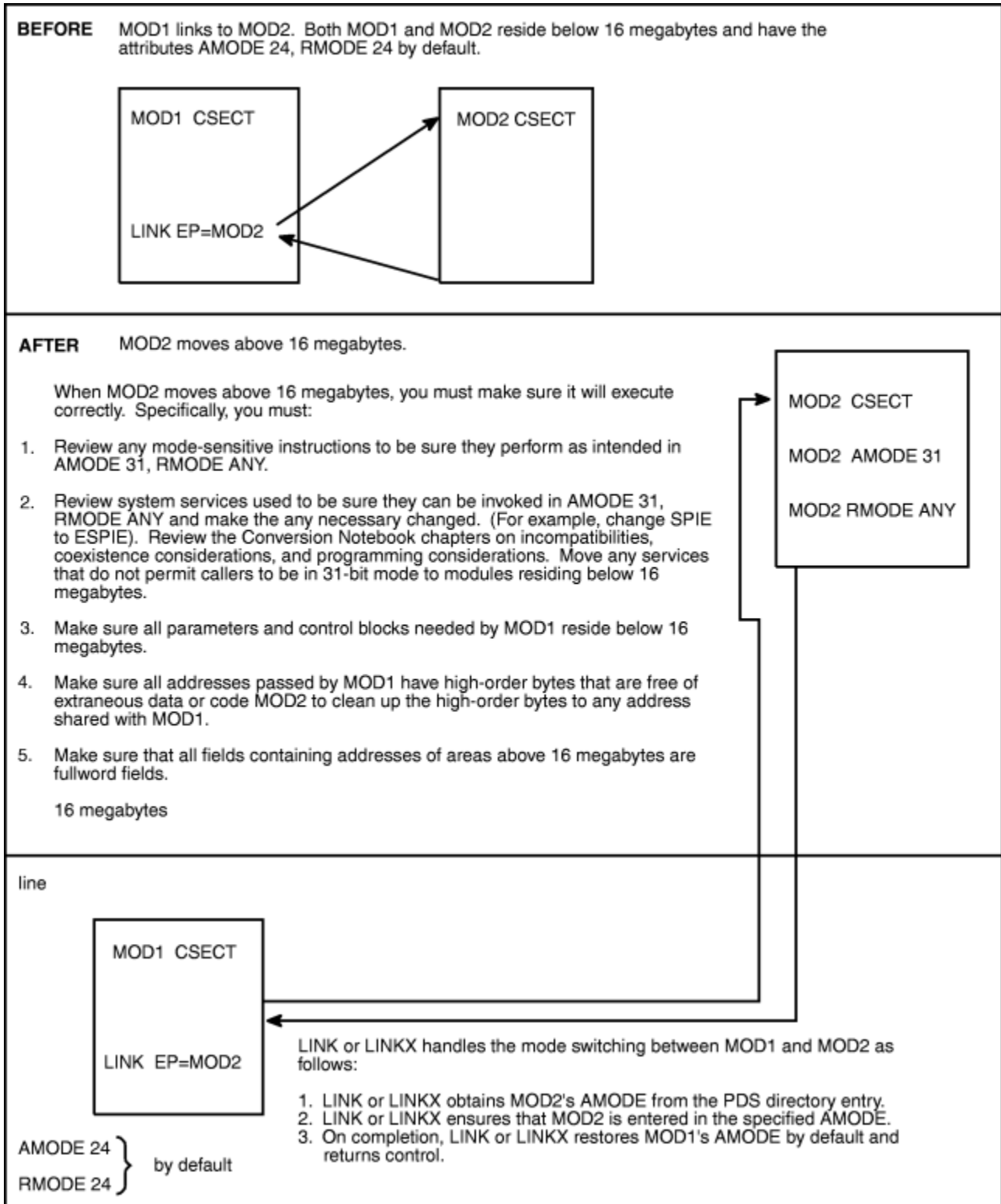
Figure 40. Example of Supervisor-Assisted Linkage
