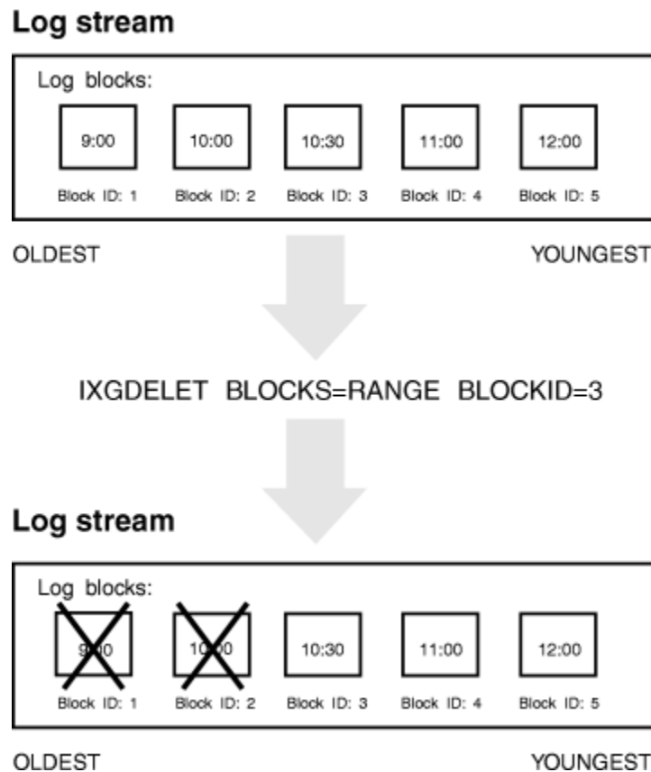
Figure 117. Deleting a Range of Log Blocks
