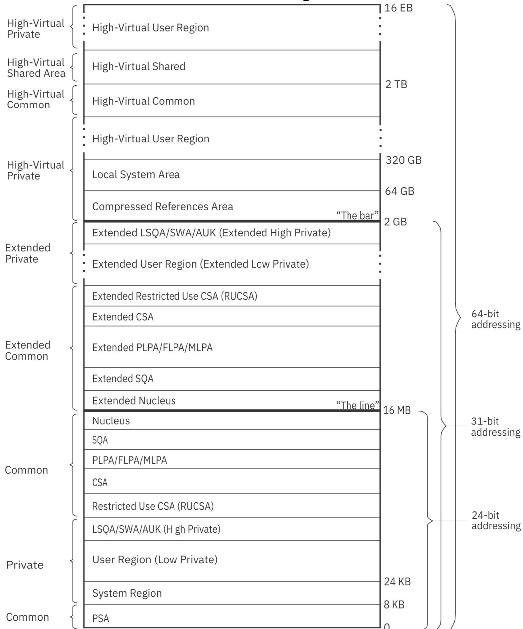
Figure 29. Virtual storage map (not drawn to scale)
