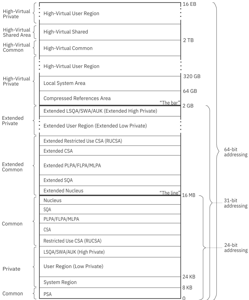
Figure 60. The 64-bit address space
