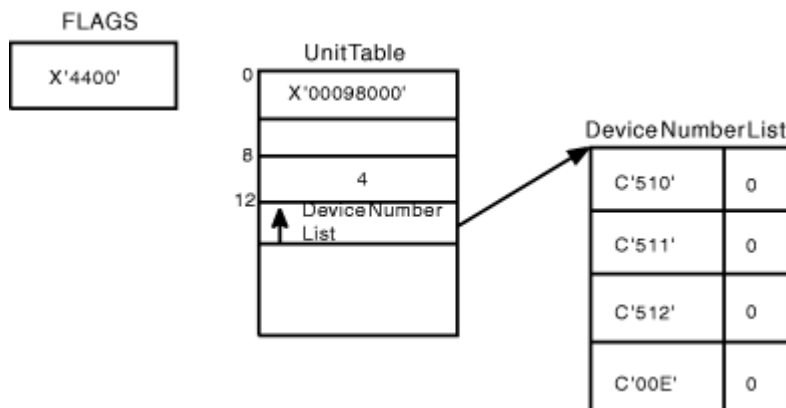
Figure 141. Input for Function Codes 1 and 5
