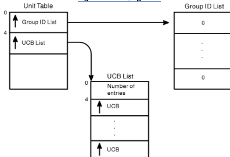
Figure 126. Requesting function code 4 (return group ID)
