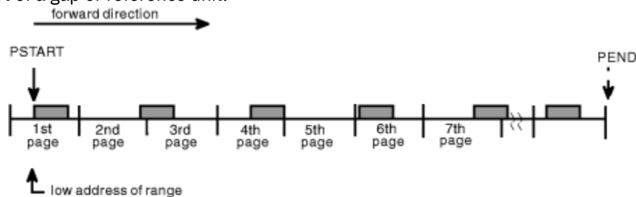
Figure 91. Illustration of Forward Direction in a Reference Pattern
