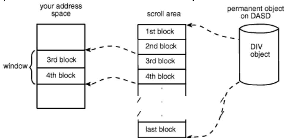
Figure 81. Mapping a Permanent Object That Has A Scroll Area
