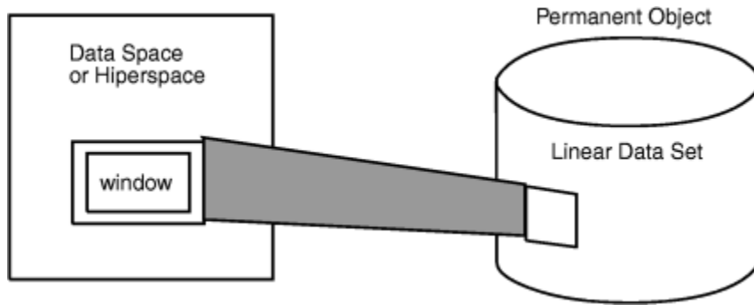
Figure 63. Mapping from a data space or hiperspace
