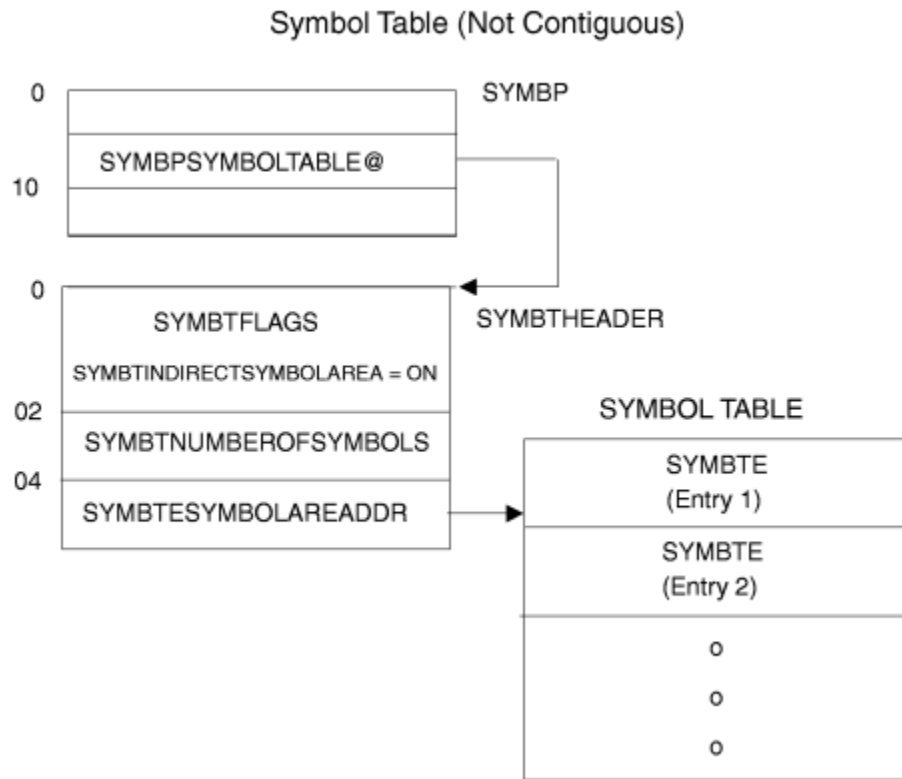
Figure 109. Non-contiguous Symbol Table
