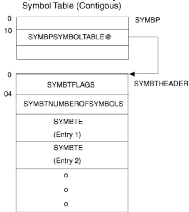
Figure 108. Contiguous Symbol Table
