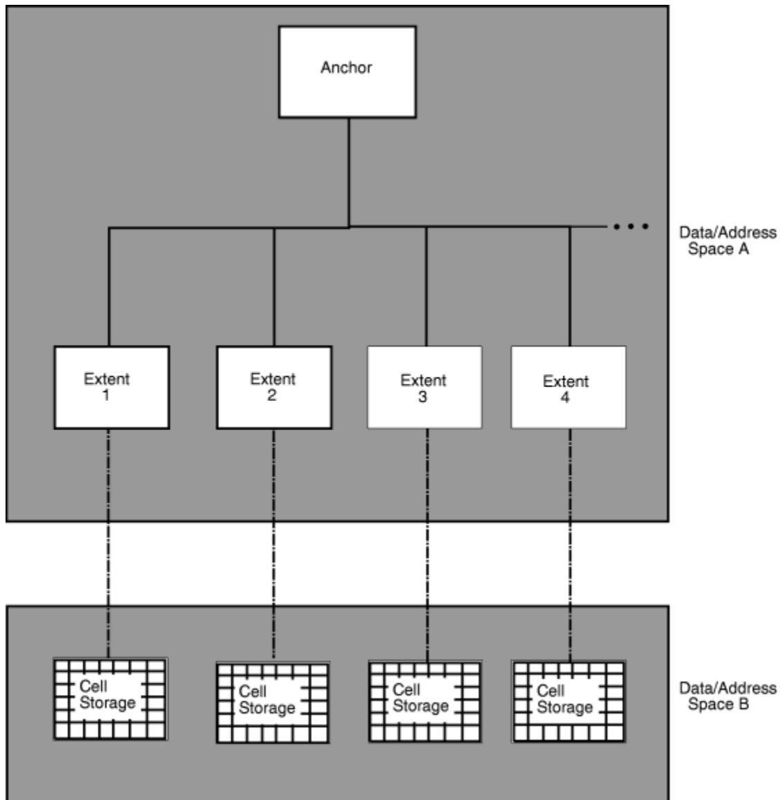
Figure 61. Cell pool storage
