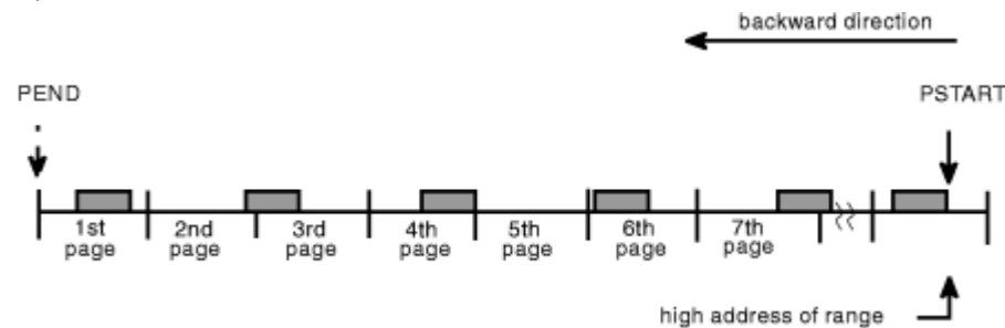
Figure 92. Illustration of Backward Direction in a Reference Pattern
