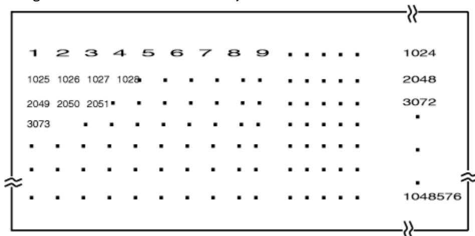
Figure 89. Example of using REFPAT with a Large Array
