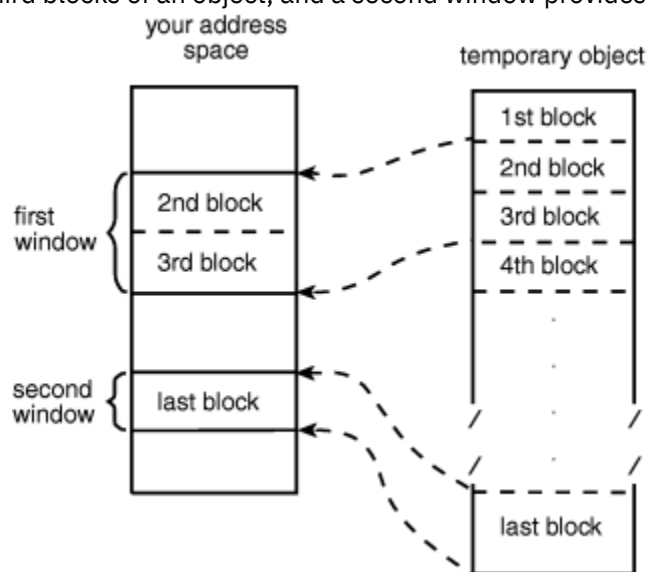
Figure 83. Mapping an Object To Multiple Windows
