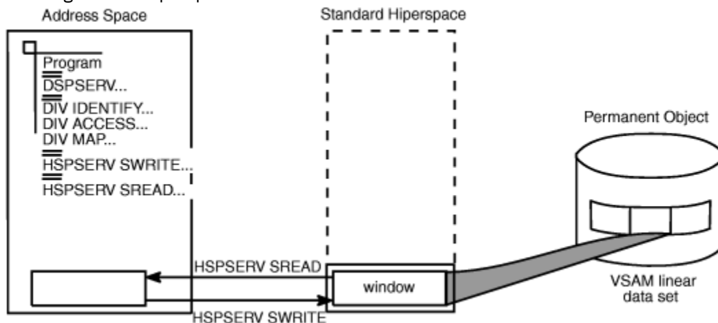
Figure 77. Example of Mapping a Data-in-Virtual Object to a Hiperspace
