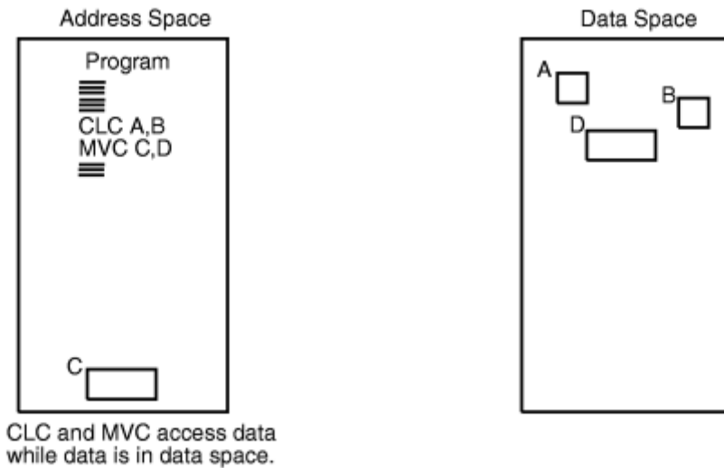
Figure 68. Accessing Data in a Data Space
