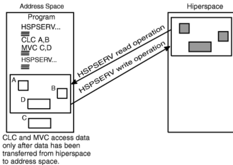
Figure 69. Accessing Data in a Hiperspace
