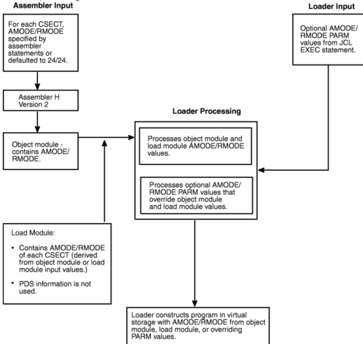
Figure 33. AMODE and RMODE Processing by the Loader
