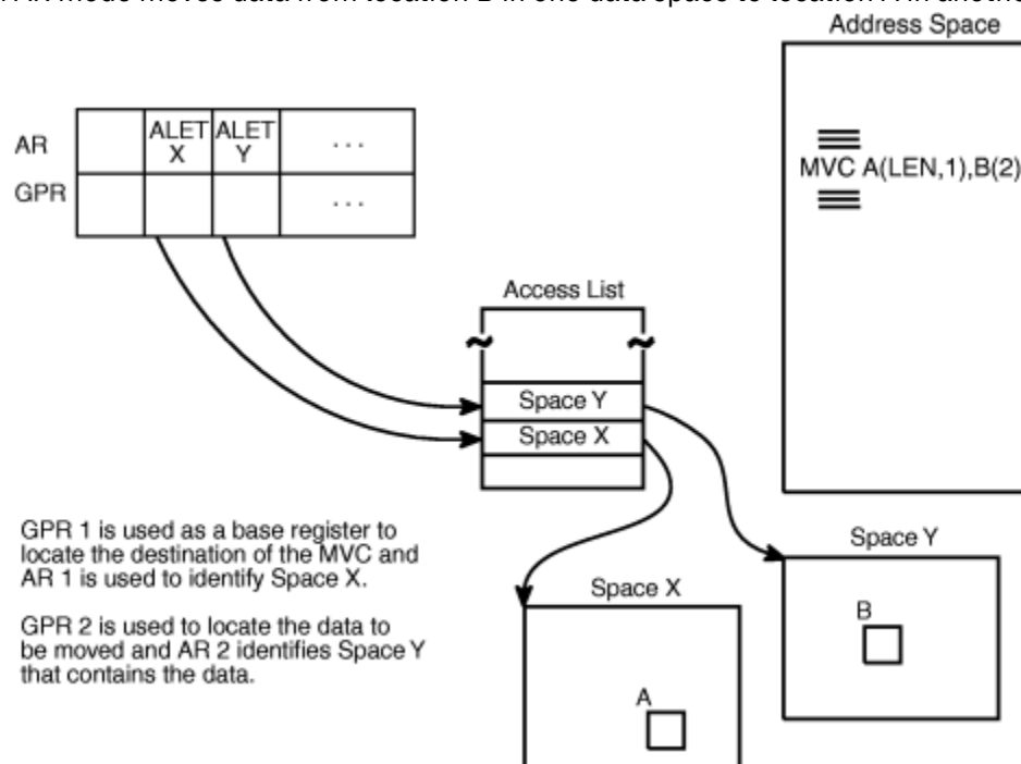
Figure 67. Using Instructions in AR Mode
