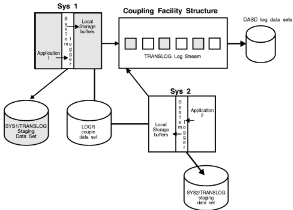
Figure 113. A Complete Coupling Facility Log Stream Configuration
