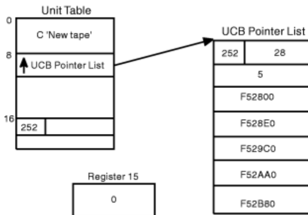
Figure 140. Output from Function Codes 3 and 10
