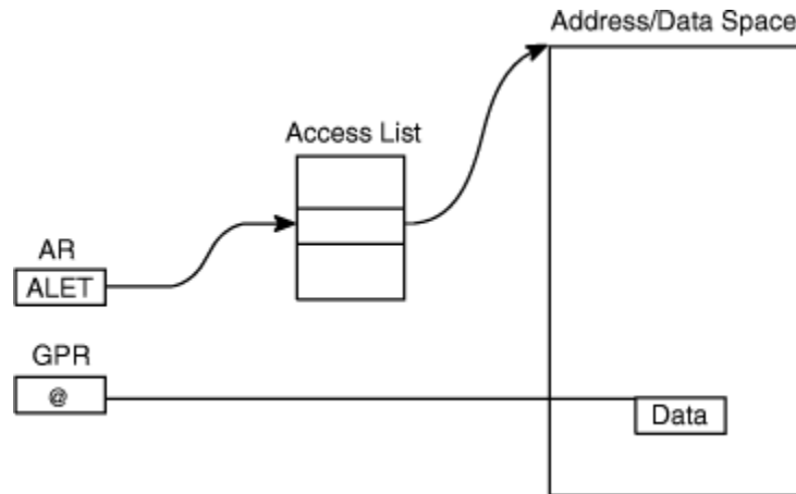
Figure 65. Using an ALET to Identify an Address Space or a Data Space
