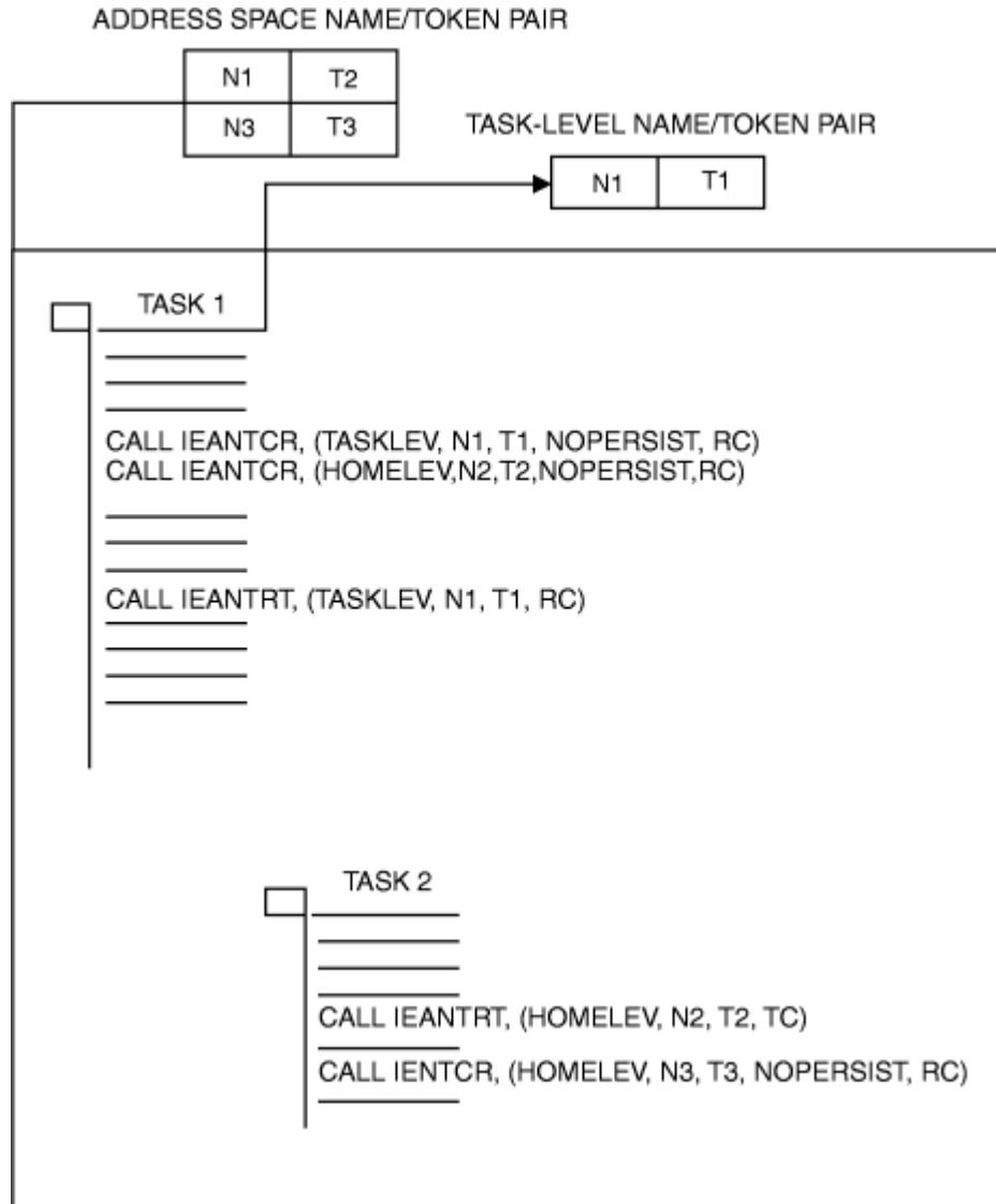
Figure 87. Using Home-Level and Task-Level Name/Token Pairs
