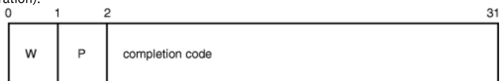
Figure 44. Event Control Block (ECB)
