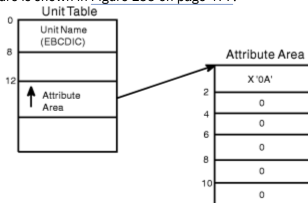
Figure 133. Requesting function code 8 (return attributes)
