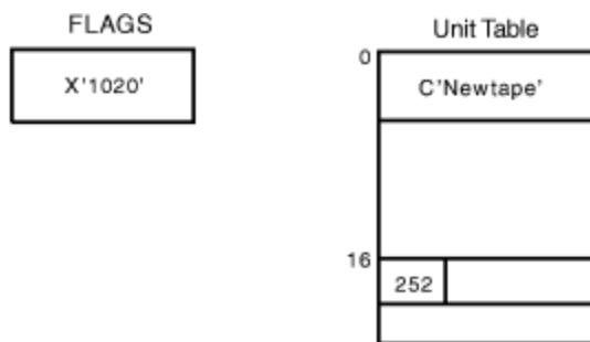
Figure 139. Input for Function Codes 3 and 10
