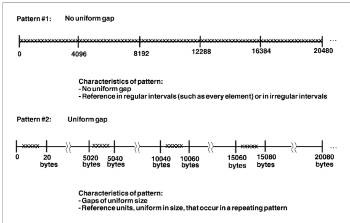
Figure 93. Two Typical Reference Patterns
