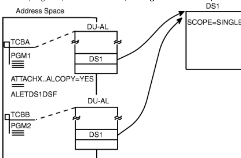
Figure 73. Two Problem Programs Sharing a SCOPE=SINGLE Data Space
