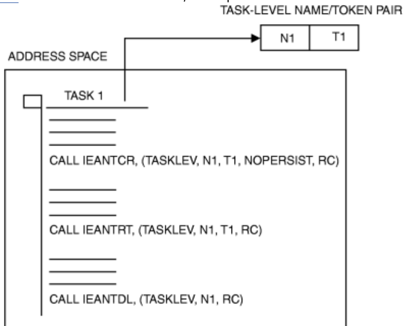
Figure 86. Using the Task Level in a Single Address Space
