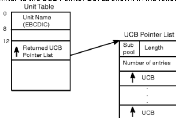
Figure 125. Output from Function Code 3 (Return UCB Addresses)
