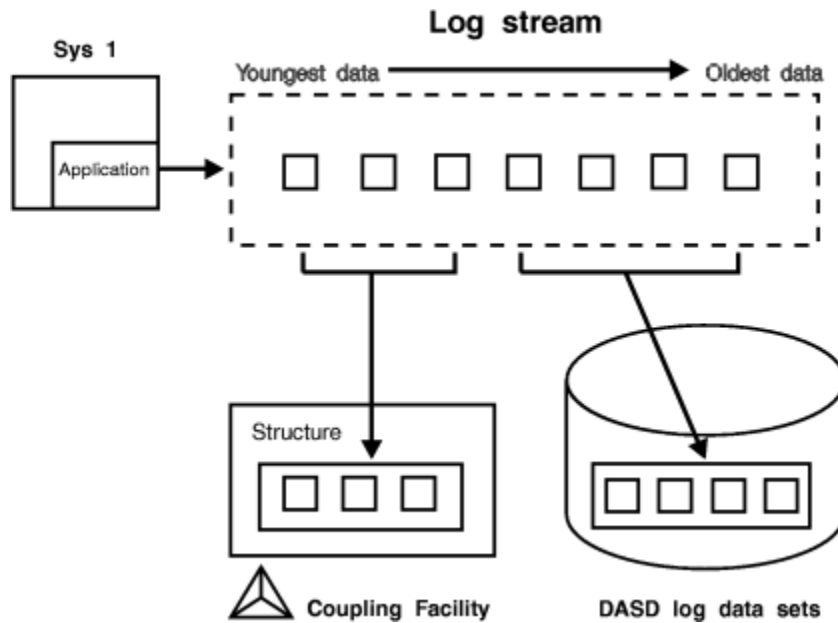
Figure 111. Log Stream Data on the Coupling Facility and DASD
