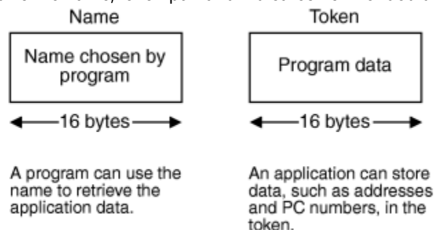
Figure 85. Using the Name and the Token
