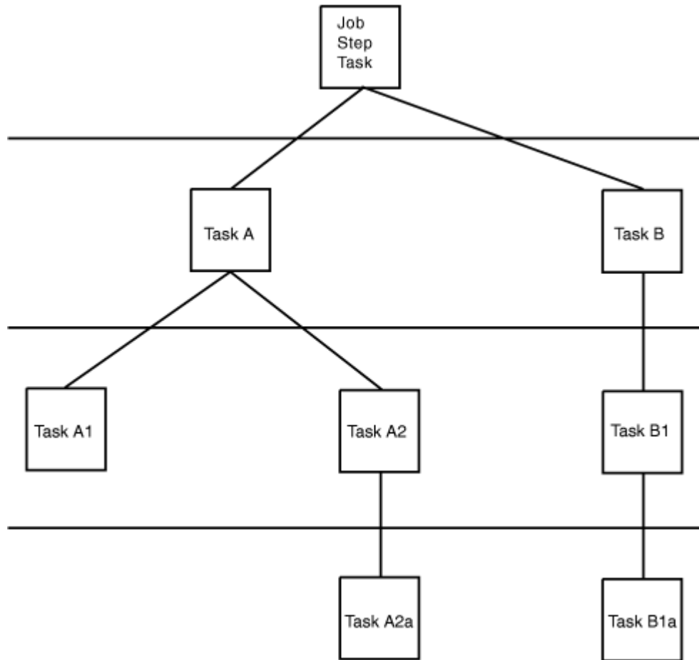
Figure 8. Levels of Tasks in a Job Step
