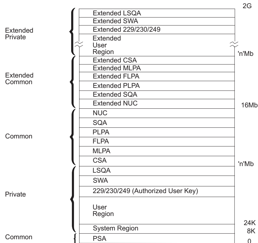
Figure 3. Virtual storage layout for single address space
