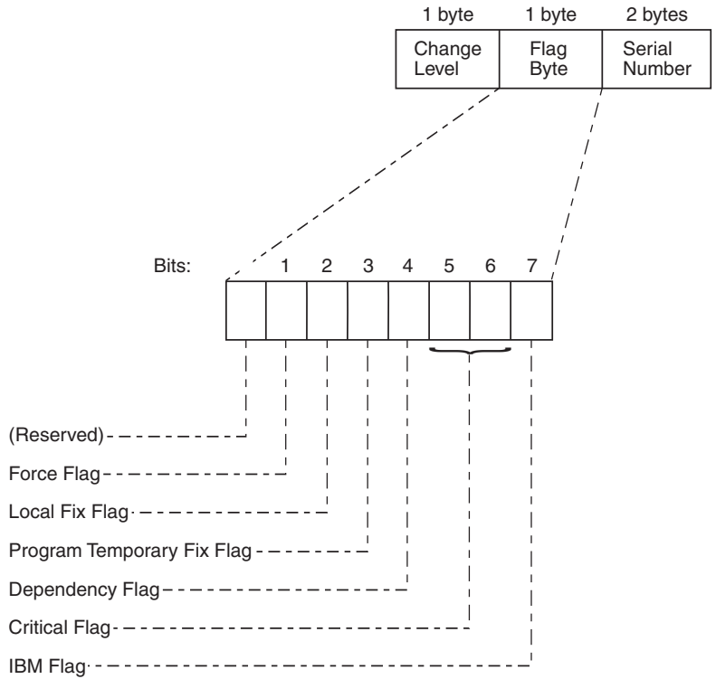
Figure 198. Flag bytes in the System Status Index field
