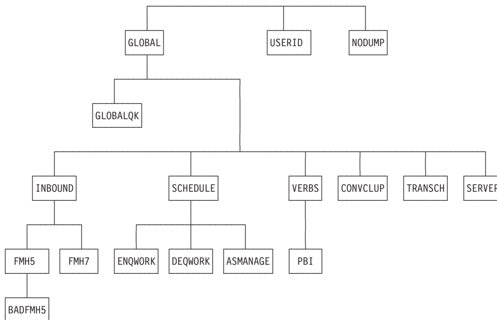
Figure 106. Hierarchy of SYSAPPC Component Trace Options. Hierarchy of SYSAPPC Component Trace Options
