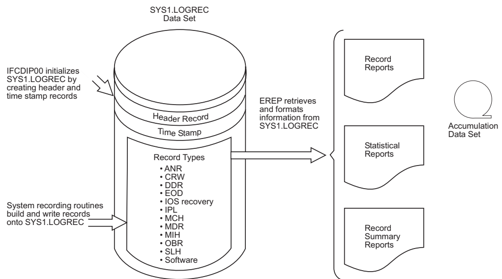
Figure 162. Logrec Error Recording Overview
