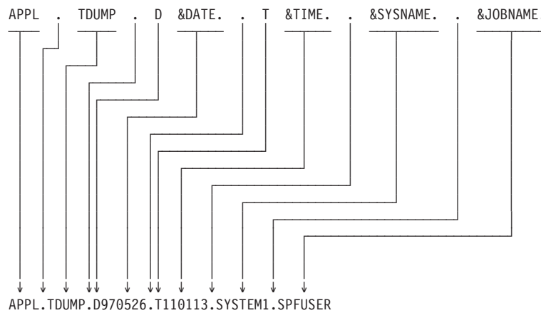
Figure 22. SPFUSER name pattern for automatically allocated dump data set
