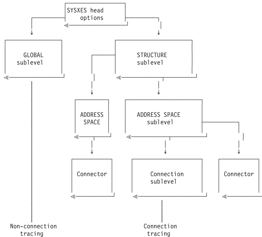
Figure 154. SYSXES SUB Trace Structure
