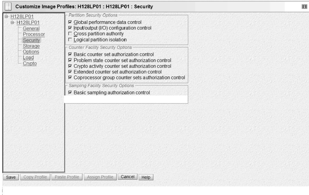
Figure 228. Activation profile security panel for new LPAR
