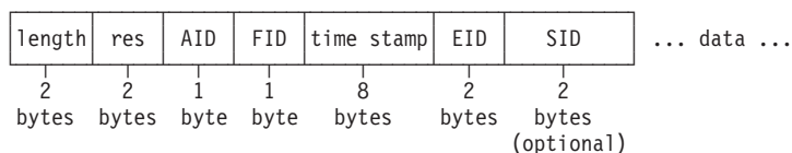
Figure 102. Header for Unformatted System trace record Format
