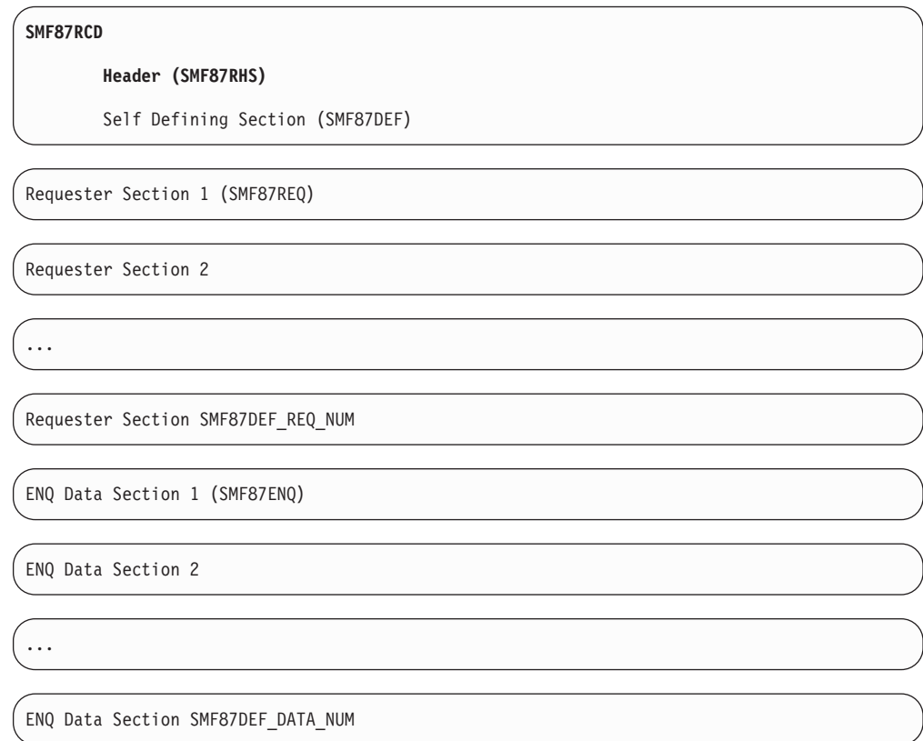
Figure 80. Record structure for SMF 87 subtype 2
