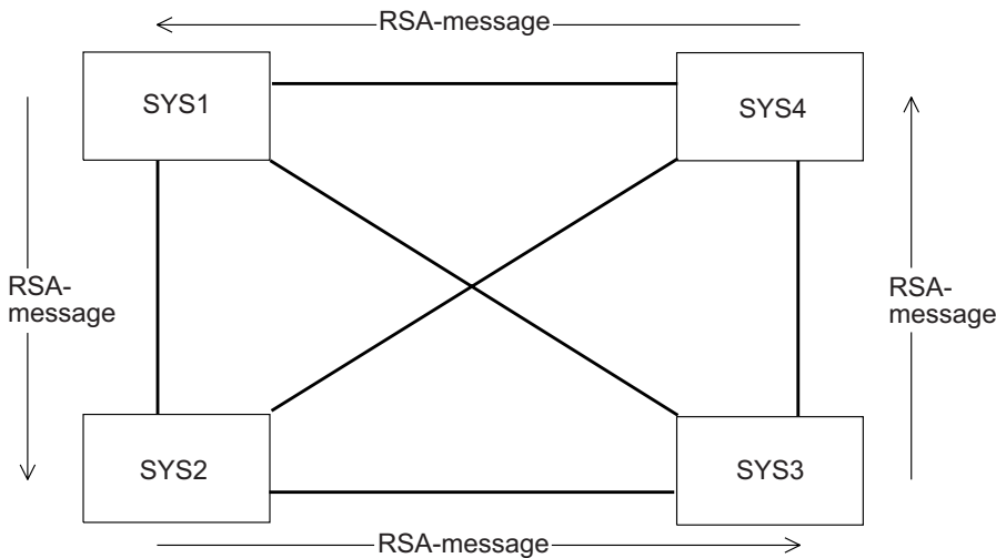
Figure 65. Ring Acceleration Configuration
