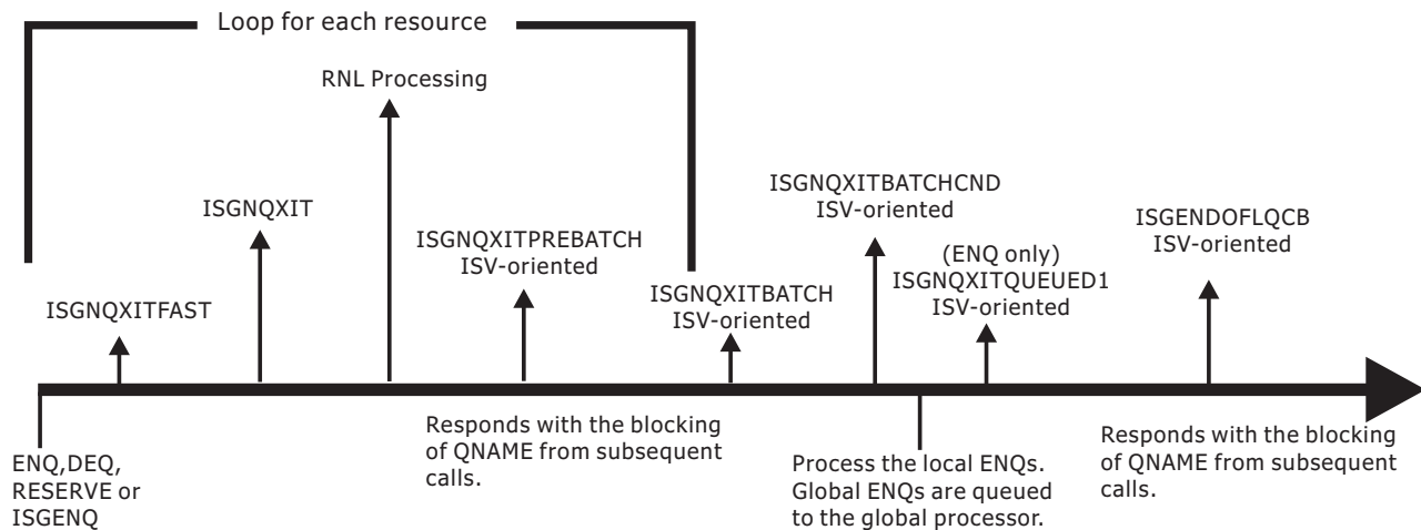
Figure 4. ENQ/DEQ exits installation flow
