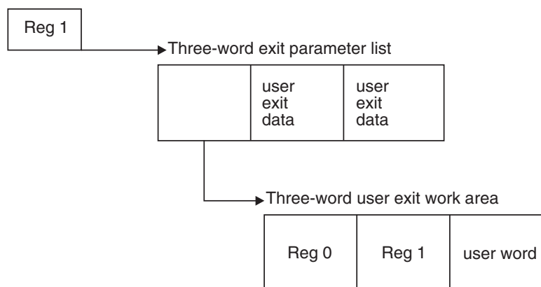
Figure 27. SMF Dump Program Input Parameter Structure
