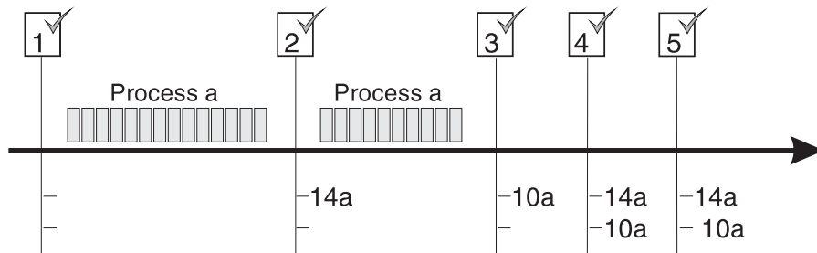
Figure 37. SMF record type 30: Example 2
