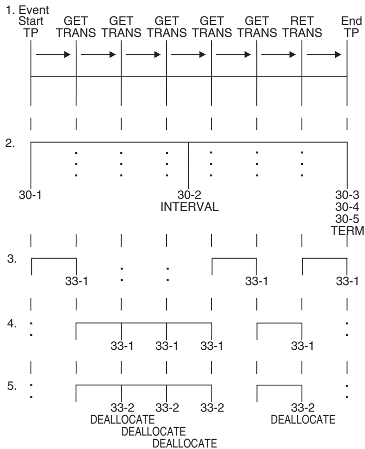
Figure 33. Example of multi-trans shell processing
