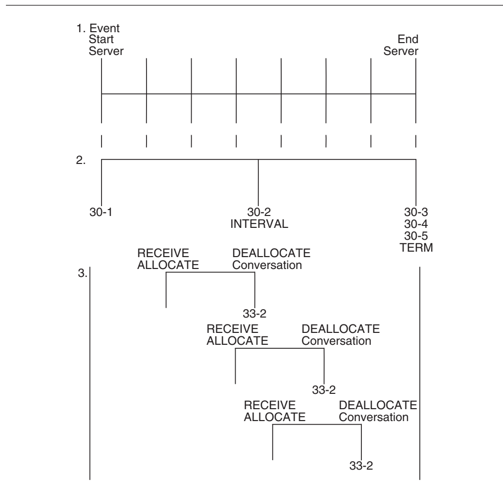
Figure 34. Example of APPC/MVS server processing
