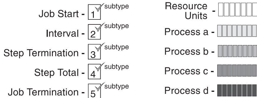
Figure 35. SMF job flow examples - key
