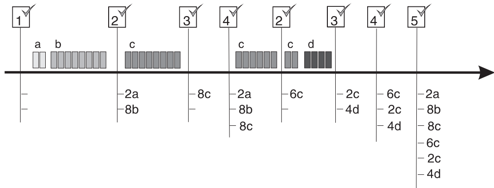
Figure 39. SMF record type 30: Example 4
