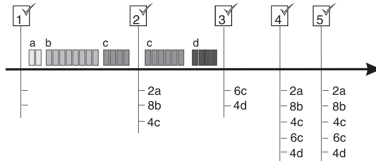
Figure 38. SMF record type 30: Example 3
