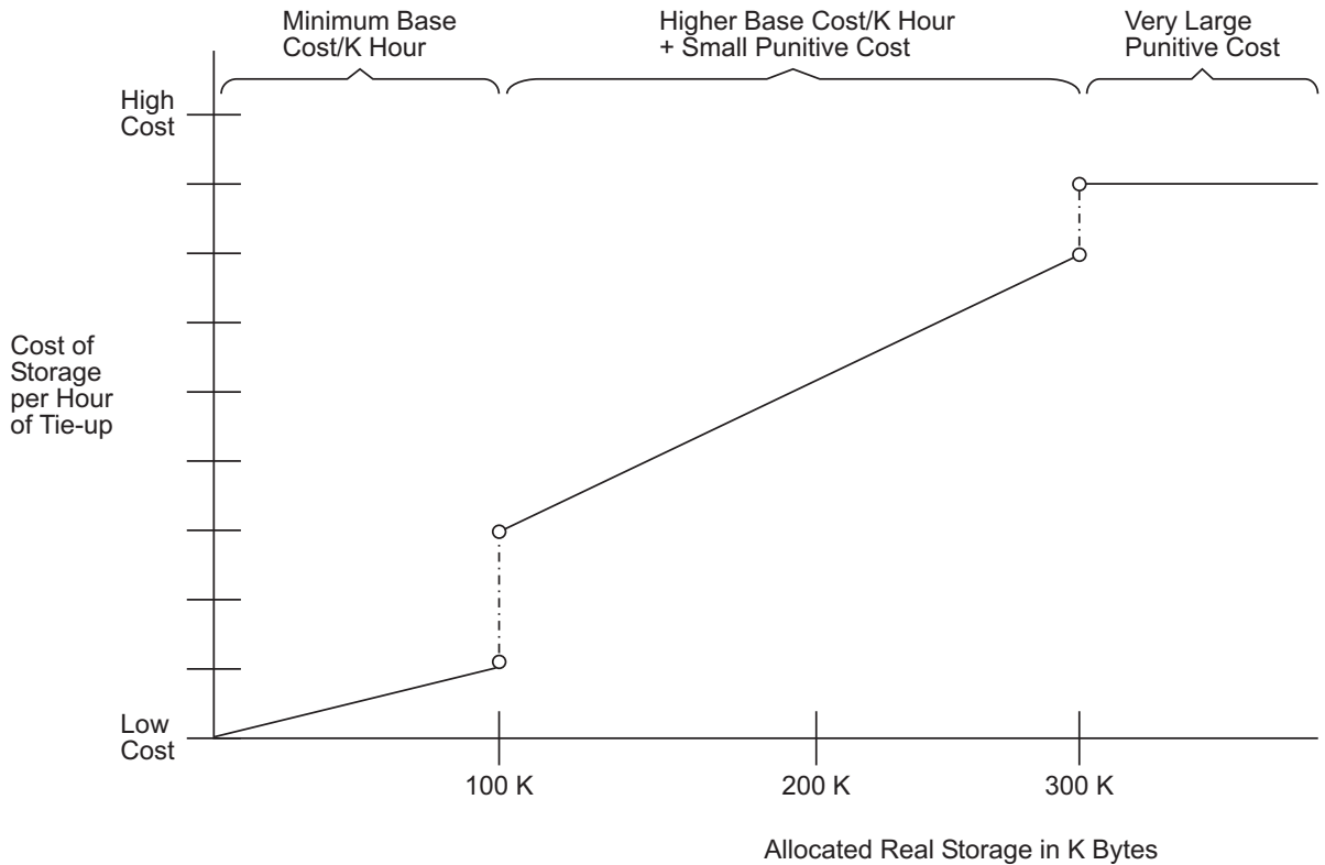
Figure 2. Sample degradation billing for ADDRSPC=REAL storage
