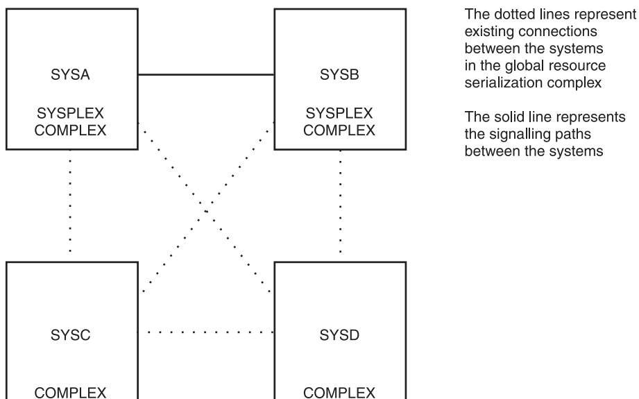
Figure 78. On PR/SM - Physical Configuration of a Sysplex on LPARs
