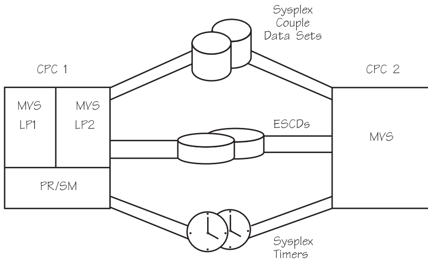
Figure 79. Configuration of a Sysplex on LPAR and Non-LPAR Systems
