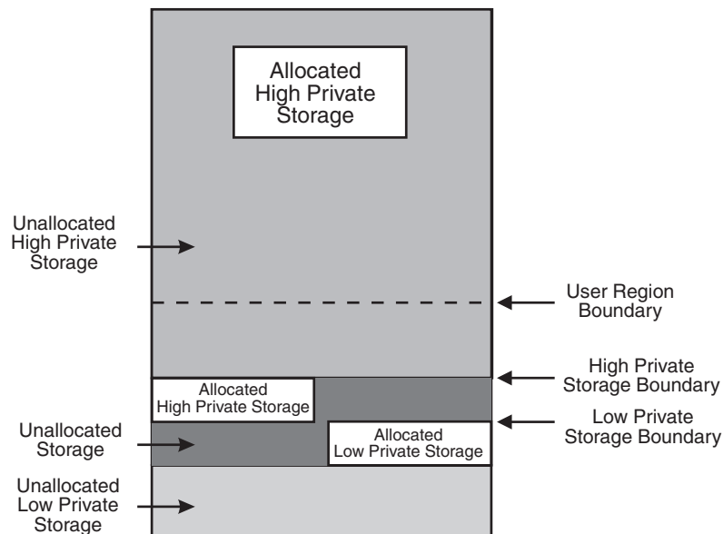
Figure 35. Low and High Private Storage Allocation
