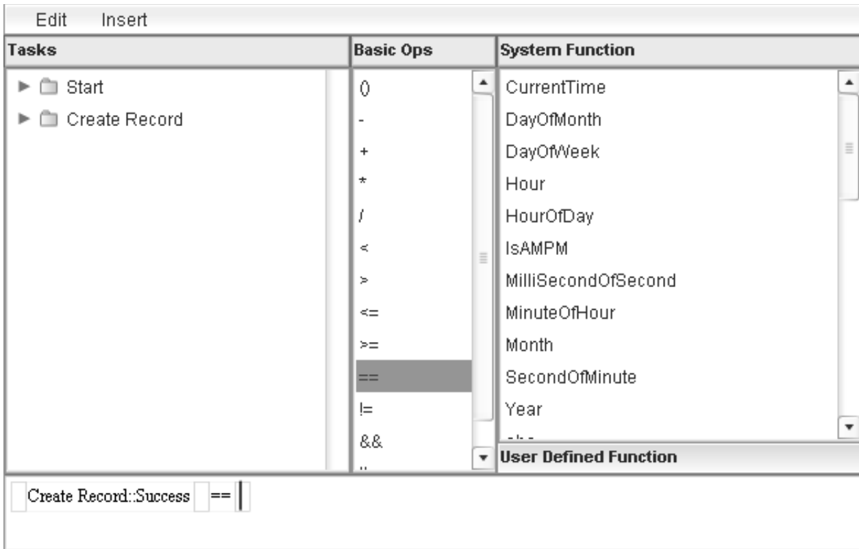
Figure 77. Condition Builder ==
