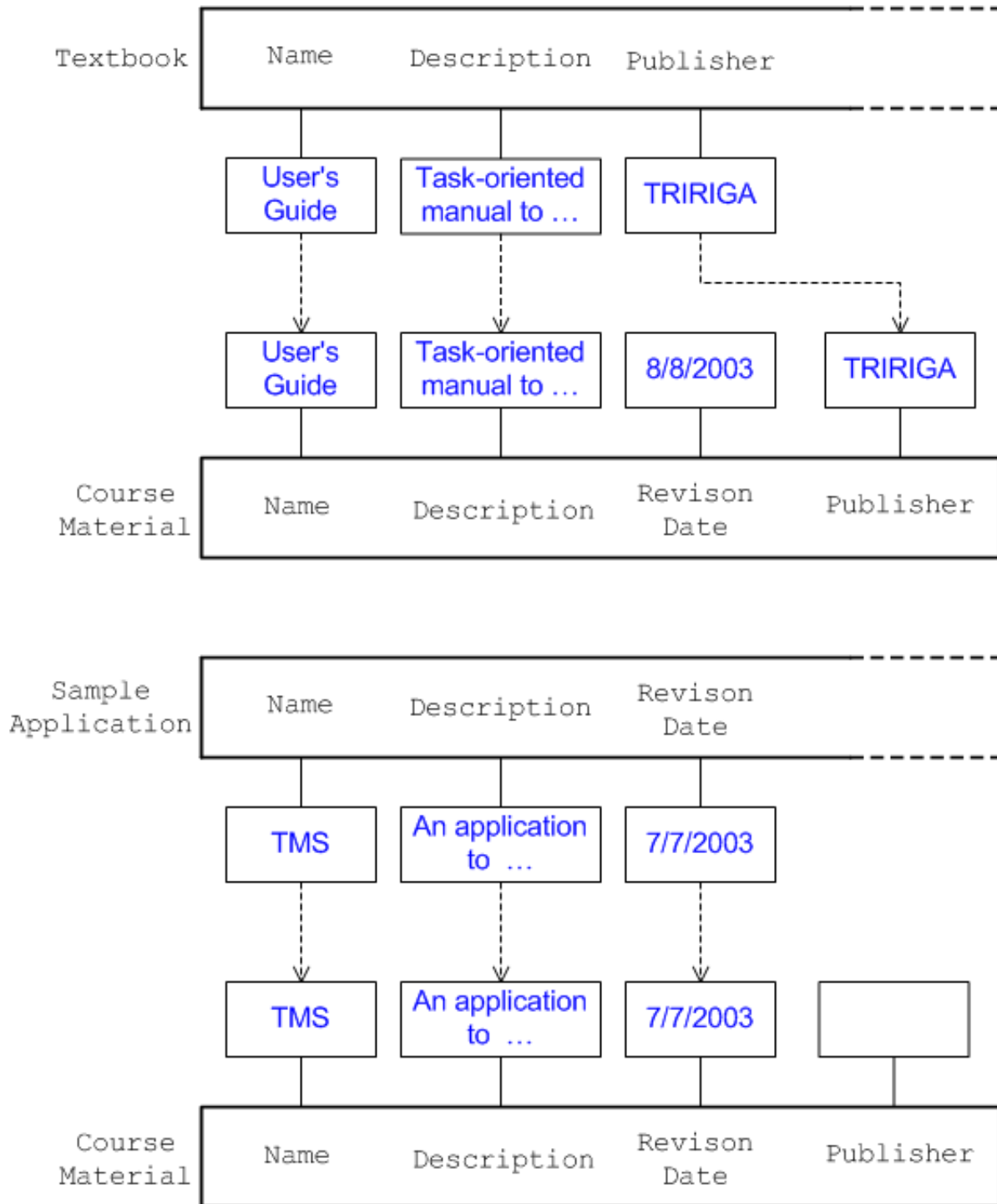
Figure 16. Links
