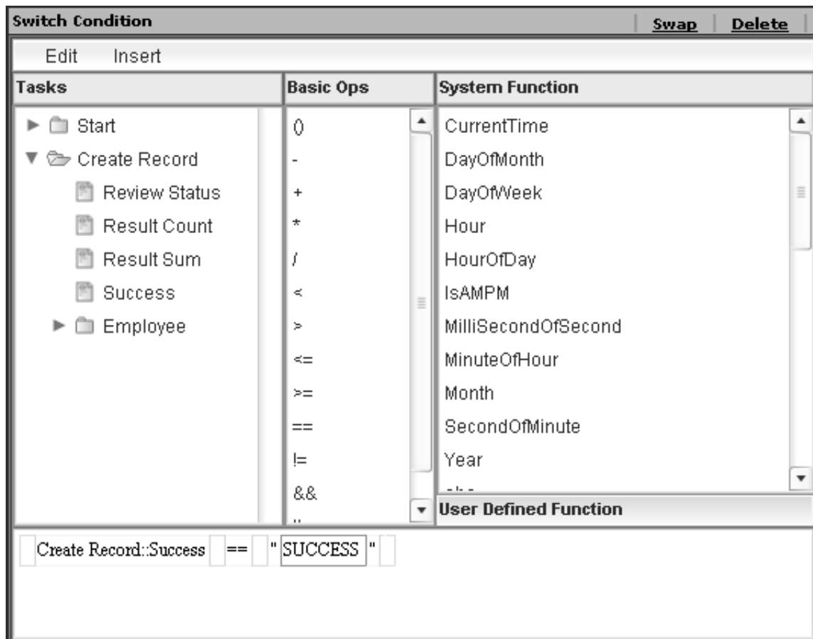
Figure 74. Switch properties
