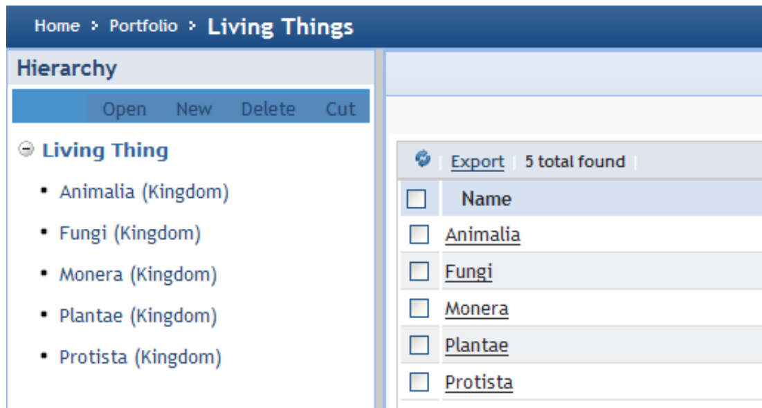
Figure 118. Kingdoms added
