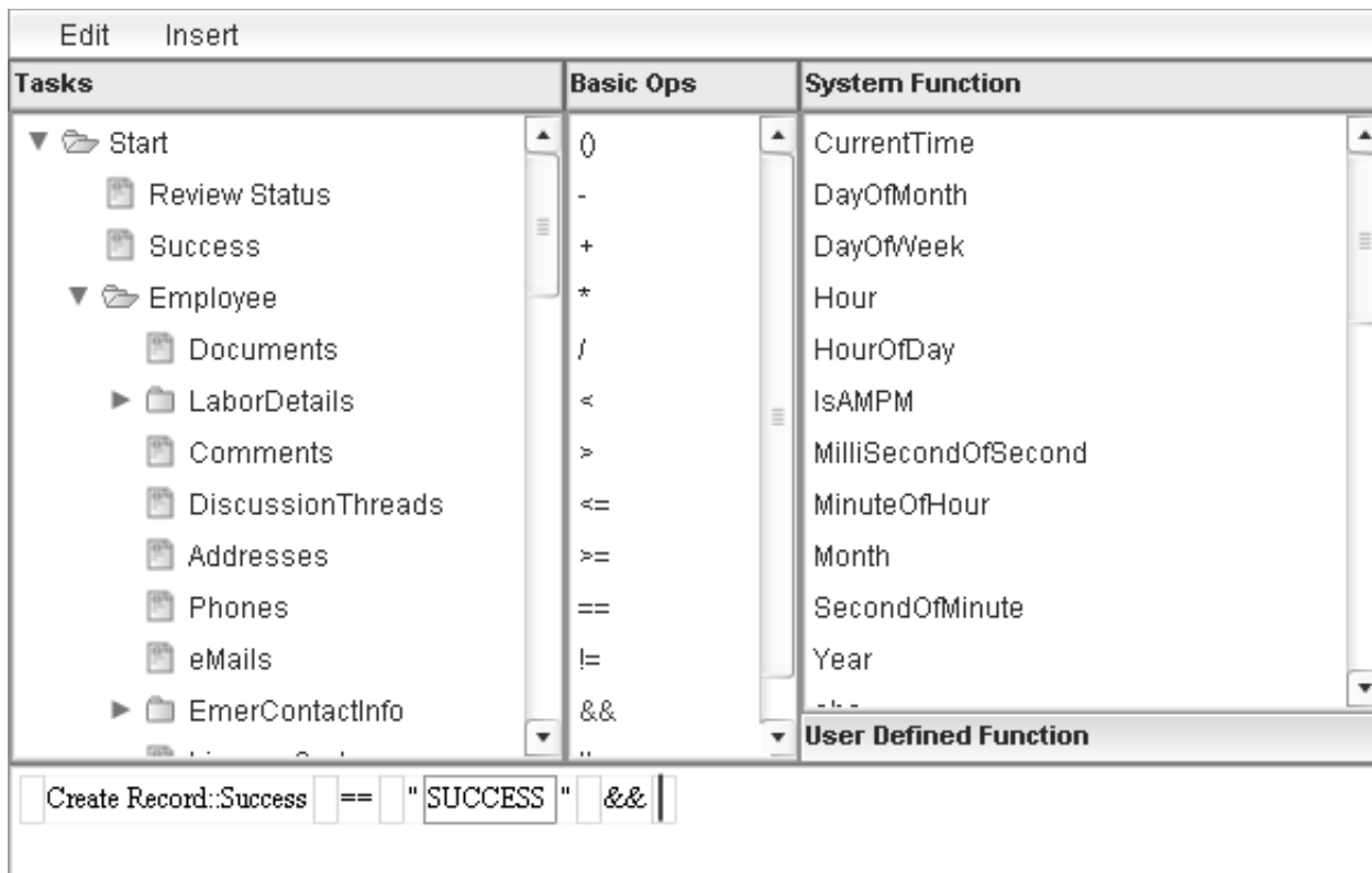
Figure 80. Condition Builder &&
