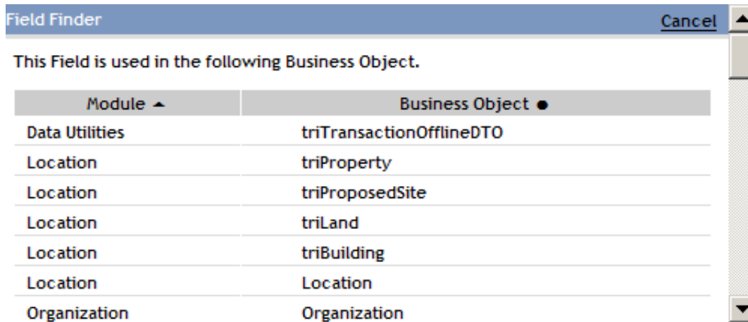
Figure 5. Field finder
