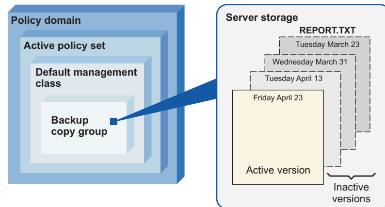
Figure 71. Active and inactive versions of REPORT.TXT
