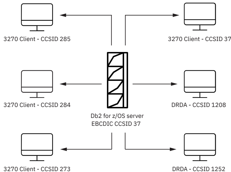
Figure 1. Example of setting CCSIDs in a distributed environment
