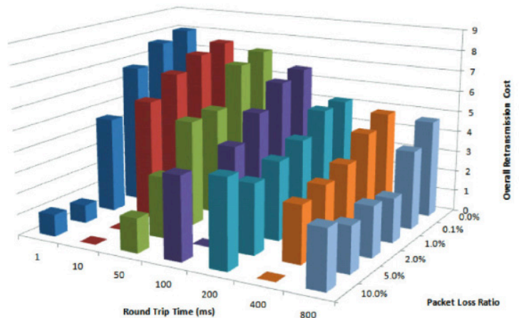
Figure 1: Shows the overall cost of transmitting one packet by a single UDT transfer on a T3 (45 Mbps) link under different RTTs and packet loss ratios. For most typical wide area networks, one packet transfer needs eight to ten retransmissions!
