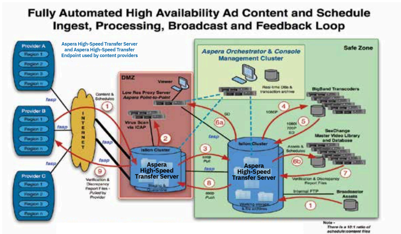
Figure 7: Simplified workflow representations under Aspera Orchestrator control
