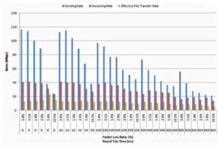
Figure 3: Difference in transmission rate, receiving rate, and effective file transfer rates for UDT on WANs.
