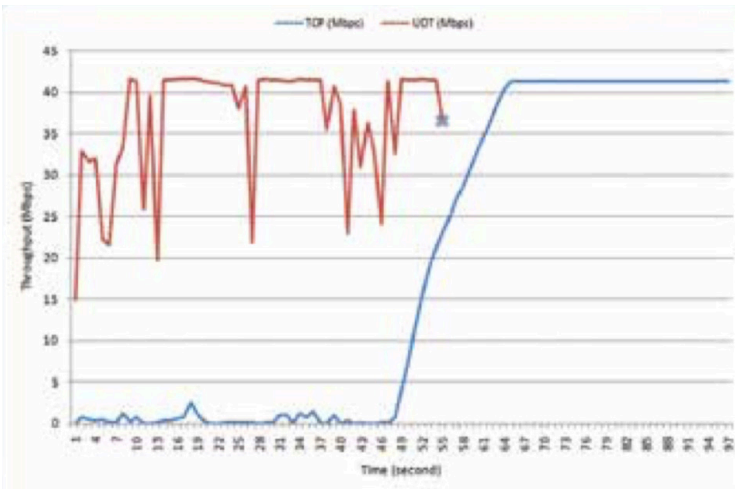
Figure 2: Shows the denial of service caused to a standard TCP flow due to the lack of proper congestion control in UDT.
