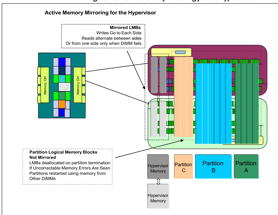
Figure 23: Active Memory Mirroring for the Hypervisor
